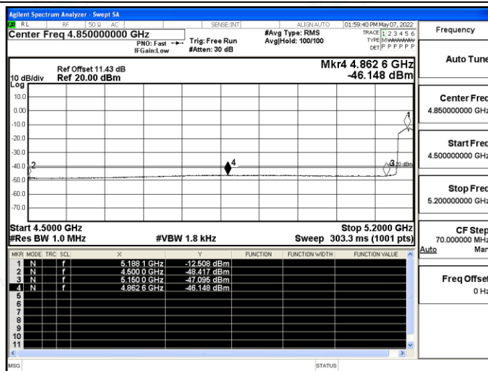
11AX40SISO_Ant A_Low_5190_Peak
