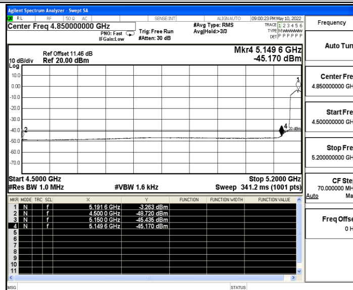
11AC40SISO_Ant B_Low_5190_Peak
