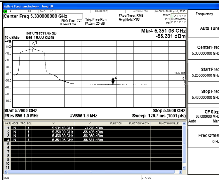
11AX40SISO_Ant B_High_5230_Peak
