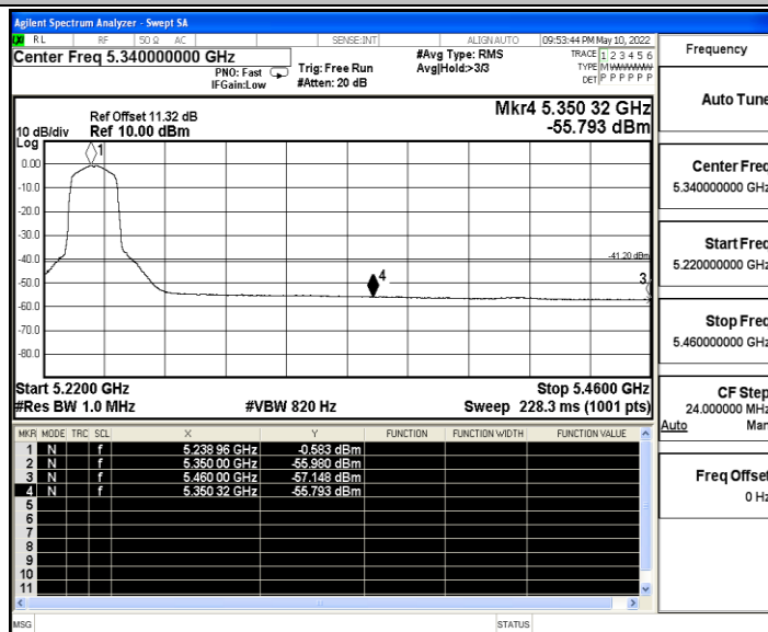
11AX20SISO_Ant B_High_5240_Peak
