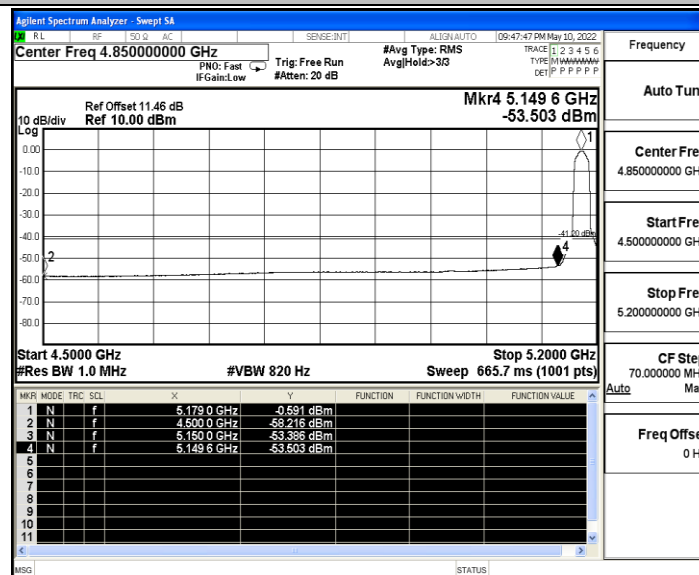
11AX20SISO_Ant B_Low_5180_Peak
