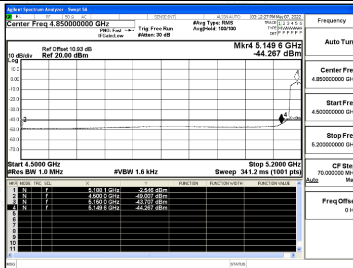
11AC40SISO_Ant A_Low_5190_Peak
