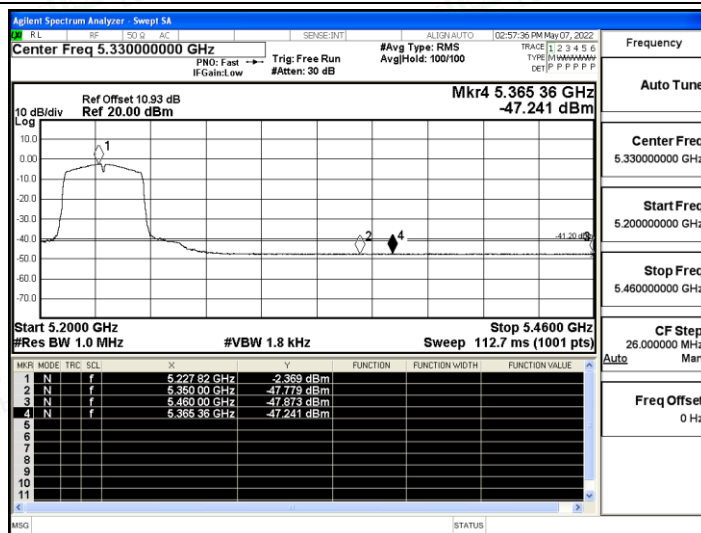
11N40SISO_Ant A_High_5230_Peak
