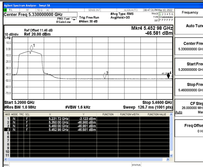
11N40SISO_Ant B_High_5230_Peak
