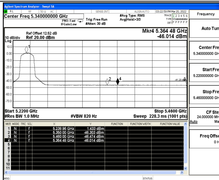
11AC20SISO_MIMO_High_5240_Peak
