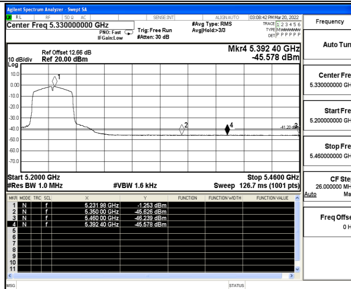
11N40SISO_MIMO_High_5230_Peak
