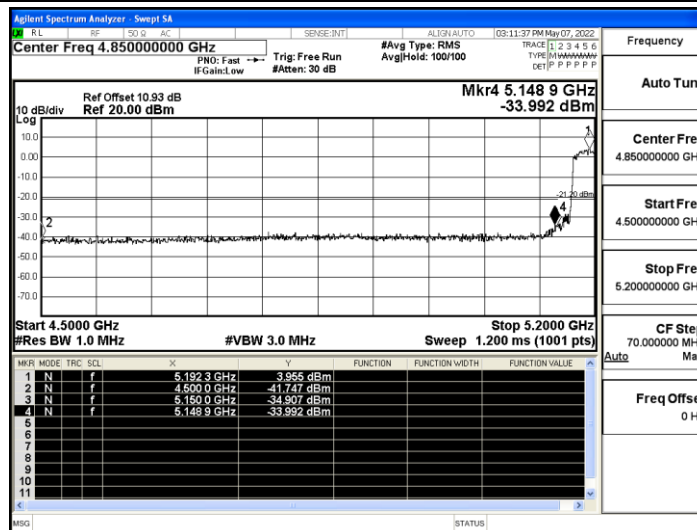
11AC40SISO_Ant A_High_5230_AV
