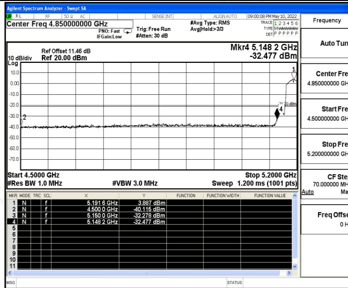
11AC40SISO_Ant B_High_5230_AV
