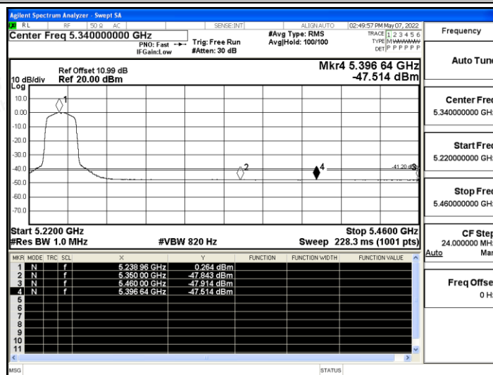
11N20SISO_Ant A_High_5240_Peak
