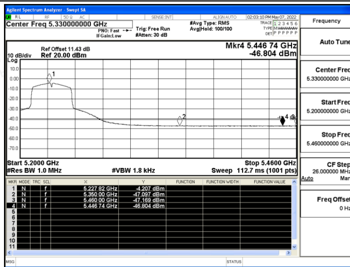
11AX40SISO_Ant A_High_5230_Peak
