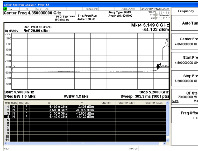
11N40SISO_Ant A_Low_5190_Peak
