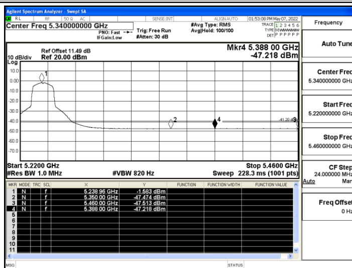
11AX20SISO_MIMO_High_5240_Peak
