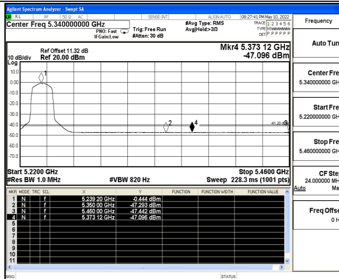
11A_Ant B_High_5240_Peak
