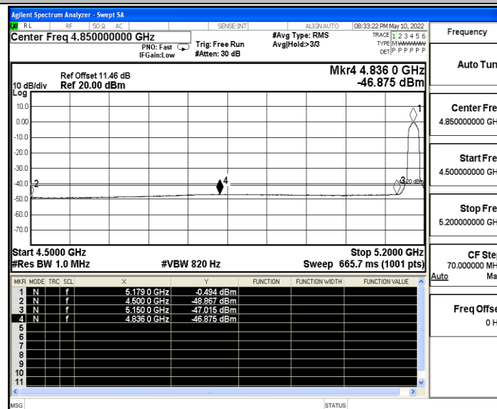
11N20SISO_Ant B_Low_5180_Peak
