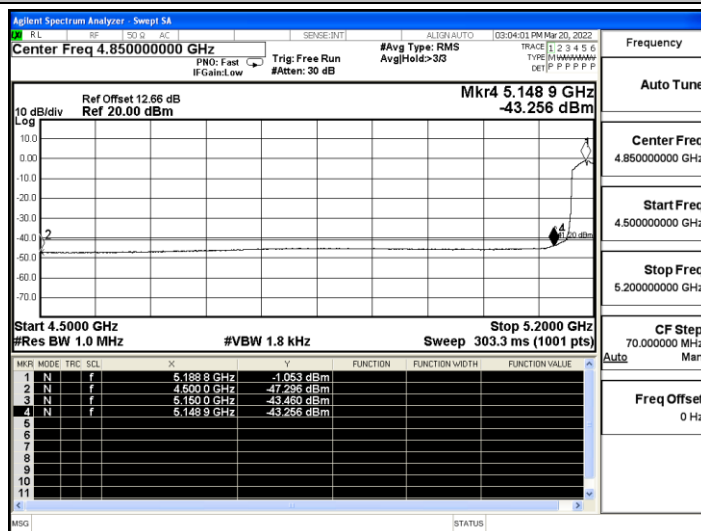
11N40SISO_MIMO_Low_5190_Peak
