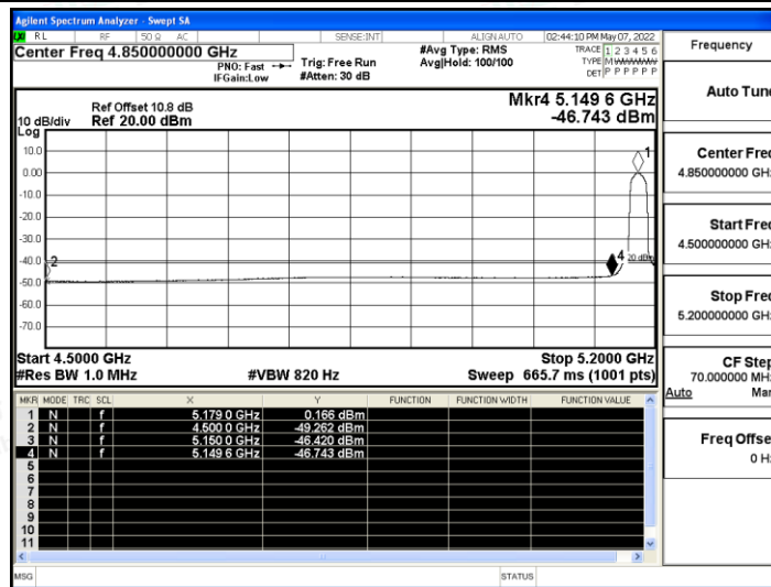
11N20SISO_Ant A_Low_5180_Peak
