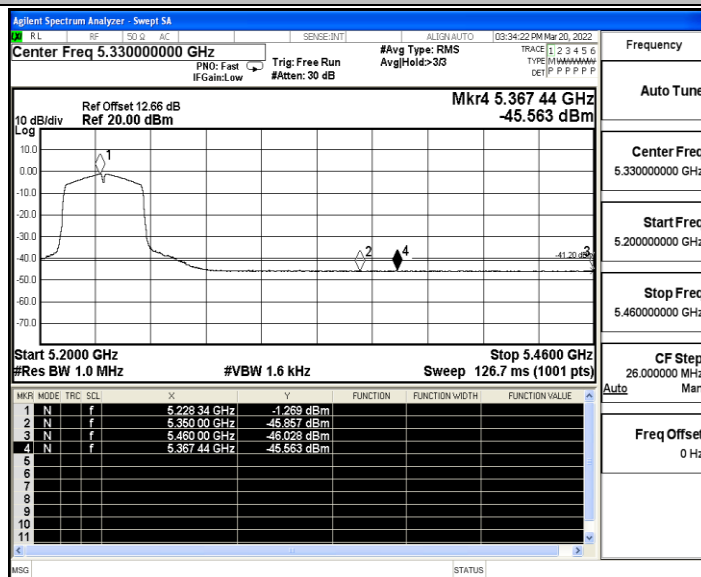
11AC40SISO_MIMO_High_5230_Peak
