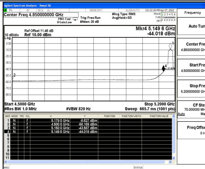
11AX20SISO_MIMO_Low_5180_Peak
