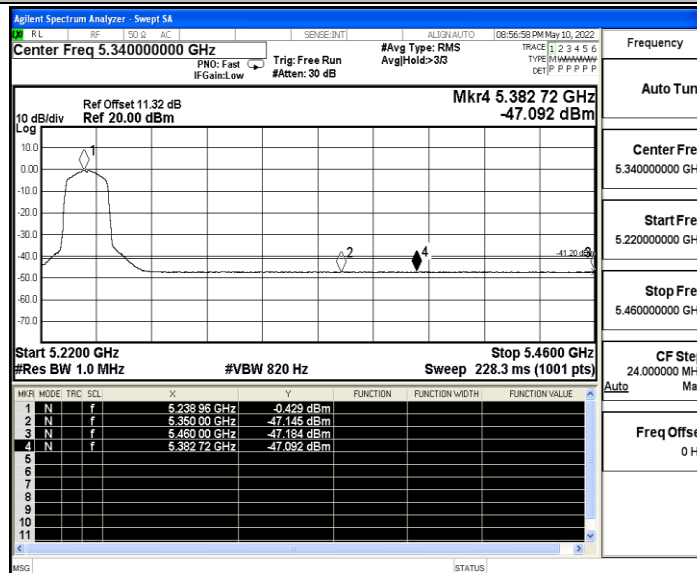
11AC20SISO_Ant B_High_5240_Peak
