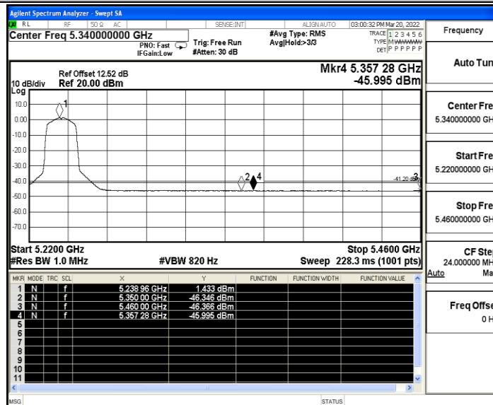
11N20SISO_MIMO_High_5240_Peak
