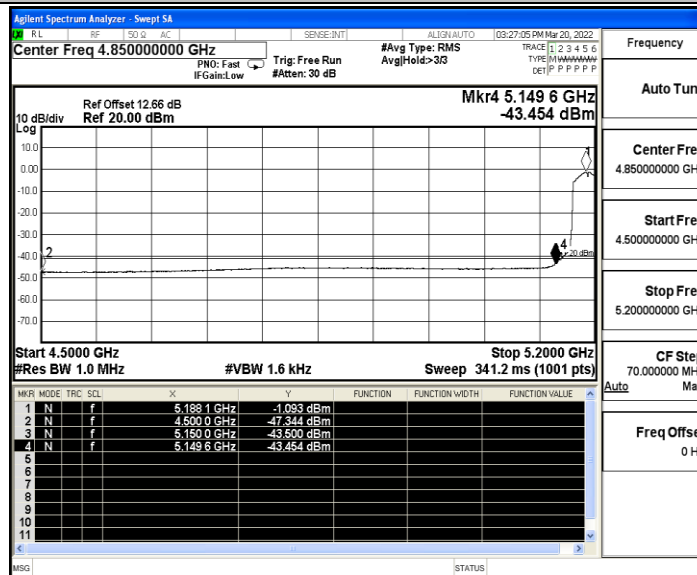
11AC40SISO_MIMO_Low_5190_Peak
