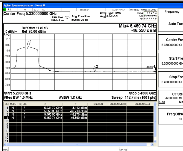
11AC40SISO_Ant B_High_5230_Peak
