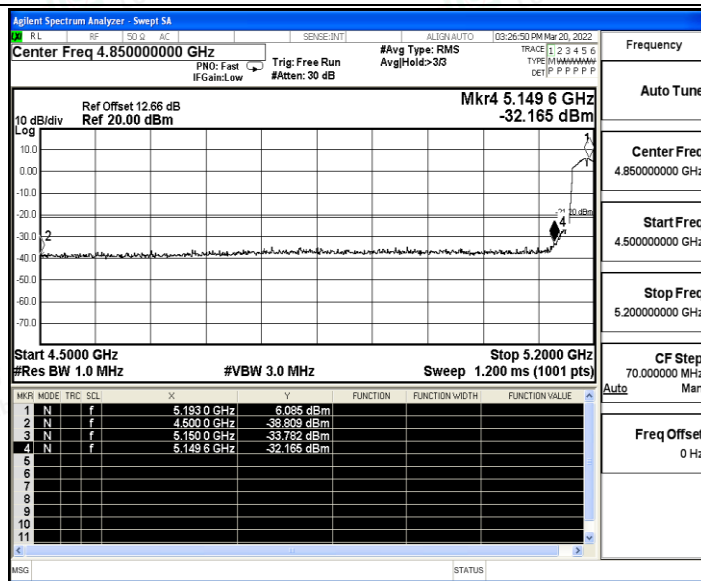
11AC40SISO_MIMO_High_5230_AV
