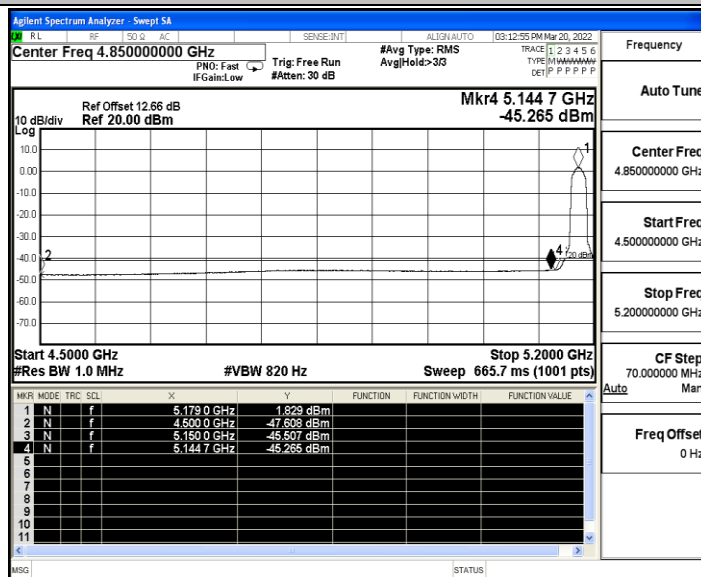
11AC20SISO_MIMO_Low_5180_Peak
