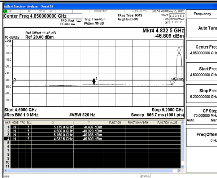
11AC20SISO_Ant B_Low_5180_Peak
