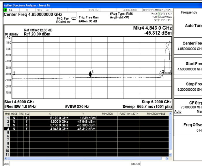
11N20SISO_MIMO_Low_5180_Peak
