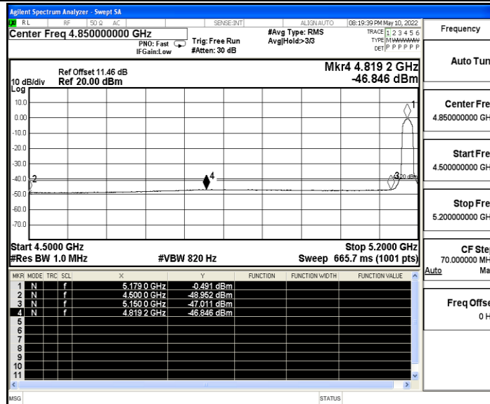
11A_Ant B_Low_5180_Peak
