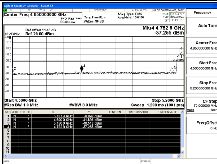
11AX40SISO_Ant A_High_5230_AV
