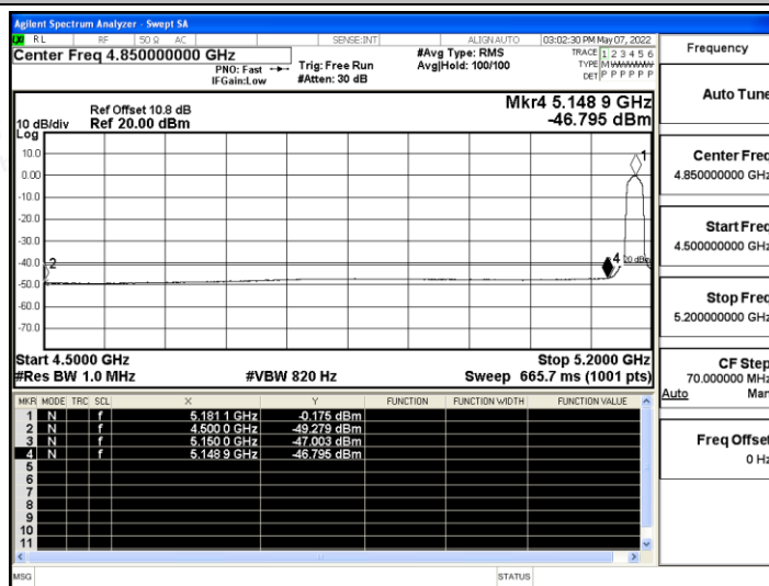
11AC20SISO_Ant A_Low_5180_Peak
