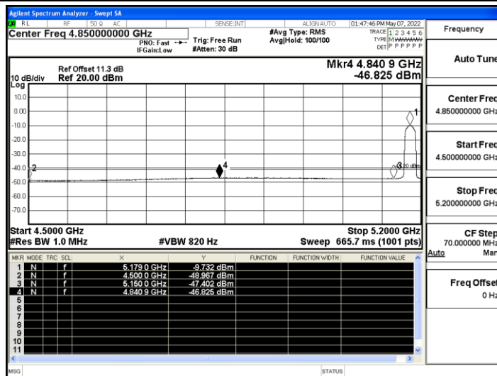
11AX20SISO_Ant A_Low_5180_Peak
