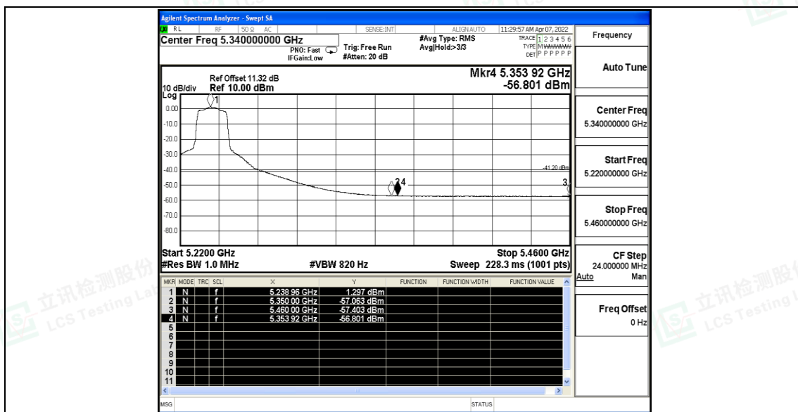
11AX20SISO_Ant A_High_5240_Peak
