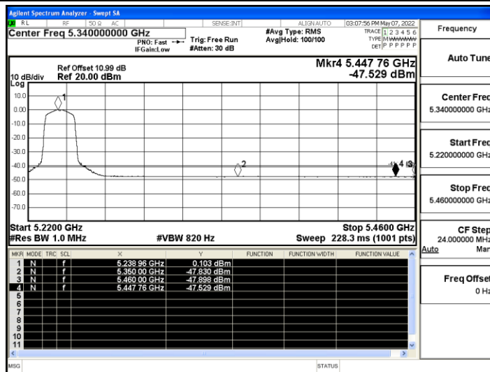
11AC20SISO_Ant A_High_5240_Peak
