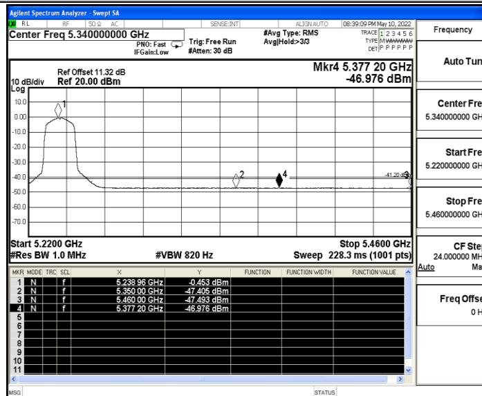
11N20SISO_Ant B_High_5240_Peak
