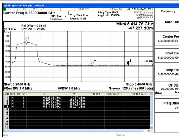
11AC40SISO_Ant A_High_5230_Peak
