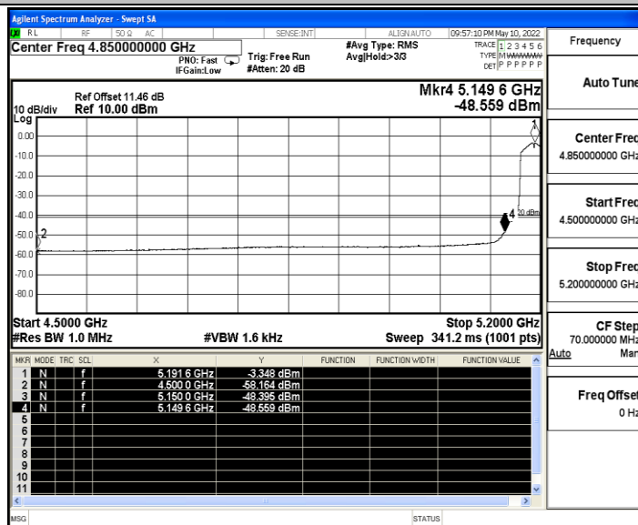
11AX40SISO_Ant B_Low_5190_Peak
