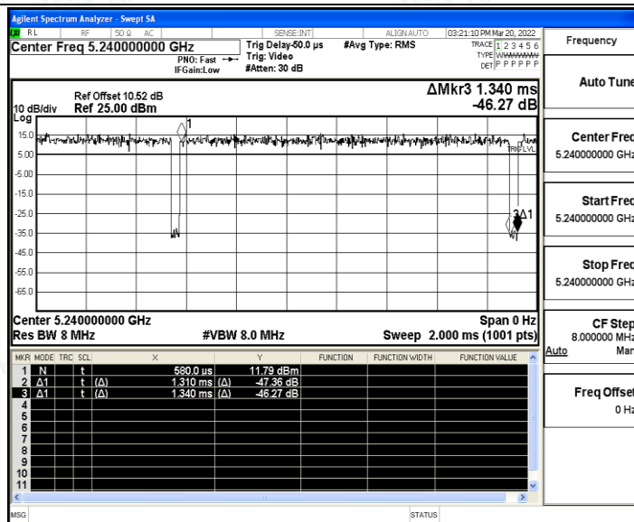
11AC40SISO_Ant A_5190
