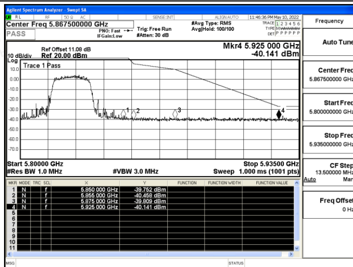
11N20SISO_Ant B_High_5825_Peak
