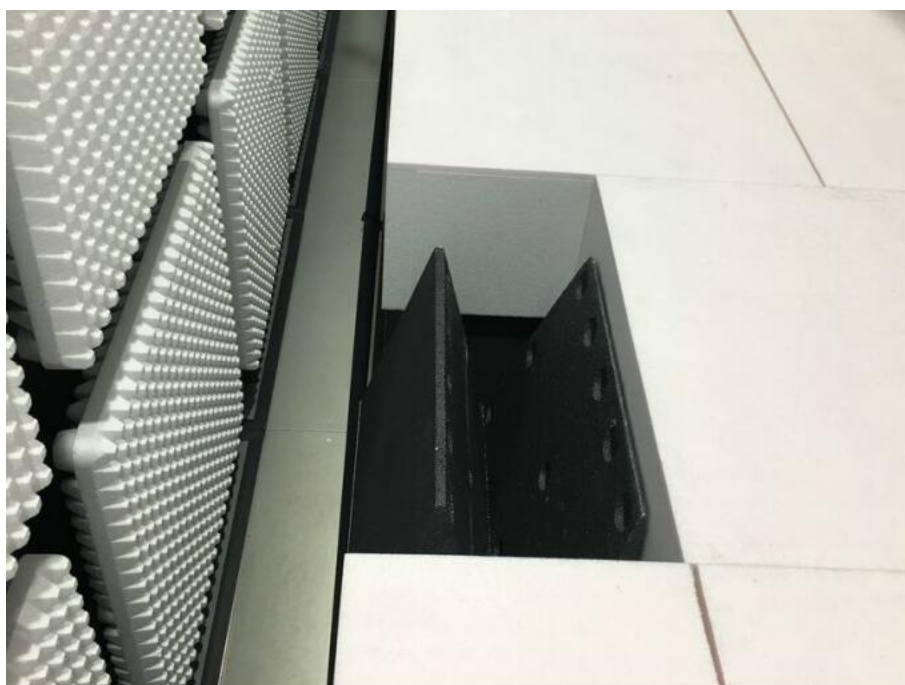
Radiated spurious emission Test Setup-6 There are absorbing materials under the ground.
