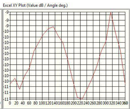
2.45GHz@Theta 0.0 Total
