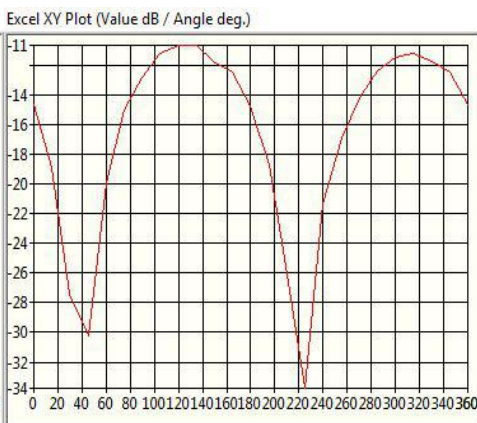
2.485GHz@Theta 0.0 Vertical
