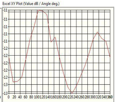
2.485GHz@Theta 0.0 Total
