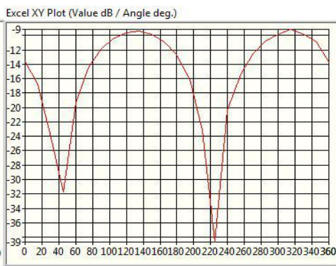
2.45GHz@Theta 0.0 Vertical
