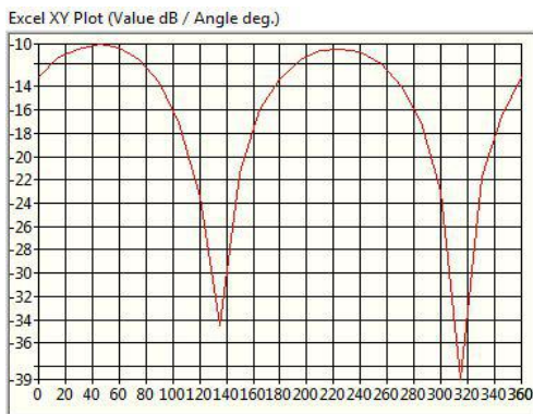
2.45GHz@Theta 0.0 Horizontal
