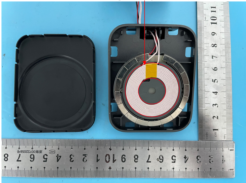
Antenna- for mobile phone charge ( \varnothing : 43mm)
