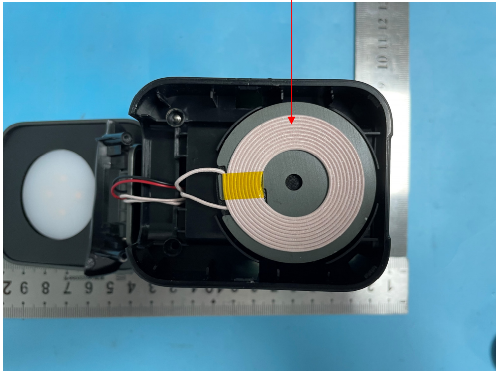
Antenna- for Airpod charge ( \varnothing : 50mm)
