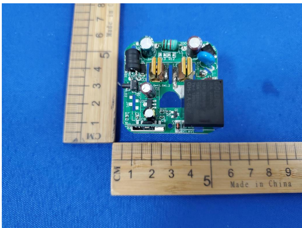
Figure 2. Internal view
