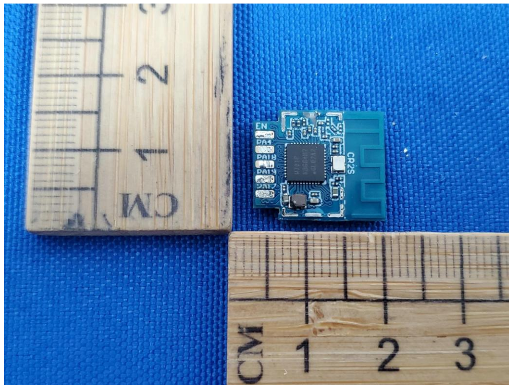
Figure 8. Internal view
