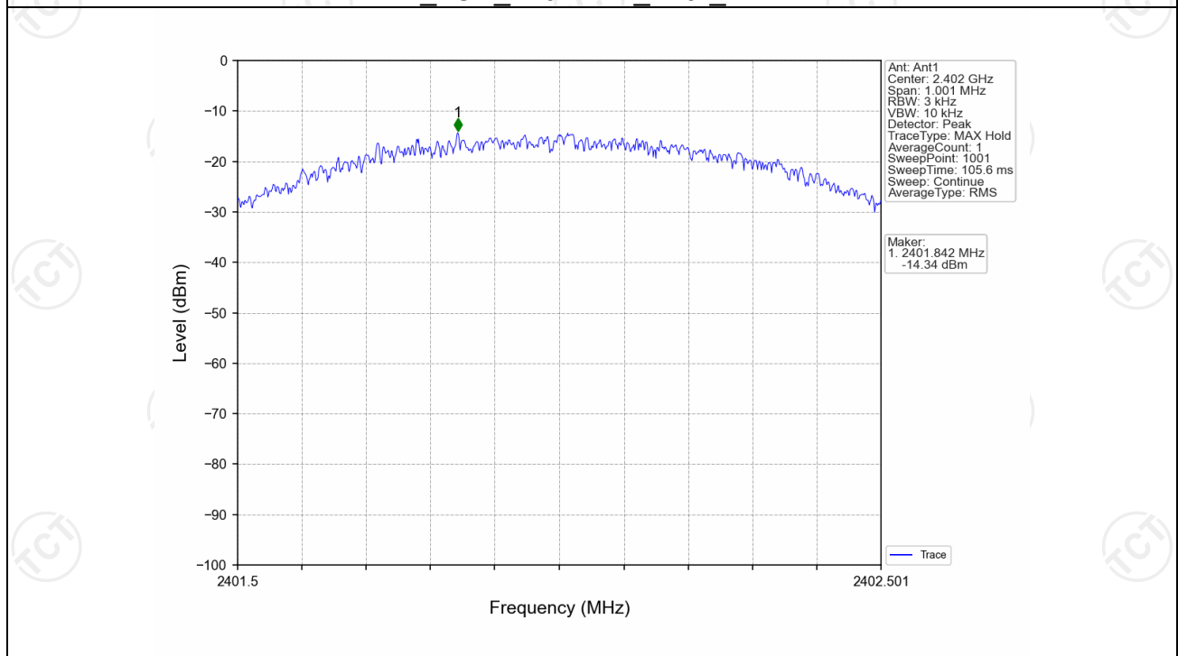
1M_LCH_2402MHz_Ant1_NTNV
