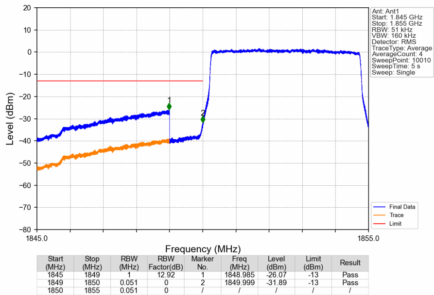
Band2_5MHz_16QAM_LCH_1852.5MHz_RB_25_0_NTNV
