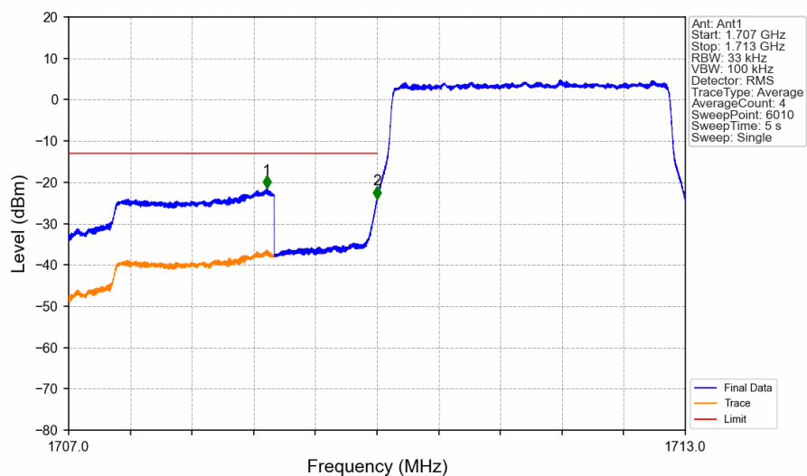
Band4_3MHz_QPSK_LCH_1711.5MHz_RB_15_0_NTNV
