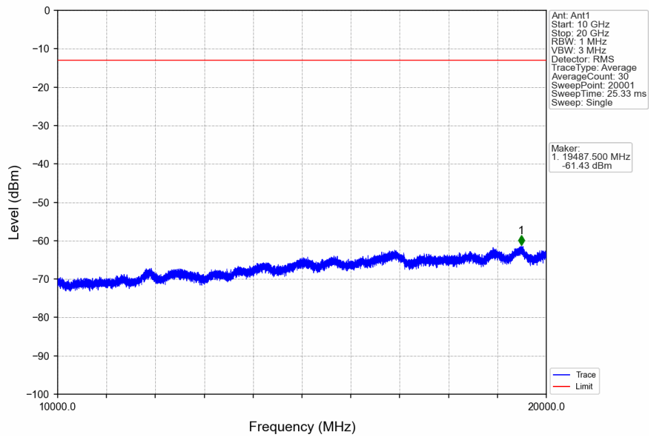
Band66_3MHz_QPSK_HCH_1778.5MHz_RB_1_0_NTV
