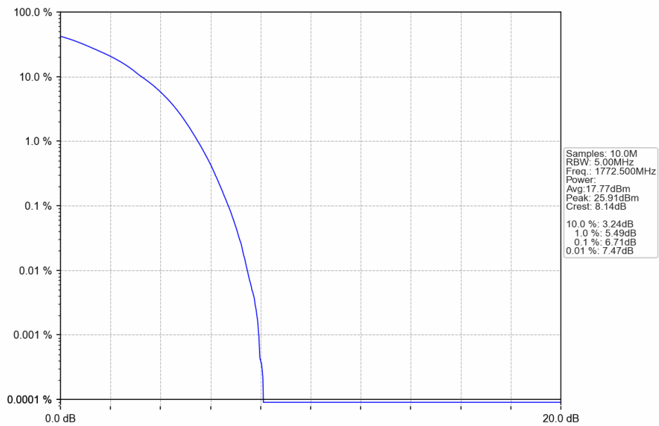
Band66_15MHz_16QAM_HCH_1772.5MHz_RB_75_0 NTN
