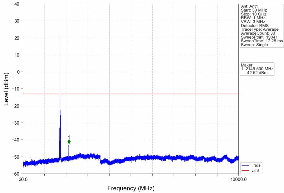
Band66_15MHz_16QAM_MCH_1745MHz_RB_1_0_NTV
