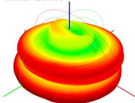
5150.0MHz H+V, Eff: 57.8%
