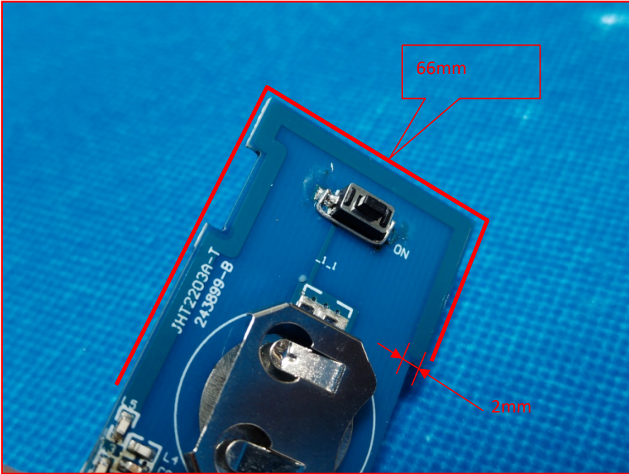
Dimension: 66mm*2mm
