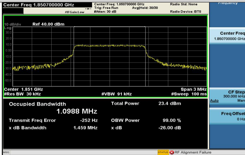
Band2-1.4MHz-16QAM-18607-6RB#0-1.0988
