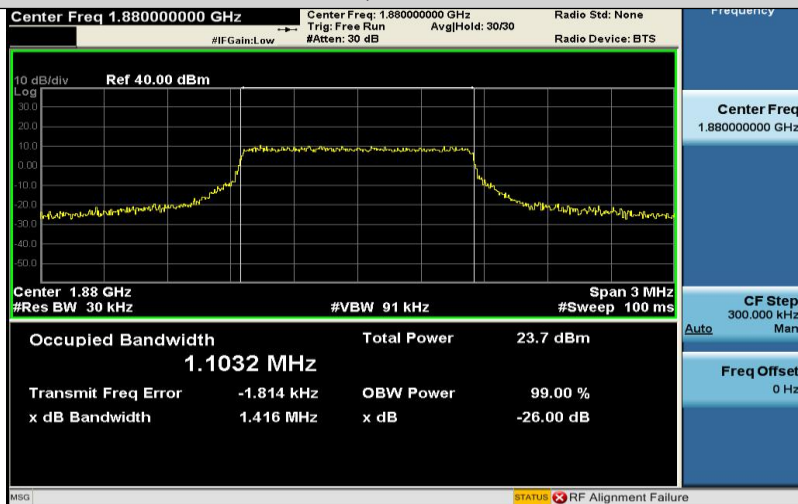
Band2-1.4MHz-16QAM-18900-6RB#0-1.1032
