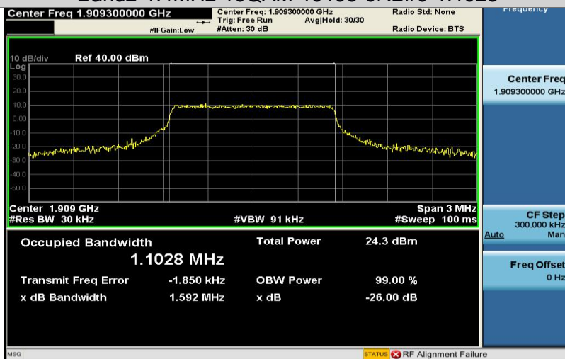
Band2-1.4MHz-16QAM-19193-6RB#0-1.1028
