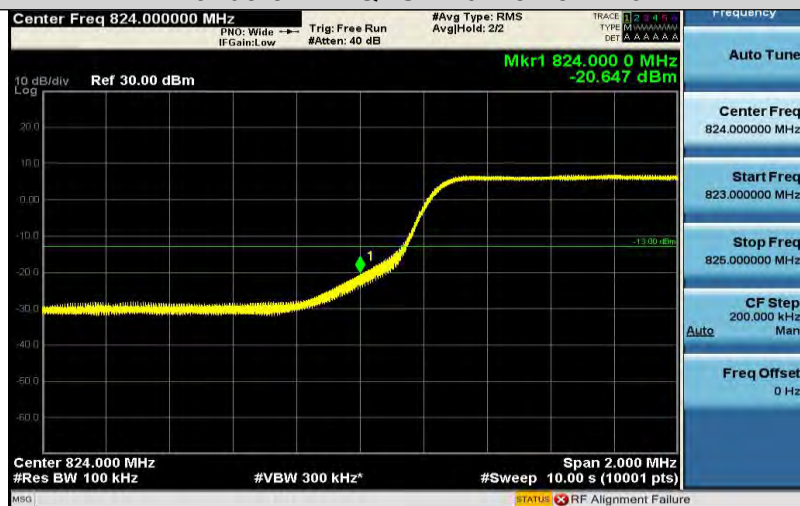
Band5-5MHz-QPSK-20425-25RB#0
