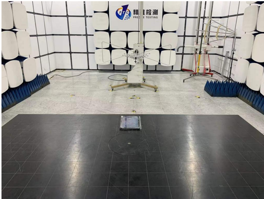
Radiated emission
