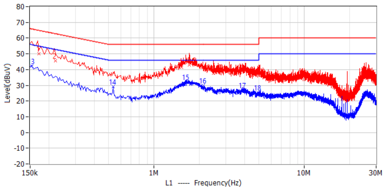
L Line
