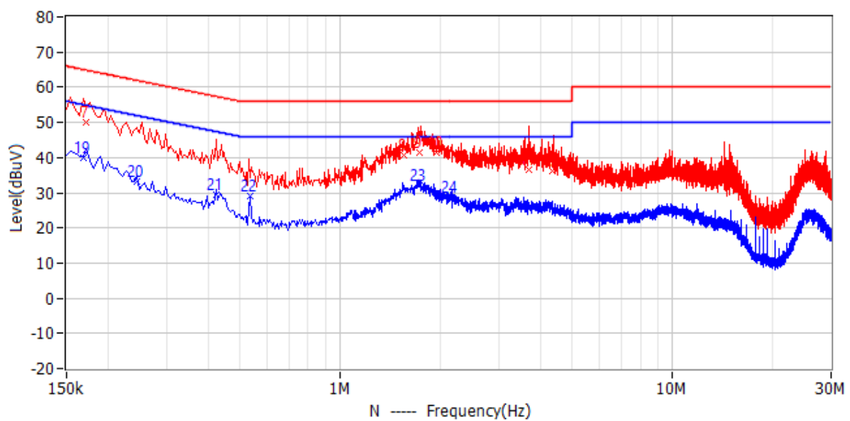
N Line
