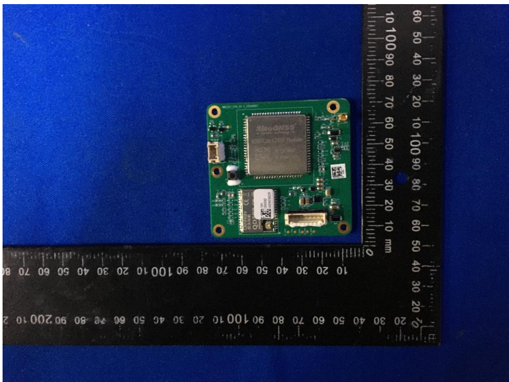
(32) EUT Photo
