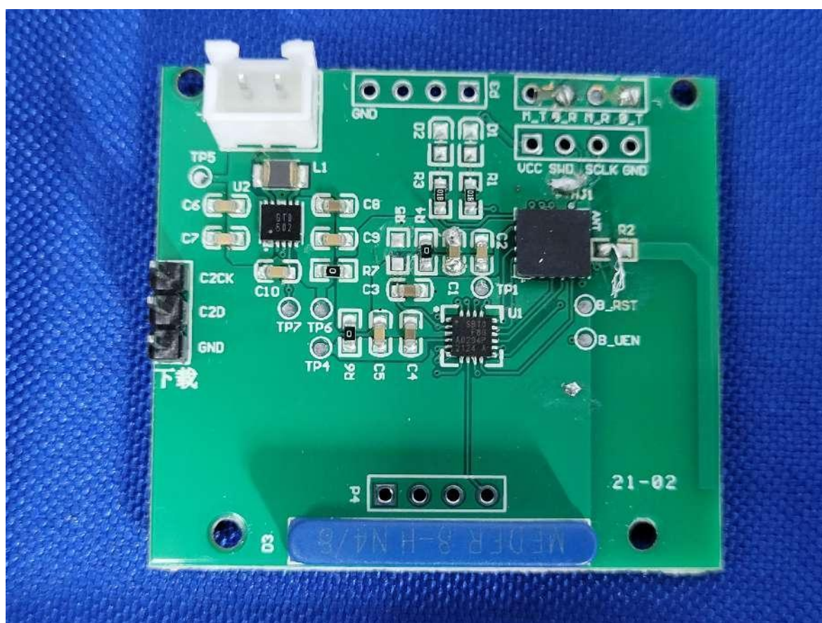
MAIN BOARD TOP SPECIAL VIEW
