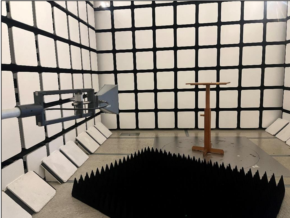
Photo 2: Measurement above 1 GHz ( 1GHz to 18 GHz)
