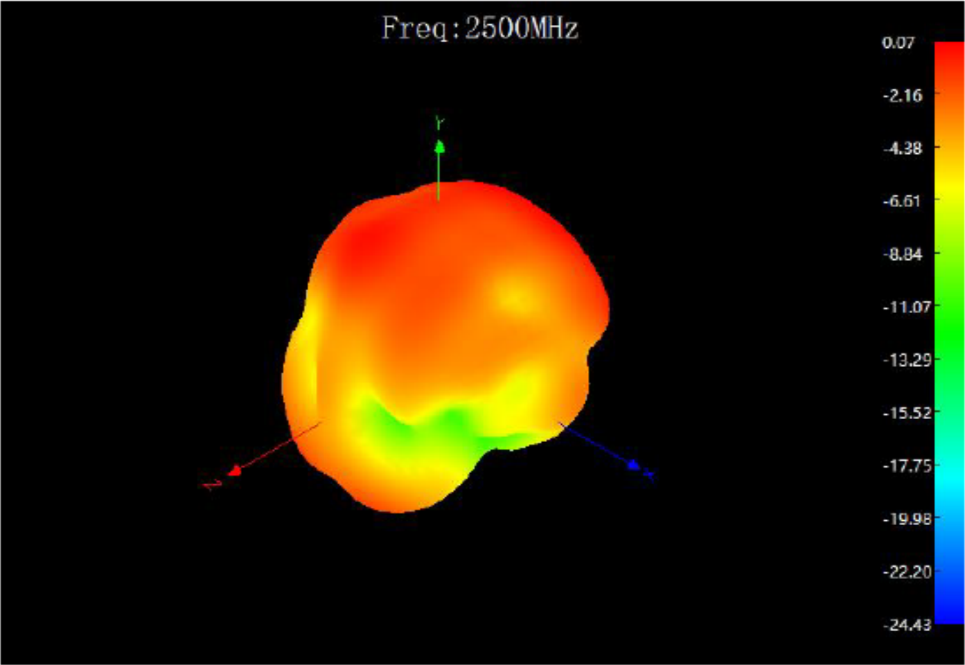
3D antenna gain diagram
