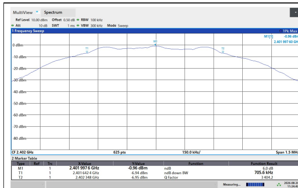
DTS BW, 2402 MHz, 1Mb
