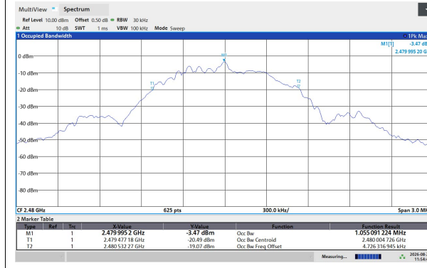
99% Occupied BW, 2480 MHz, 1Mb
