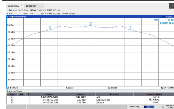
DTS BW, 2440 MHz, 1Mb
