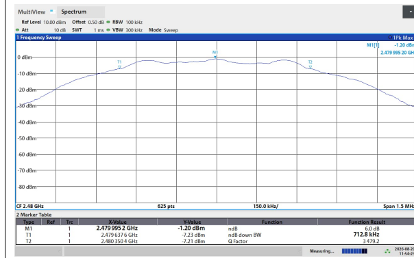
DTS BW, 2480 MHz, 1Mb
