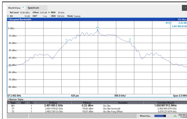
99% Occupied BW, 2402 MHz, 1Mb
