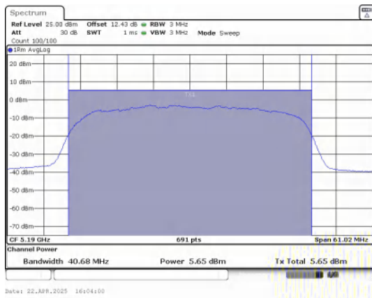
Conducted AVG output power IEEE 802.11n_40_Channel 38_Antenna 0
