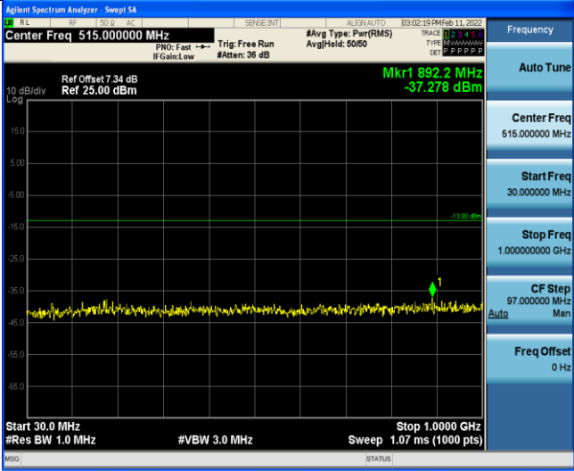
Band4-1.4MHz-16QAM-20393-1RB#0-Range3:30~1000MHz
