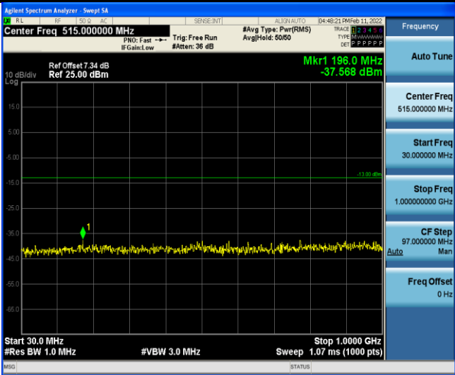
Band4-3MHz-16QAM-20175-1RB#0-Range3:30~1000MHz
