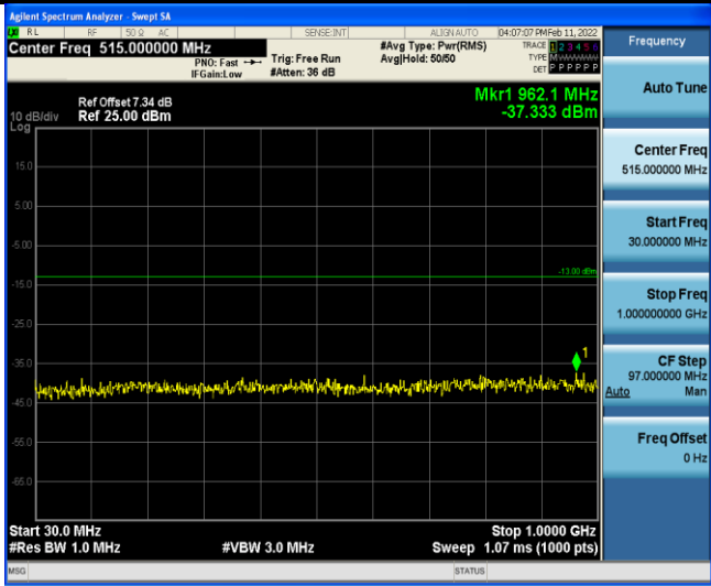
Band4-15MHz-16QAM-20175-1RB#0-Range3:30~1000MHz
