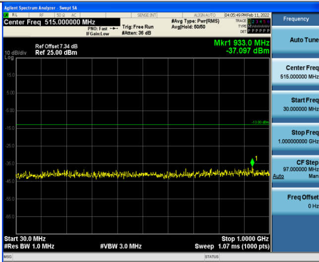
Band4-15MHz-16QAM-20025-1RB#0-Range3:30~1000MHz
