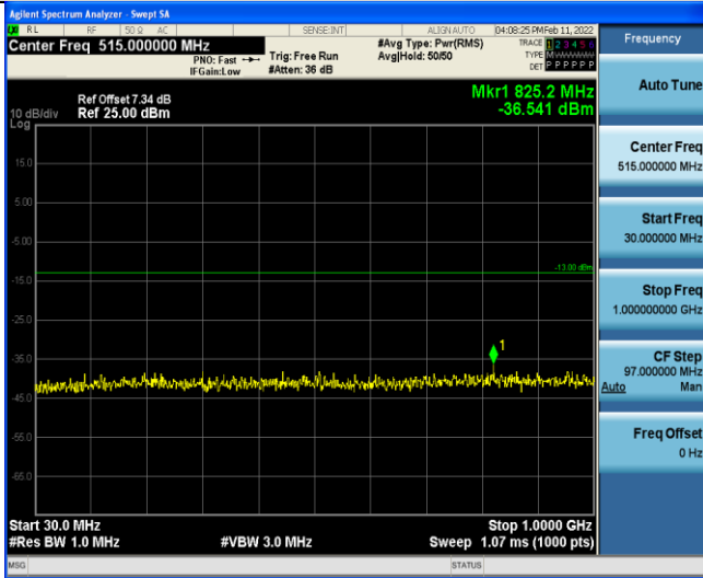
Band4-15MHz-16QAM-20325-1RB#0-Range3:30~1000MHz
