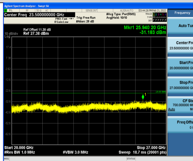
Band7-5MHz-16QAM-21100-1RB#0-Range3:20000~27000MHz
