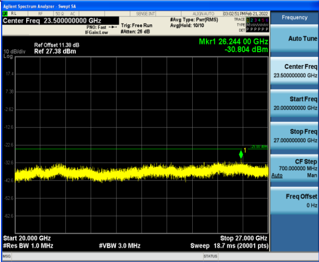
Band7-5MHz-16QAM-20775-1RB#0-Range5:20000~27000MHz
