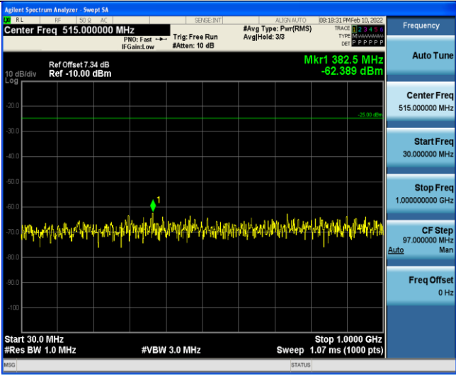
Band7-5MHz-16QAM-21425-1RB#0-Range3:30~1000MHz
