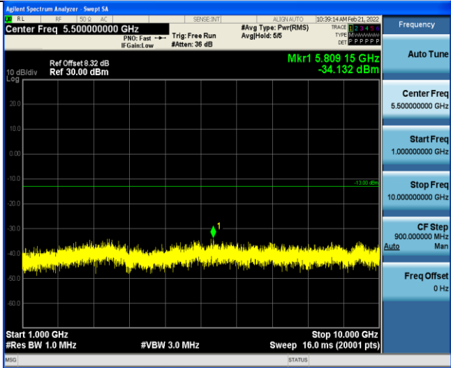
Band12-5MHz-16QAM-23095-1RB#0-Range2:1000~10000MHz
