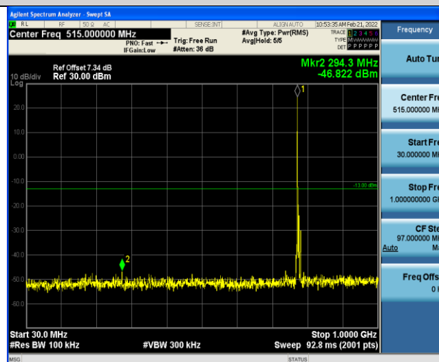
Band13-5MHz-QPSK-23205-1RB#0-Range1:30~1000MHz
