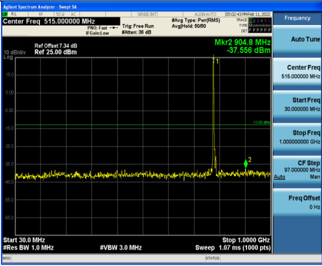
Band13-5MHz-16QAM-23255-1RB#0-Range3:30~1000MHz
