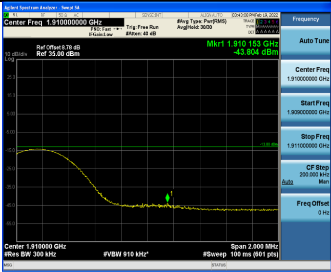
Band2-15MHz-QPSK-19125-1RB#74
