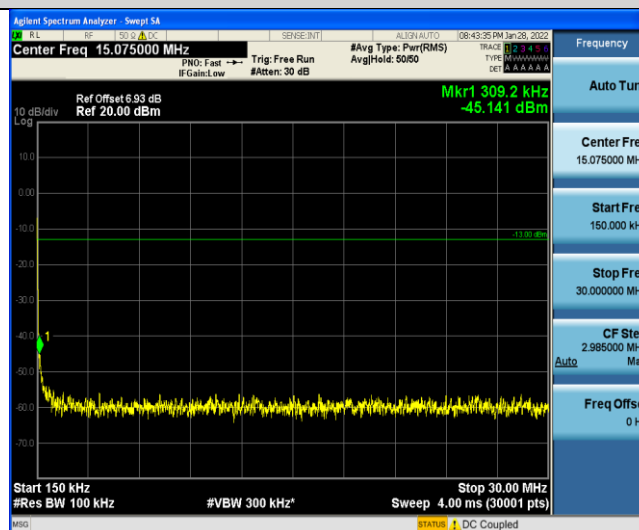
Band V-4233-30~1000MHz
