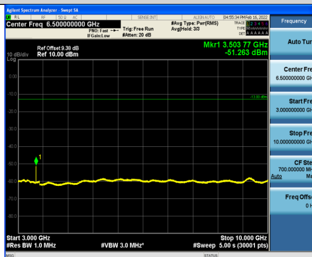
Band IV-1513-10000~20000MHz
