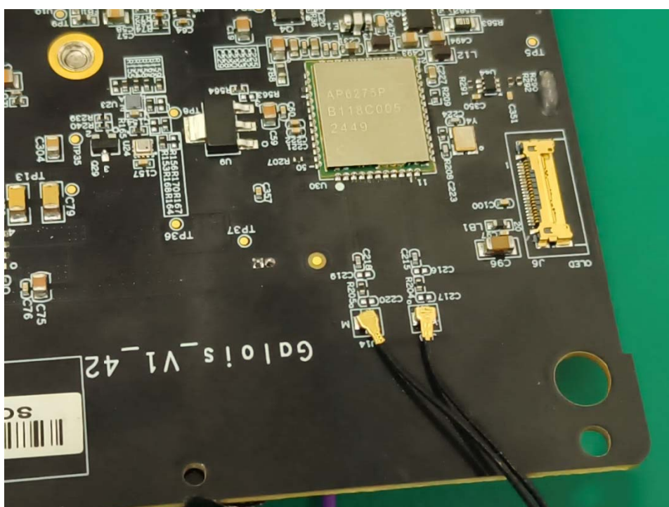
(Antenna connector)
