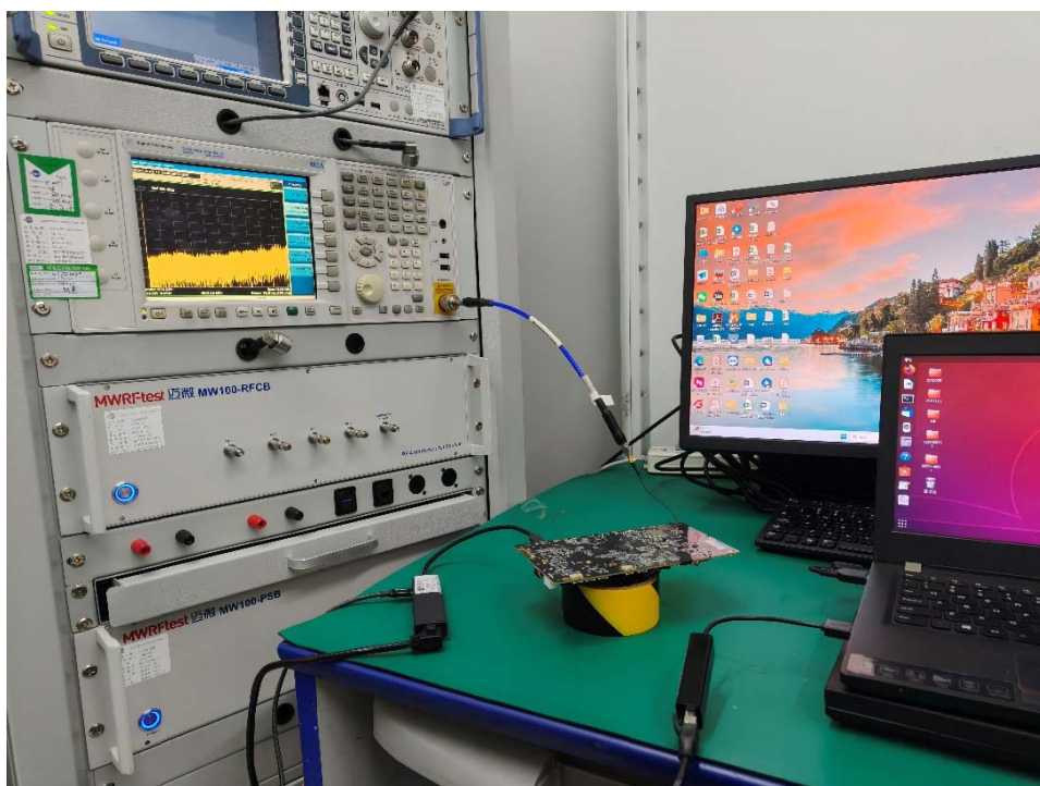
(Bluetooth&WLAN)
