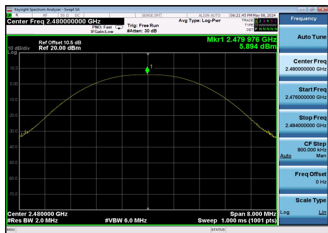
Output Power: 2480MHz
