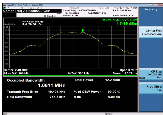
6dB Bandwidth: 2480MHz
