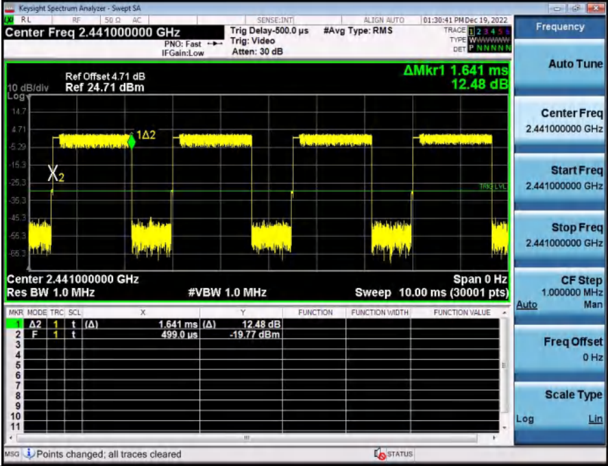
Dwell Time (Hopping) BT 3-DH3 2441 One Burst Time
