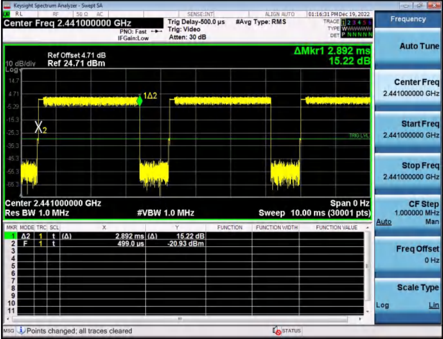
Dwell Time (Hopping) BT 3-DH5 2441 One Burst Time
