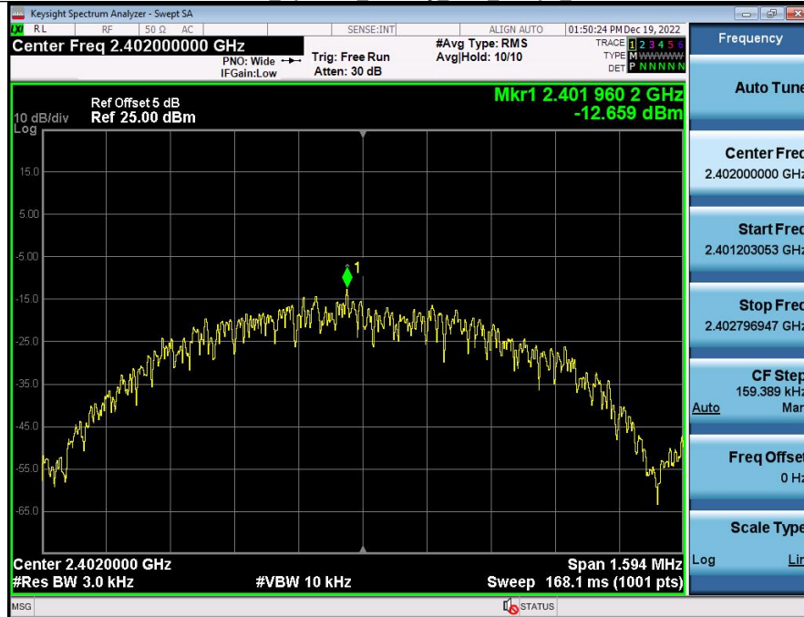
Power_Spectral_Density_BLE_1Mbps_2402
