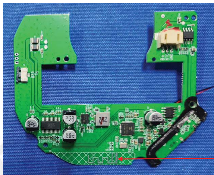
Bluetooth Antenna
