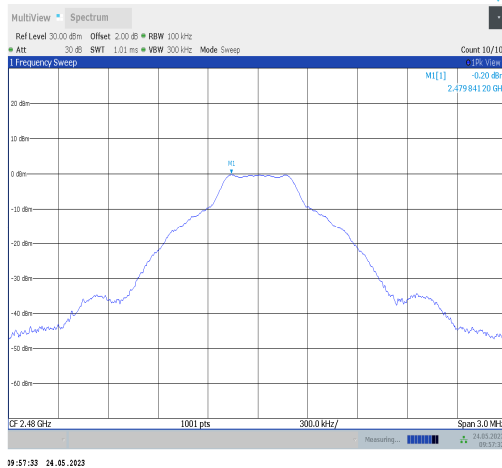
BLE_1M-Ant0-2480-0~Reference
