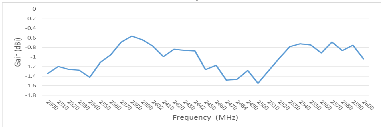
Peak Gain
