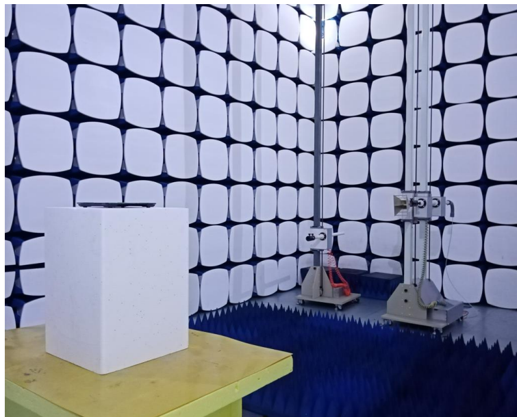
Radiated emission above 1GHz
