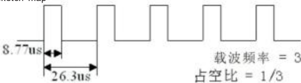
载波示意图 Carrier sketch map
