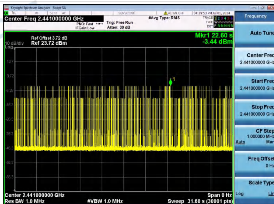
Dwell_Time_(Hopping)_NVNT_ANT1_1-DH5_2441_00_Accumulated
