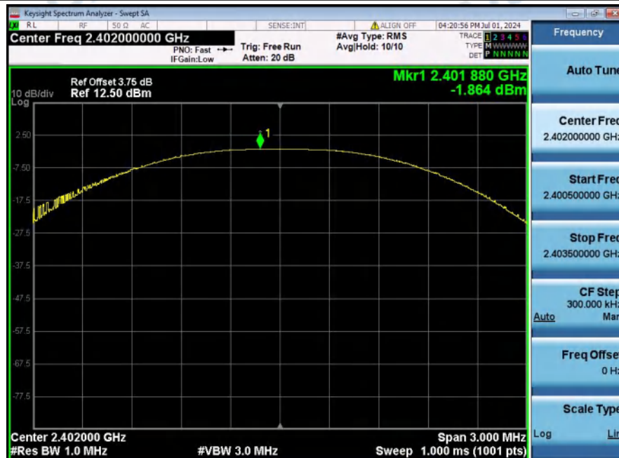
Peak_Output_Power_NVNT_ANT1_1-DH5_2402_00
