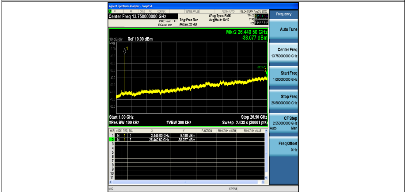
SRD-Ant1-2445-1000~26500-PASS
