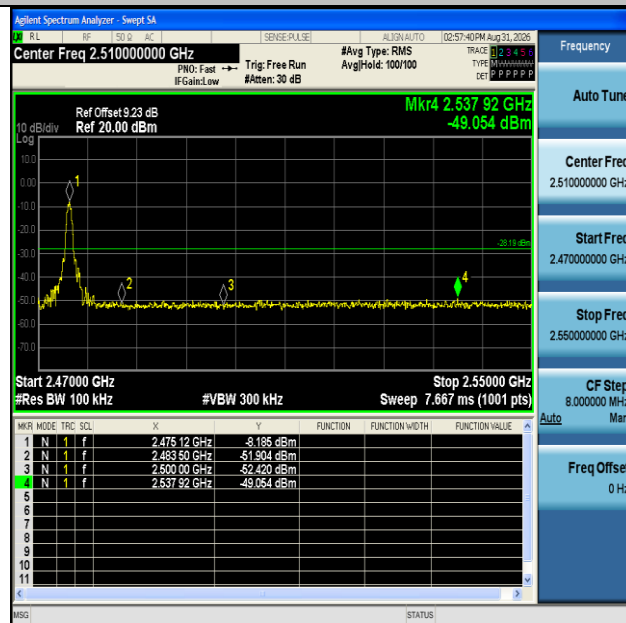
SRD-Ant1-2475-PASS
