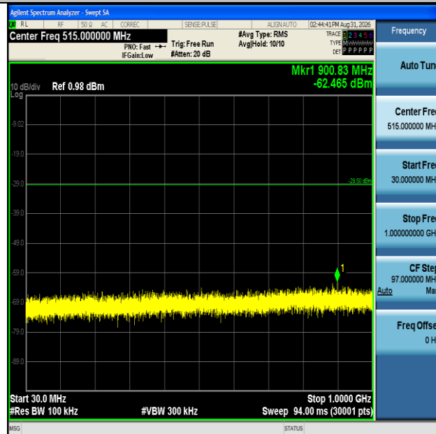
SRD-Ant1-2405-30~1000-PASS
