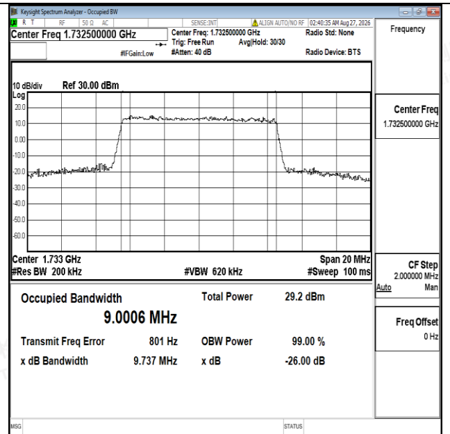
Band4-10MHz-16QAM-20175-50RB#0-PASS
