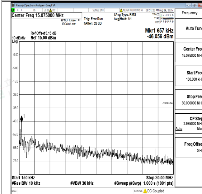
Band4-1.4MHz-16QAM-20175-1RB#0-0.15~30-PASS
