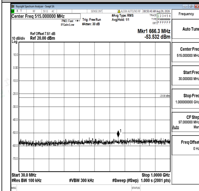
Band4-1.4MHz-QPSK-20175-1RB#0-30~1000-PASS
