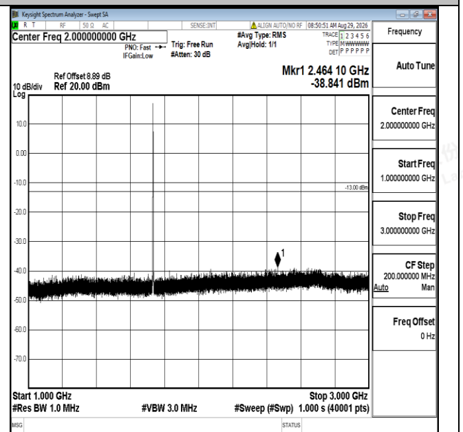
Band4-1.4MHz-QPSK-20175-1RB#0-1000~3000-PASS
