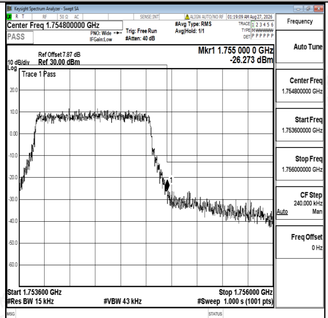
Band4-1.4MHz-16QAM-20393-6RB#0-PASS
