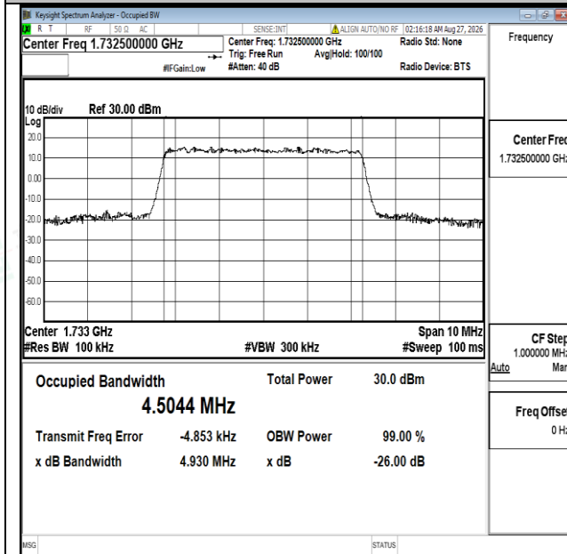
Band4-5MHz-QPSK-20175-25RB#0-PASS
