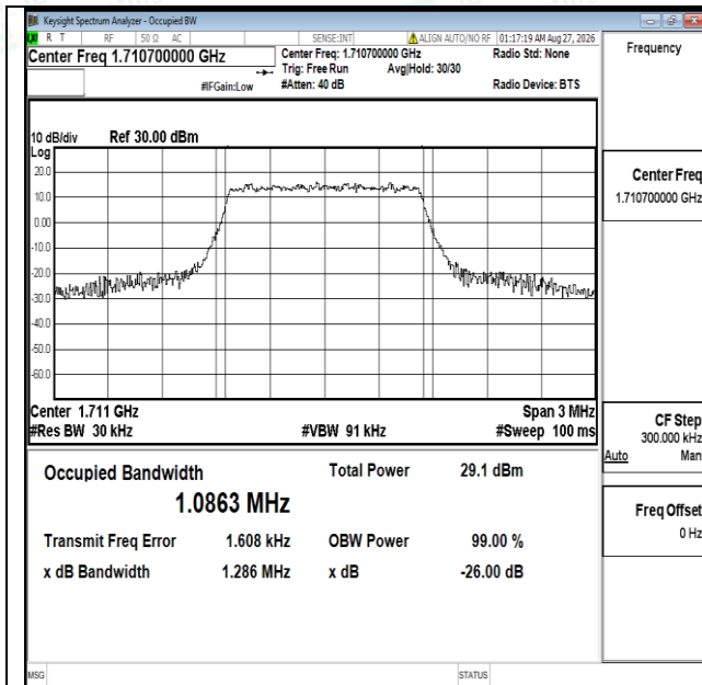
Band4-1.4MHz-QPSK-19957-6RB#0-PASS
