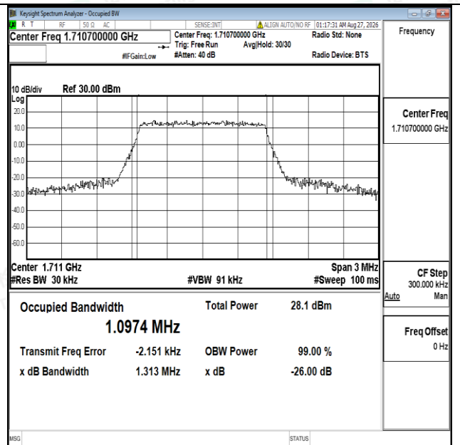
Band4-1.4MHz-16QAM-19957-6RB#0-PASS
