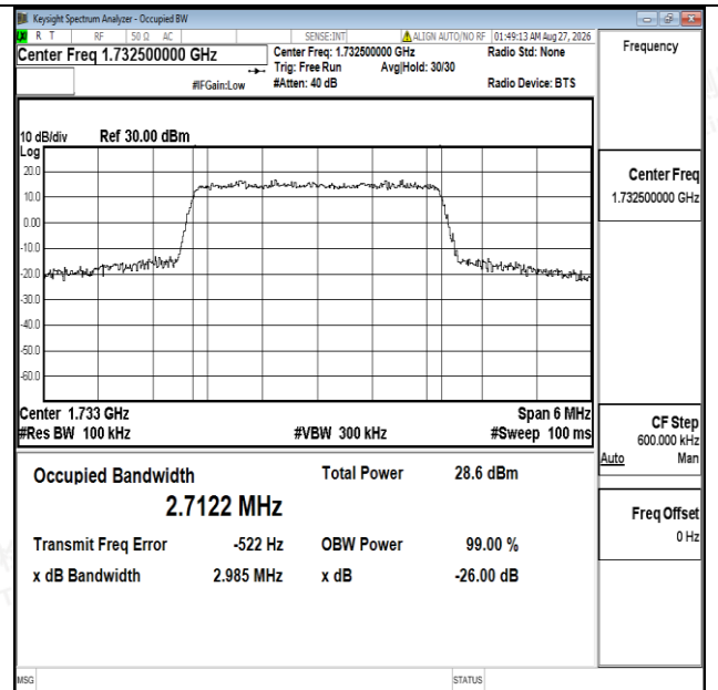
Band4-3MHz-16QAM-20175-15RB#0-PASS
