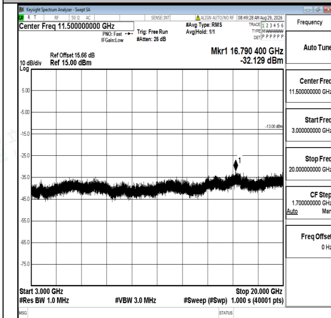
Band4-1.4MHz-QPSK-19957-1RB#0-3000~20000-PASS
