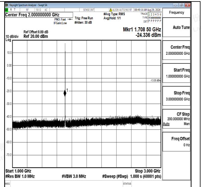
Band4-1.4MHz-QPSK-19957-1RB#0-1000~3000-PASS
