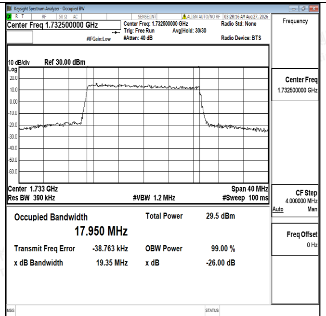
Band4-20MHz-16QAM-20175-100RB#0-PASS
