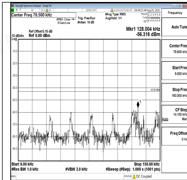
Band4-1.4MHz-QPSK-19957-1RB#0-0.009~0.15-PASS
