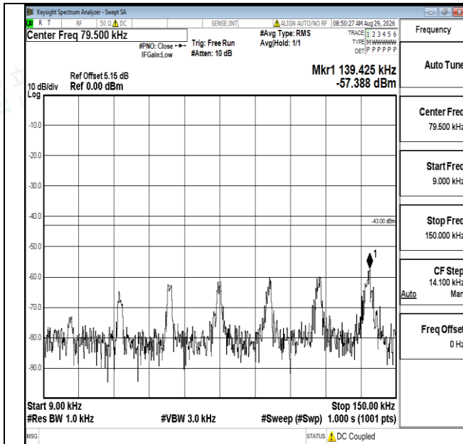
Band4-1.4MHz-QPSK-20175-1RB#0-0.009~0.15-PASS
