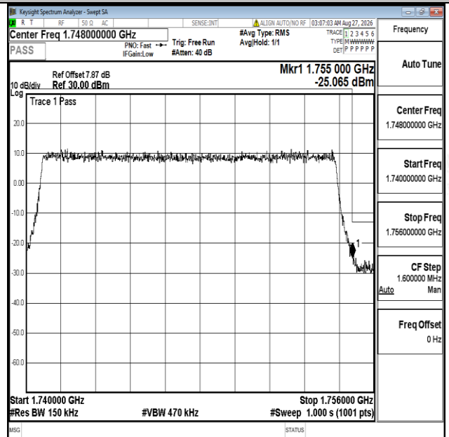
Band4-15MHz-16QAM-20325-75RB#0-PASS
