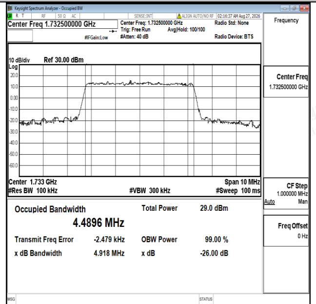
Band4-5MHz-16QAM-20175-25RB#0-PASS
