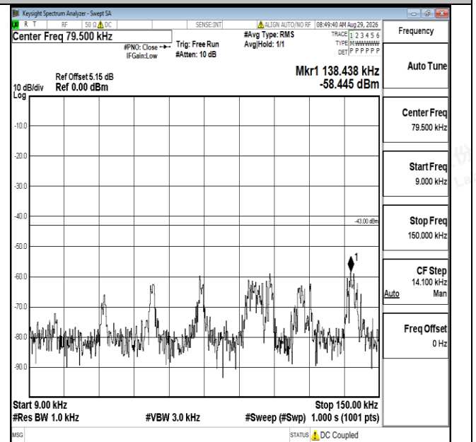
Band4-1.4MHz-16QAM-19957-1RB#0-0.009~0.15-PASS
