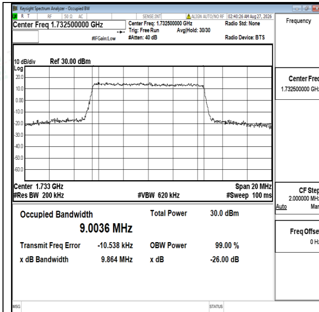
Band4-10MHz-QPSK-20175-50RB#0-PASS
