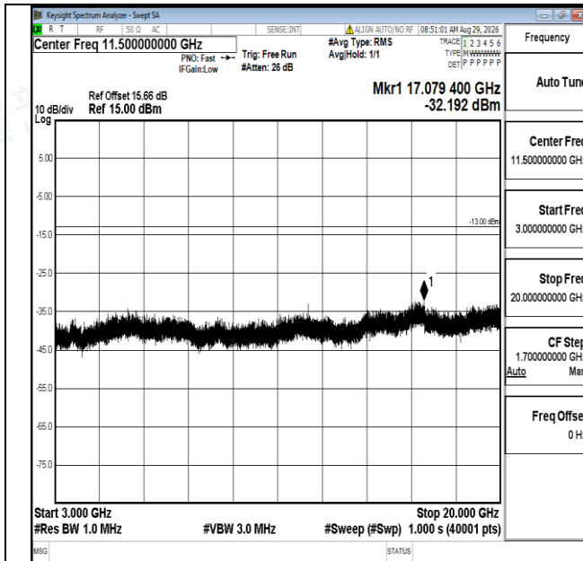
Band4-1.4MHz-QPSK-20175-1RB#0-3000~20000-PASS
