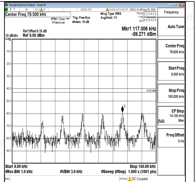
Band4-1.4MHz-16QAM-20175-1RB#0-0.009~0.15-PASS
