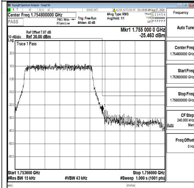
Band4-1.4MHz-QPSK-20393-6RB#0-PASS
