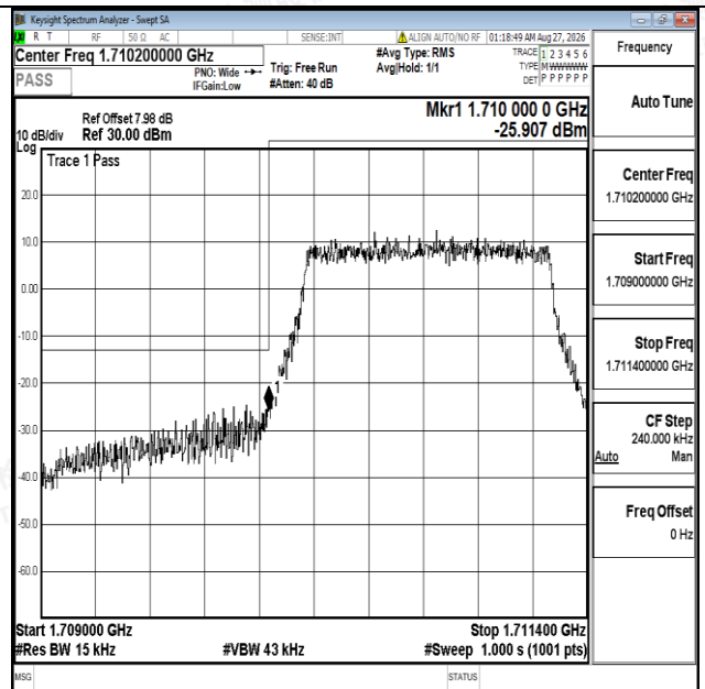
Band4-1.4MHz-16QAM-19957-6RB#0-PASS
