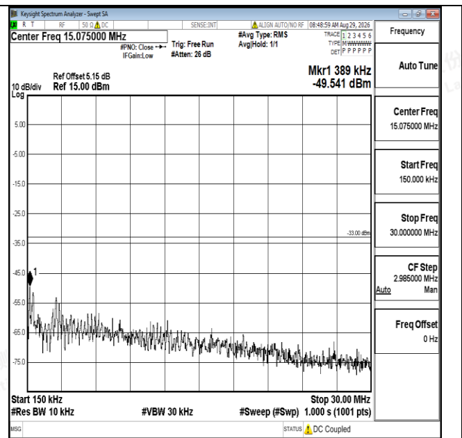
Band4-1.4MHz-QPSK-19957-1RB#0-0.15~30-PASS
