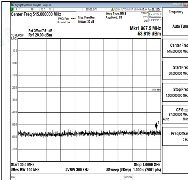
Band4-1.4MHz-QPSK-19957-1RB#0-30~1000-PASS
