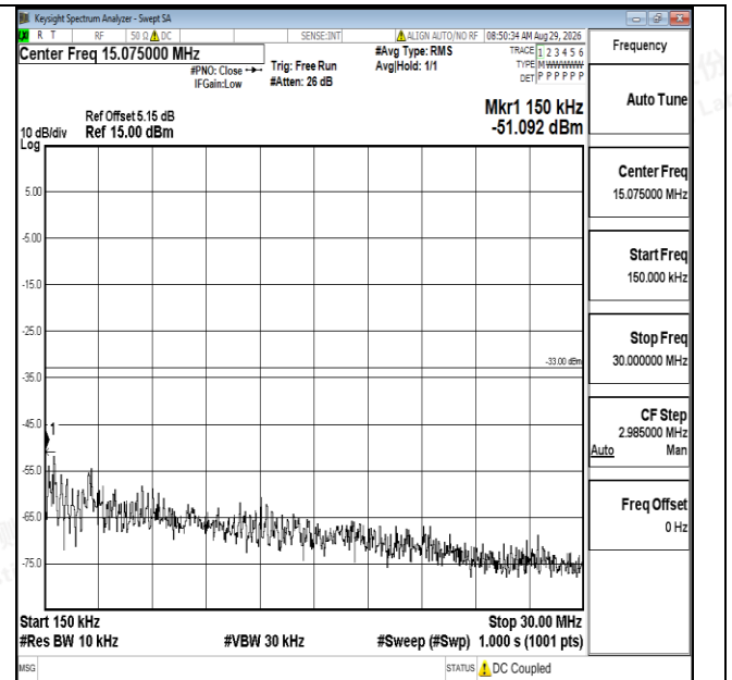
Band4-1.4MHz-QPSK-20175-1RB#0-0.15~30-PASS
