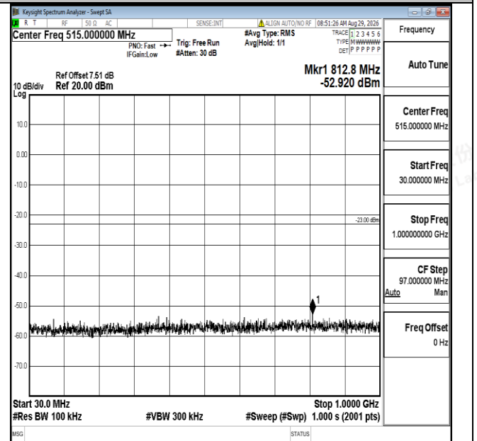
Band4-1.4MHz-16QAM-20175-1RB#0-30~1000-PASS
