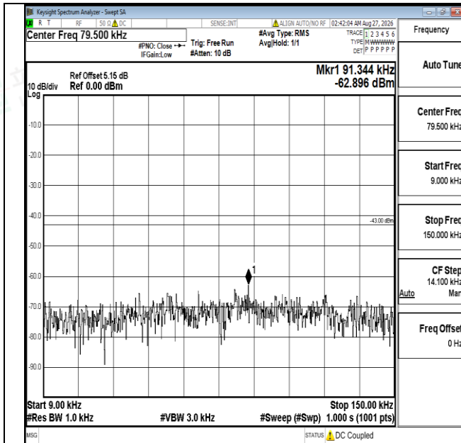
Band4-10MHz-QPSK-20000-1RB#0-0.009~0.15-PASS
