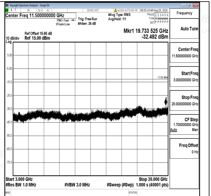
Band4-3MHz-16QAM-19965-1RB#0-3000-20000-PASS
