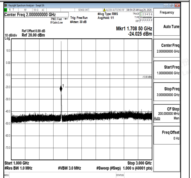
Band4-3MHz-QPSK-19965-1RB#0-1000~3000-PASS
