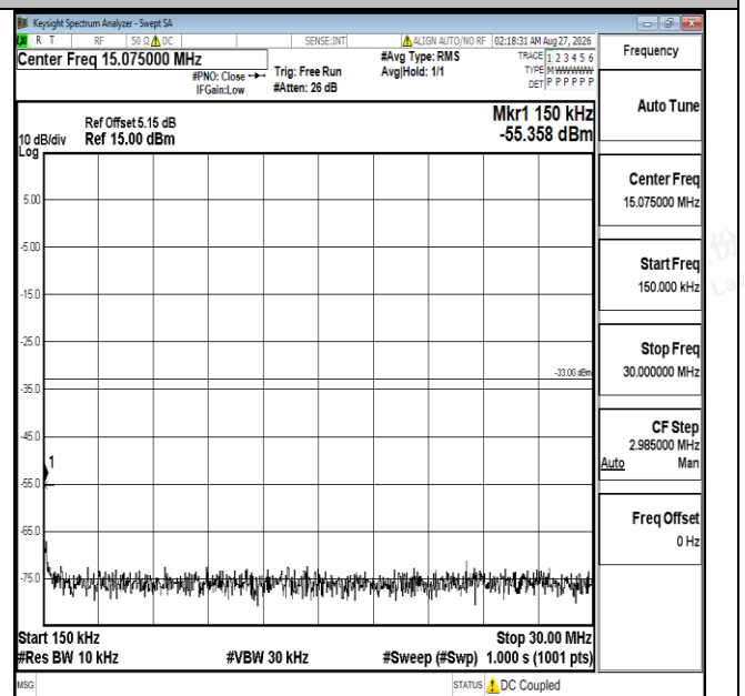
Band4-5MHz-QPSK-19975-1RB#0-0.15~30-PASS
