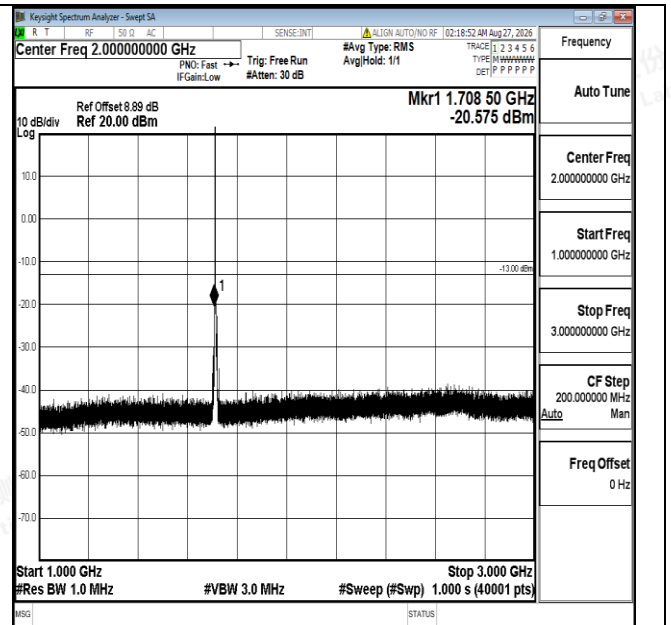
Band4-5MHz-QPSK-19975-1RB#0-1000~3000-PASS
