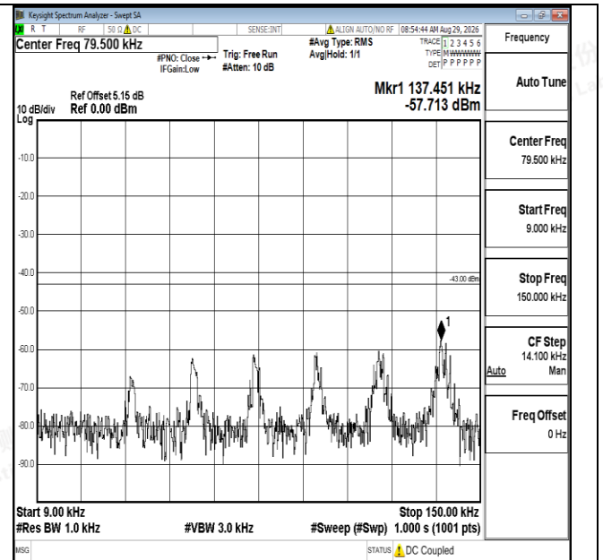
Band4-3MHz-16QAM-19965-1RB#0-0.009~0.15-PASS
