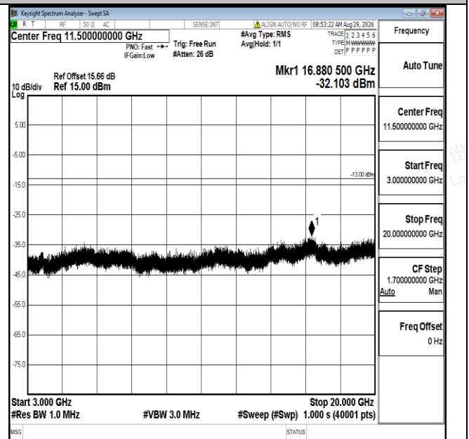
Band4-1.4MHz-16QAM-20393-1RB#0-3000~20000-PASS
