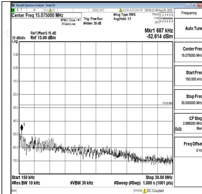
Band4-3MHz-16QAM-20175-1RB#0-0.15~30-PASS
