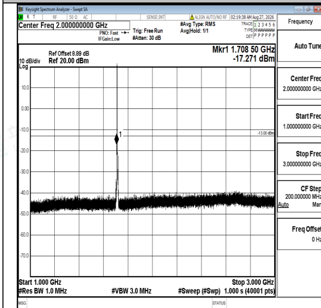
Band4-5MHz-16QAM-19975-1RB#0-1000~3000-PASS
