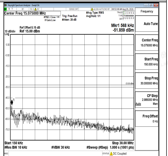
Band4-1.4MHz-QPSK-20393-1RB#0-0.15~30-PASS
