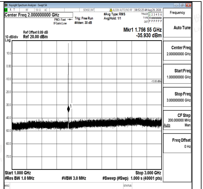
Band4-1.4MHz-QPSK-20393-1RB#0-1000~3000-PASS
