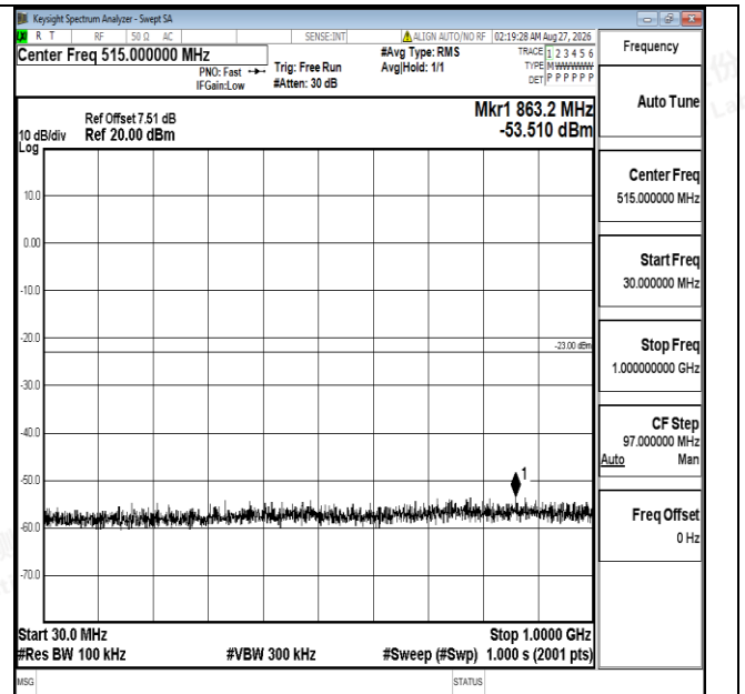
Band4-5MHz-16QAM-19975-1RB#0-30~1000-PASS
