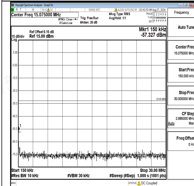
Band4-10MHz-16QAM-20000-1RB#0-0.15~30-PASS
