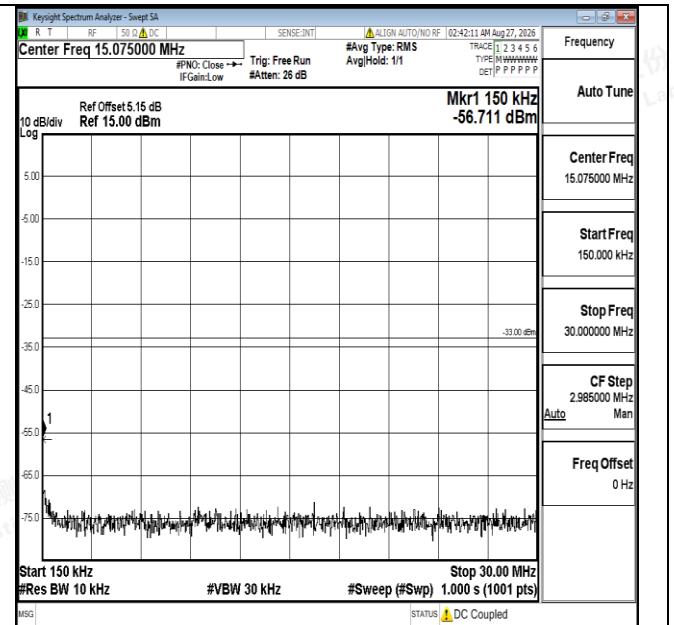
Band4-10MHz-QPSK-20000-1RB#0-0.15~30-PASS
