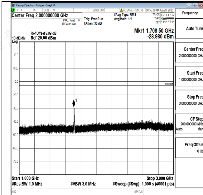
Band4-3MHz-16QAM-19965-1RB#0-1000-3000-PASS
