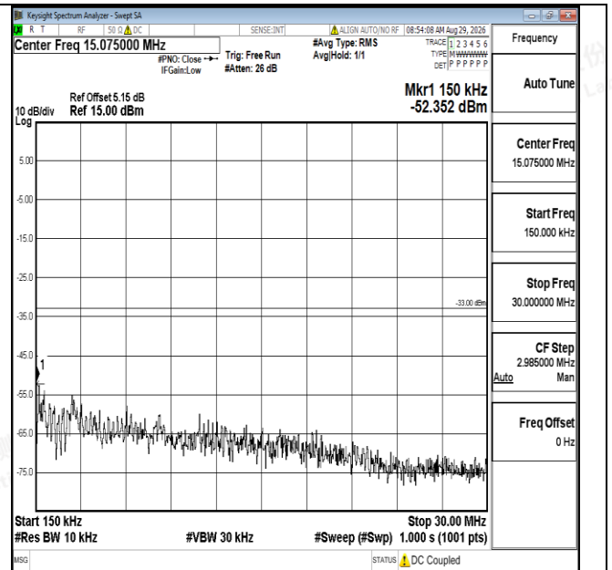
Band4-3MHz-QPSK-19965-1RB#0-0.15~30-PASS
