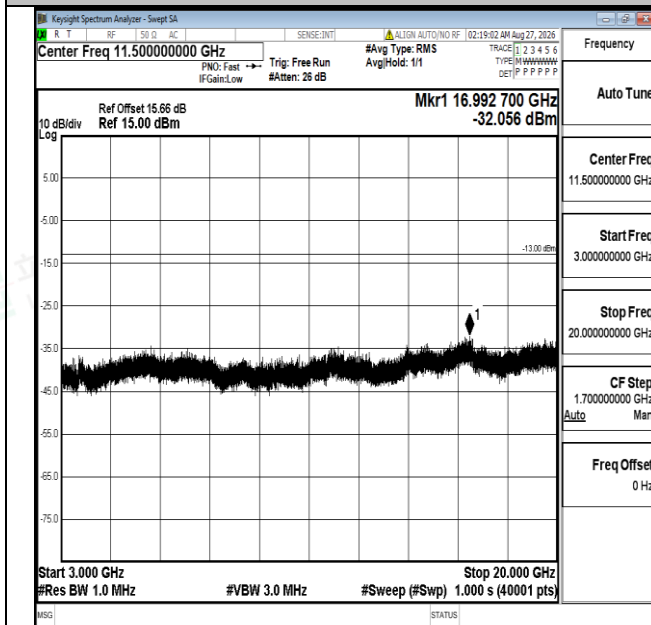
Band4-5MHz-QPSK-19975-1RB#0-3000~20000-PASS
