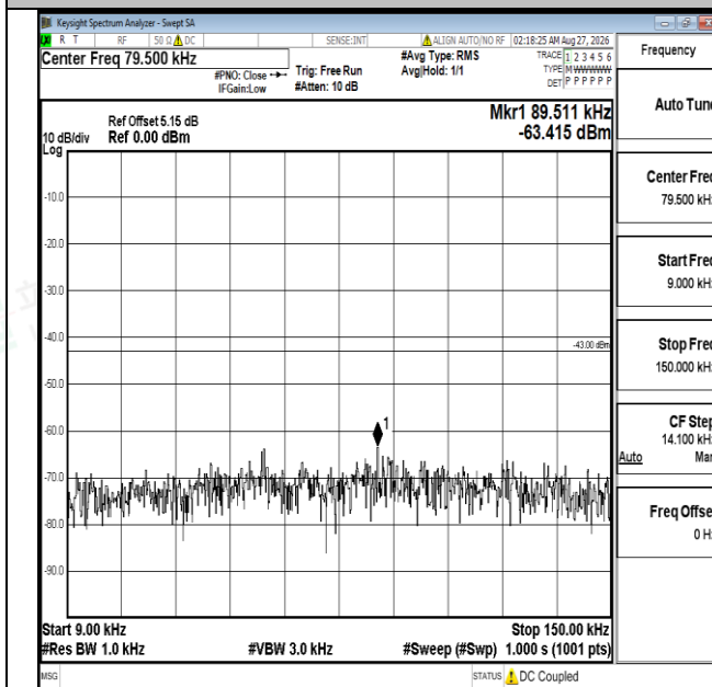
Band4-5MHz-QPSK-19975-1RB#0-0.009~0.15-PASS
