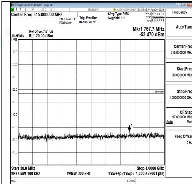
Band4-3MHz-QPSK-20175-1RB#0-30~1000-PASS
