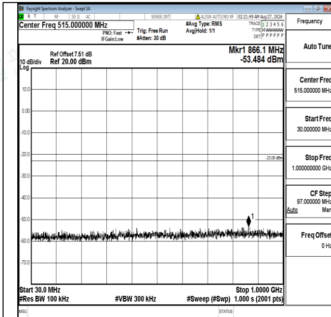
Band4-5MHz-QPSK-20375-1RB#0-30~1000-PASS
