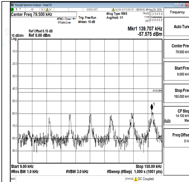
Band4-3MHz-QPSK-19965-1RB#0-0.009~0.15-PASS
