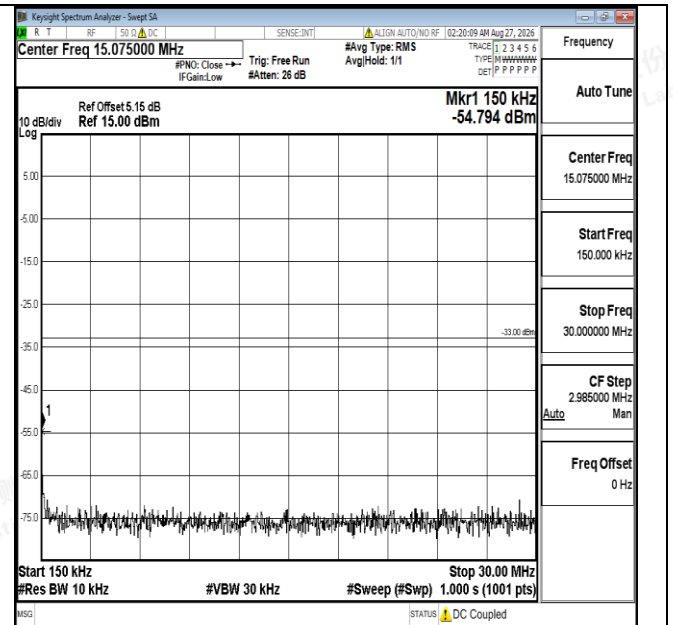
Band4-5MHz-QPSK-20175-1RB#0-0.15~30-PASS
