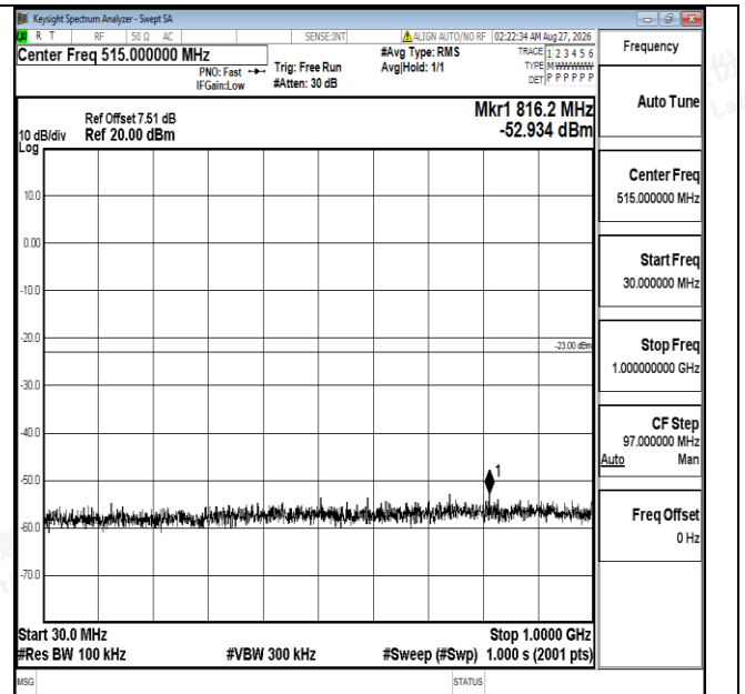
Band4-5MHz-16QAM-20375-1RB#0-30~1000-PASS
