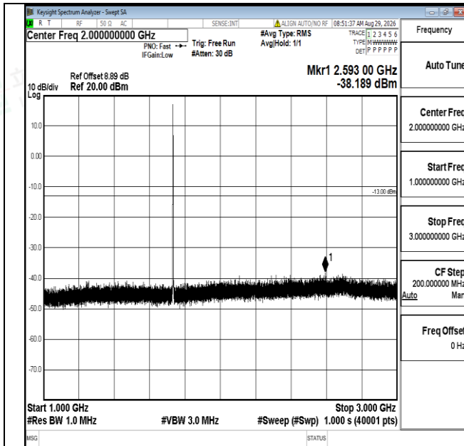
Band4-1.4MHz-16QAM-20175-1RB#0-1000~3000-PASS
