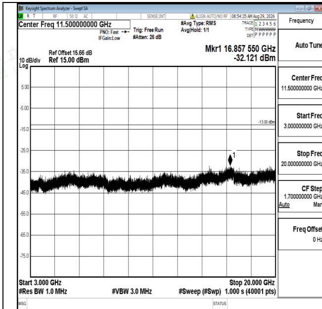
Band4-3MHz-QPSK-19965-1RB#0-3000~20000-PASS
