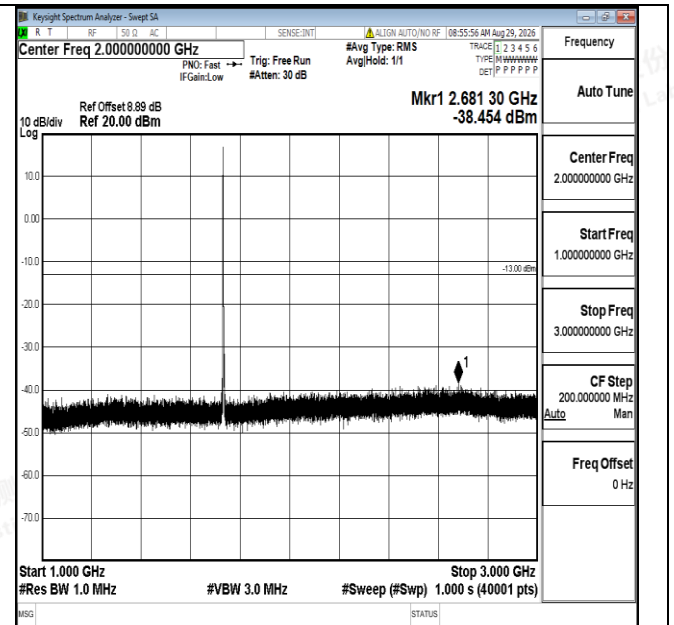
Band4-3MHz-QPSK-20175-1RB#0-1000~3000-PASS
