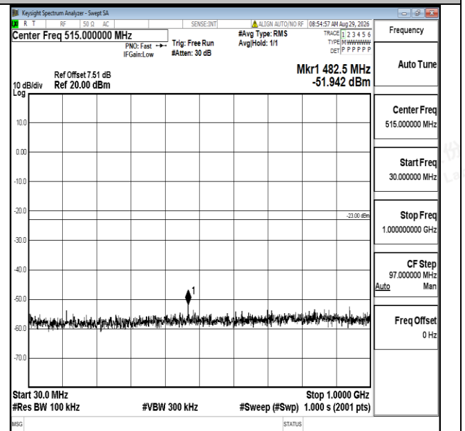
Band4-3MHz-16QAM-19965-1RB#0-30~1000-PASS
