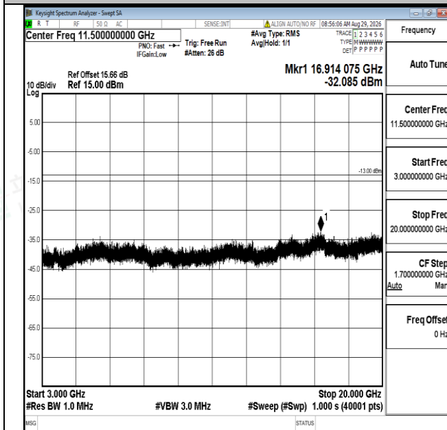
Band4-3MHz-QPSK-20175-1RB#0-3000~20000-PASS
