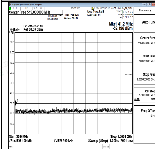
Band4-3MHz-QPSK-20385-1RB#0-30~1000-PASS
