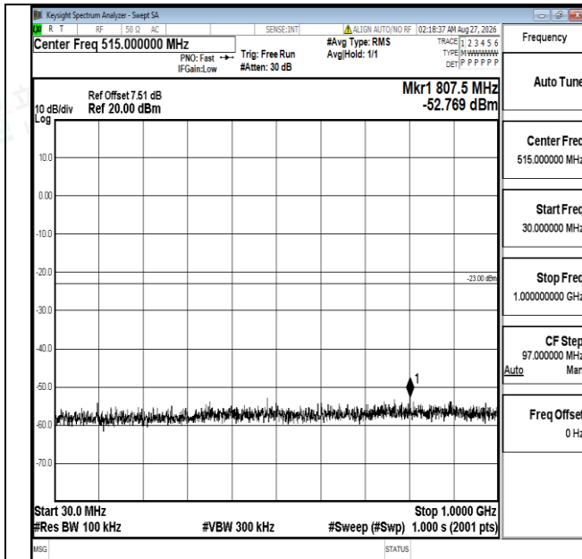
Band4-5MHz-QPSK-19975-1RB#0-30~1000-PASS
