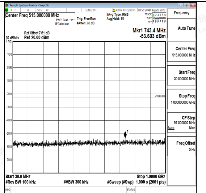
Band4-3MHz-16QAM-20175-1RB#0-30~1000-PASS
