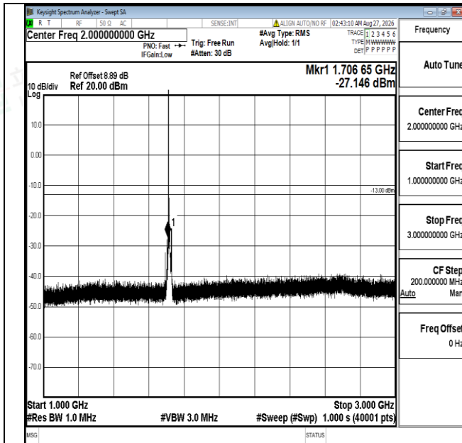
Band4-10MHz-16QAM-20000-1RB#0-1000~3000-PASS
