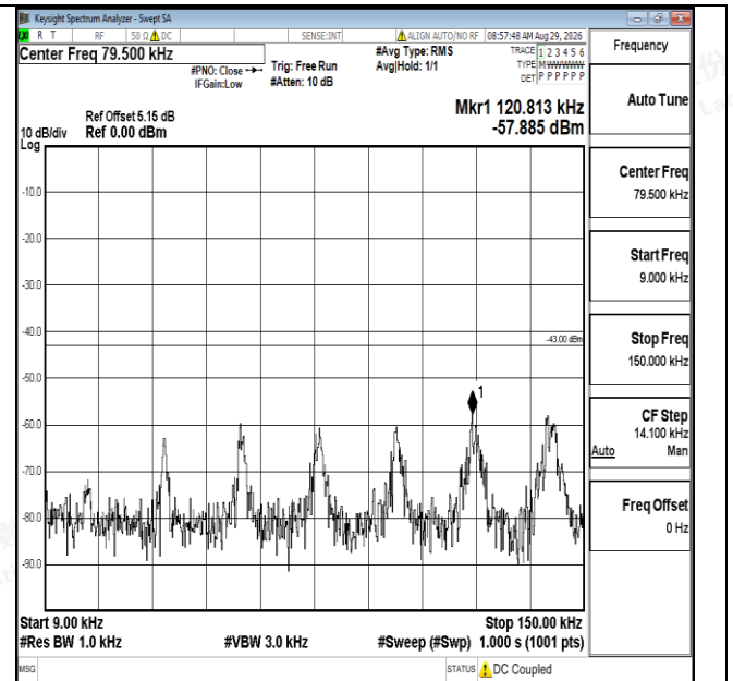
Band4-3MHz-16QAM-20385-1RB#0-0.009~0.15-PASS
