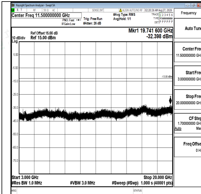
Band4-5MHz-QPSK-20175-1RB#0-3000~20000-PASS
