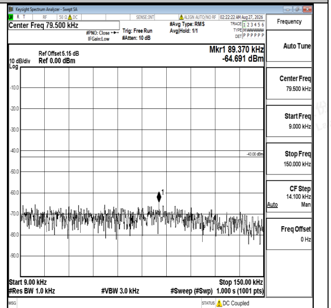
Band4-5MHz-16QAM-20375-1RB#0-0.009~0.15-PASS
