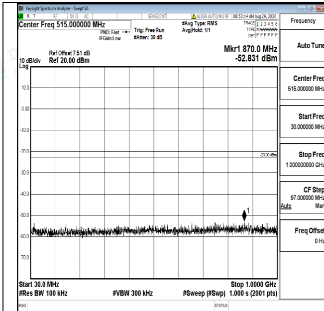
Band4-1.4MHz-QPSK-20393-1RB#0-30~1000-PASS
