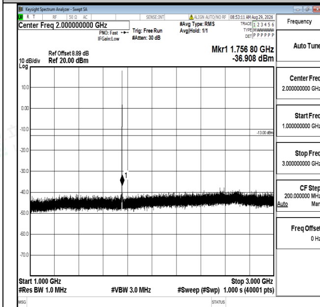
Band4-1.4MHz-16QAM-20393-1RB#0-1000~3000-PASS
