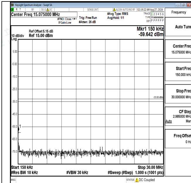
Band4-5MHz-16QAM-19975-1RB#0-0.15~30-PASS
