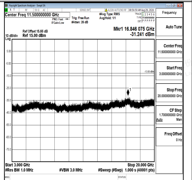
Band4-3MHz-16QAM-20175-1RB#0-3000~20000-PASS
