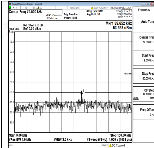
Band4-5MHz-QPSK-20175-1RB#0-0.009~0.15-PASS
