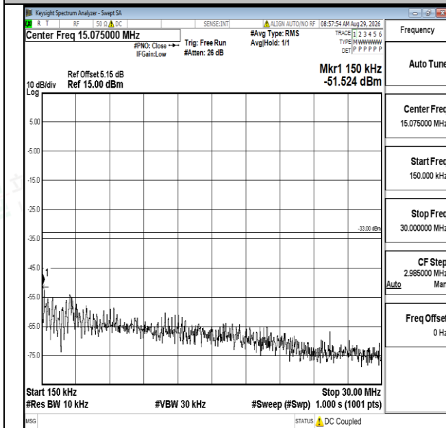
Band4-3MHz-16QAM-20385-1RB#0-0.15~30-PASS
