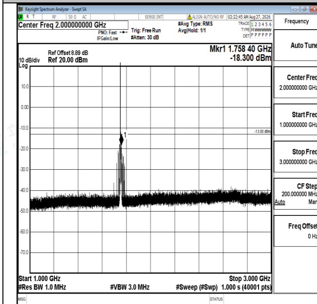
Band4-5MHz-16QAM-20375-1RB#0-1000~3000-PASS
