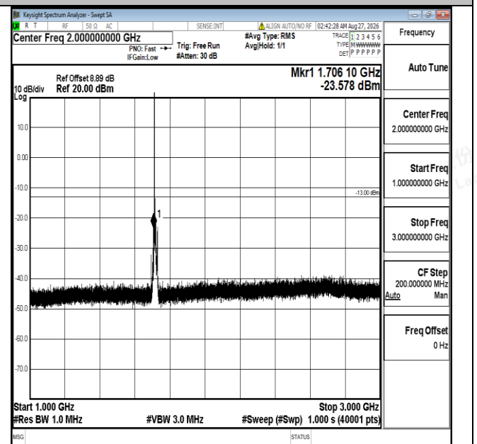
Band4-10MHz-QPSK-20000-1RB#0-1000~3000-PASS
