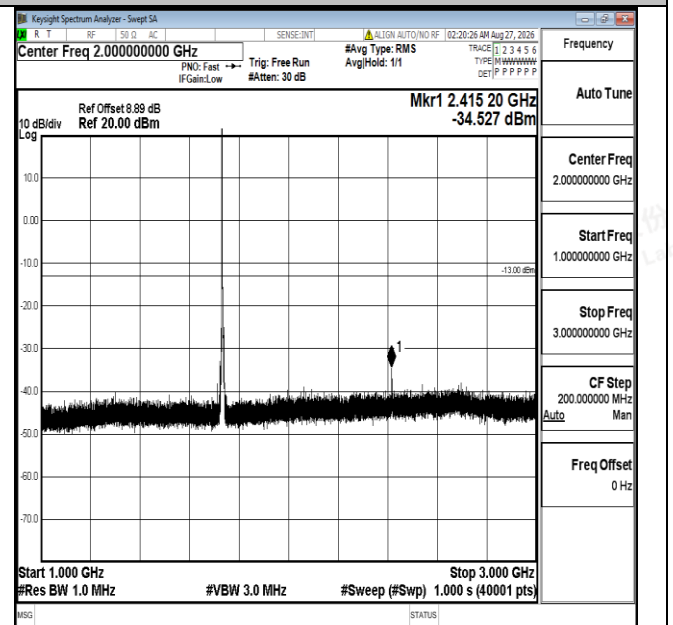
Band4-5MHz-QPSK-20175-1RB#0-1000~3000-PASS
