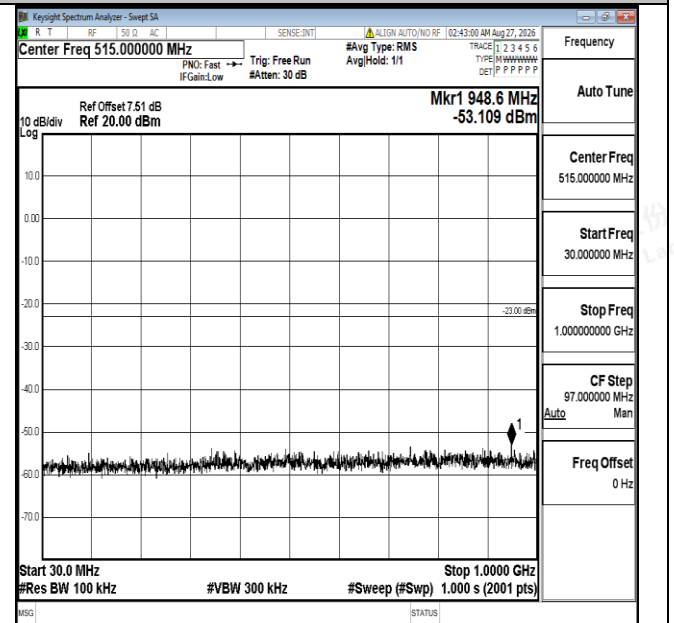
Band4-10MHz-16QAM-20000-1RB#0-30~1000-PASS
