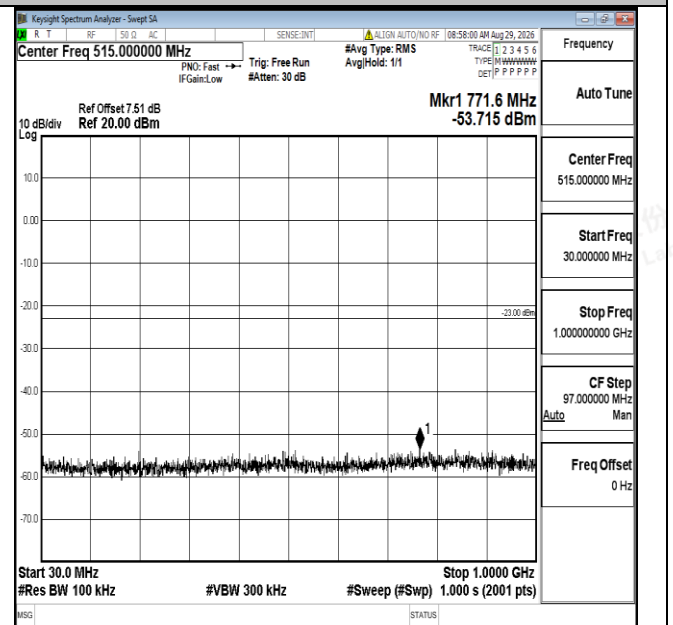
Band4-3MHz-16QAM-20385-1RB#0-30~1000-PASS
