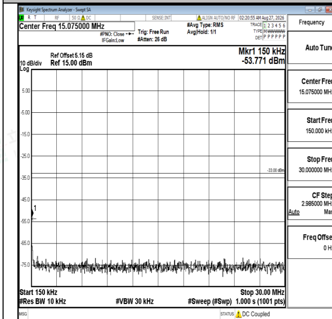
Band4-5MHz-16QAM-20175-1RB#0-0.15~30-PASS
