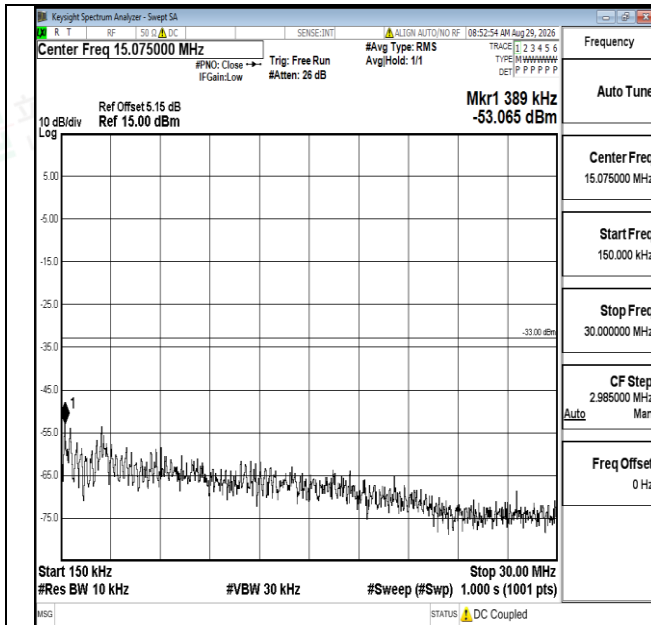
Band4-1.4MHz-16QAM-20393-1RB#0-0.15~30-PASS
