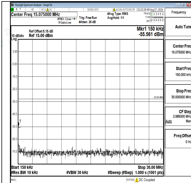
Band4-5MHz-16QAM-20375-1RB#0-0.15~30-PASS
