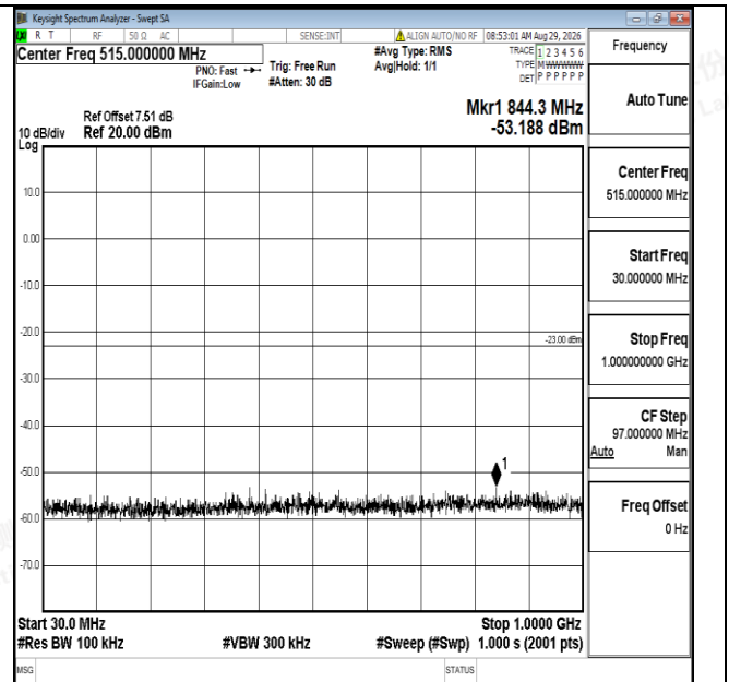
Band4-1.4MHz-16QAM-20393-1RB#0-30~1000-PASS
