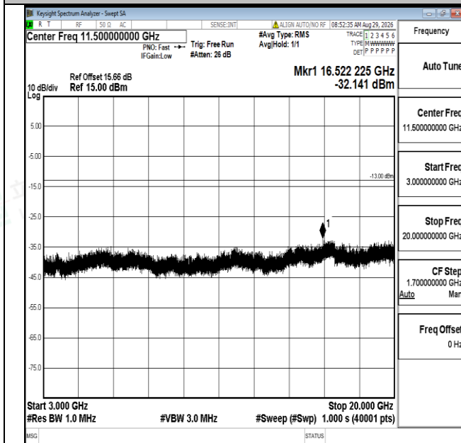
Band4-1.4MHz-QPSK-20393-1RB#0-3000~20000-PASS
