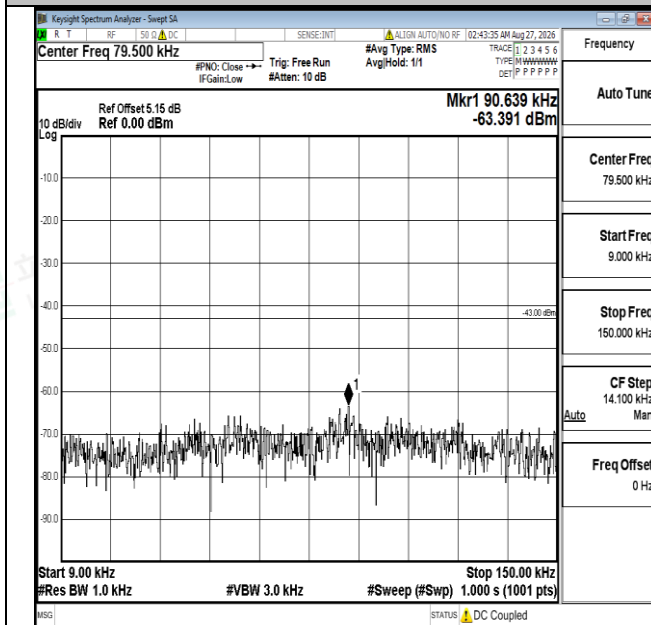
Band4-10MHz-QPSK-20175-1RB#0-0.009~0.15-PASS
