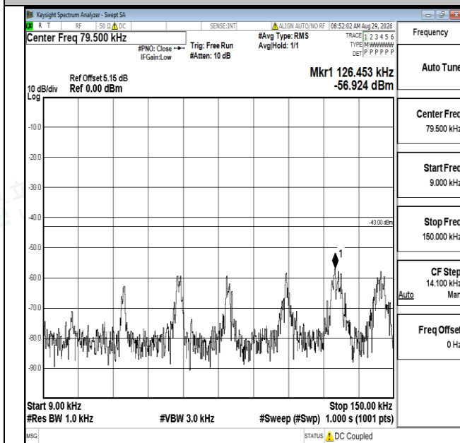
Band4-1.4MHz-QPSK-20393-1RB#0-0.009~0.15-PASS
