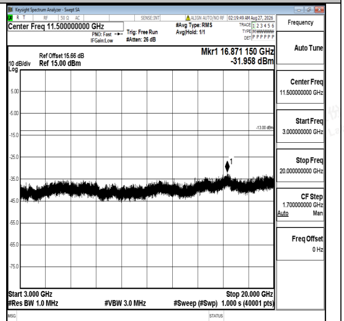
Band4-5MHz-16QAM-19975-1RB#0-3000~20000-PASS
