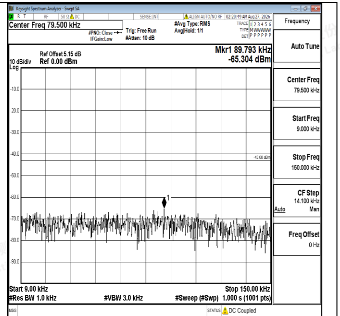
Band4-5MHz-16QAM-20175-1RB#0-0.009~0.15-PASS
