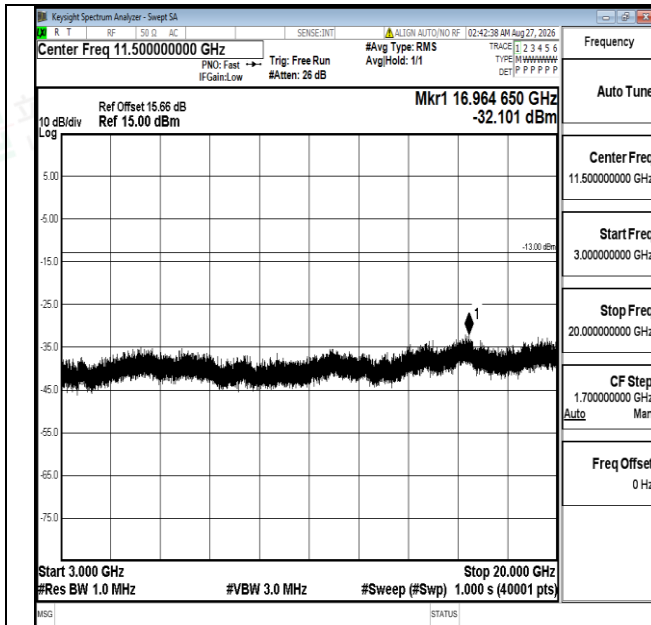
Band4-10MHz-QPSK-20000-1RB#0-3000~20000-PASS
