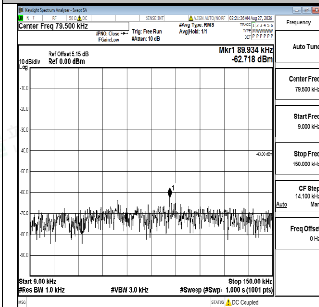
Band4-5MHz-QPSK-20375-1RB#0-0.009~0.15-PASS
