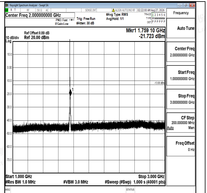
Band4-5MHz-QPSK-20375-1RB#0-1000~3000-PASS
