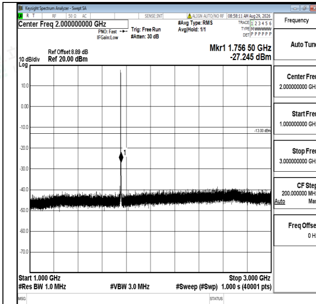
Band4-3MHz-16QAM-20385-1RB#0-1000~3000-PASS
