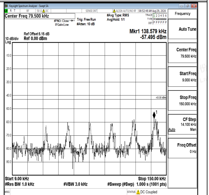
Band4-1.4MHz-16QAM-20393-1RB#0-0.009~0.15-PASS
