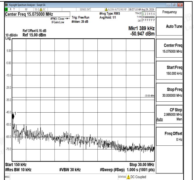
Band4-3MHz-QPSK-20385-1RB#0-0.15~30-PASS
