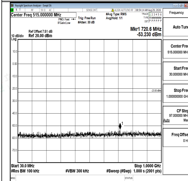
Band4-3MHz-QPSK-19965-1RB#0-30~1000-PASS
