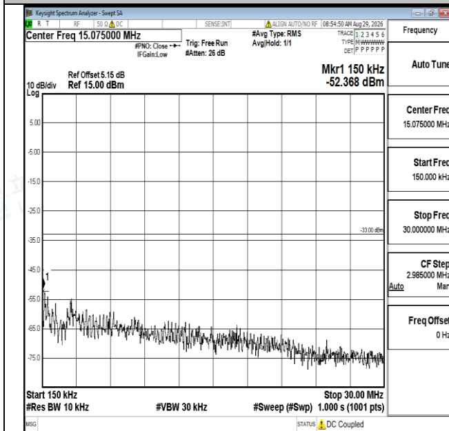
Band4-3MHz-16QAM-19965-1RB#0-0.15~30-PASS
