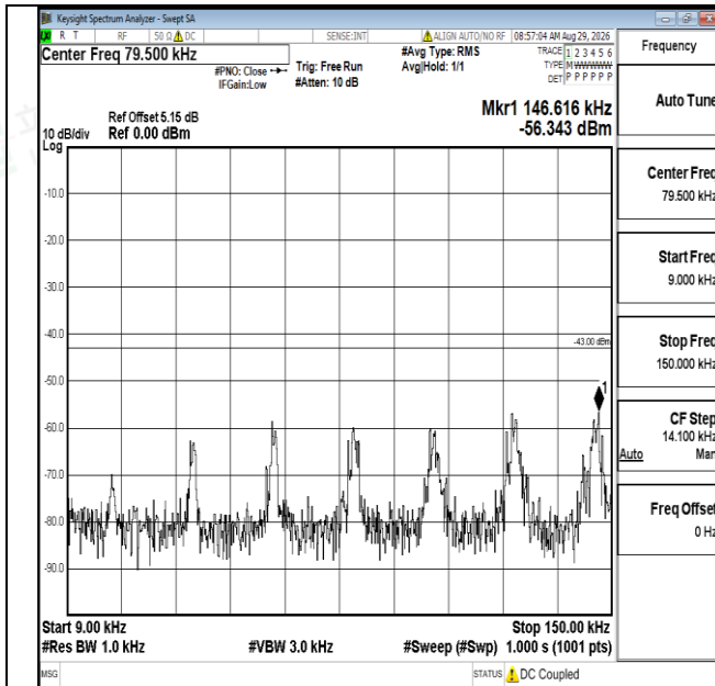
Band4-3MHz-QPSK-20385-1RB#0-0.009~0.15-PASS
