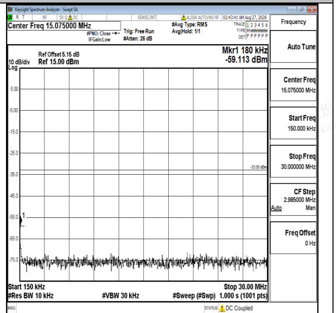
Band4-10MHz-QPSK-20175-1RB#0-0.15~30-PASS
