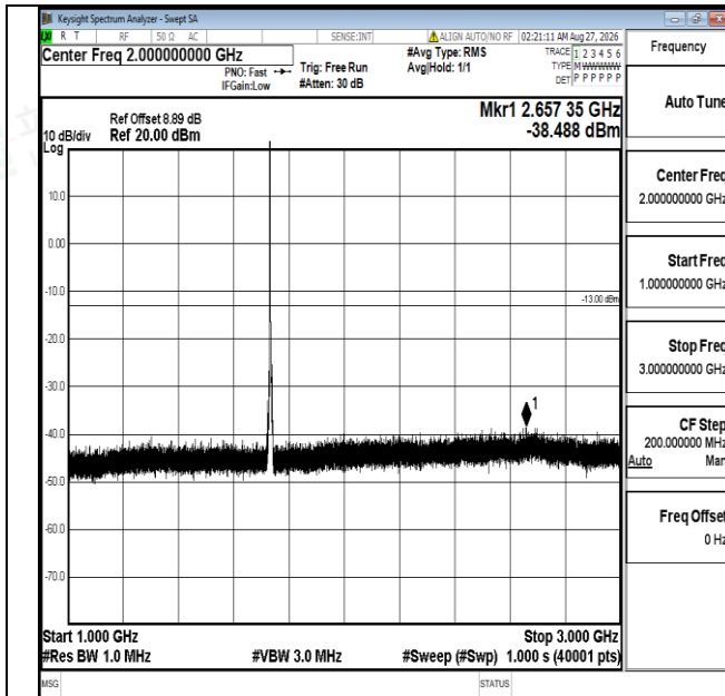
Band4-5MHz-16QAM-20175-1RB#0-1000~3000-PASS
