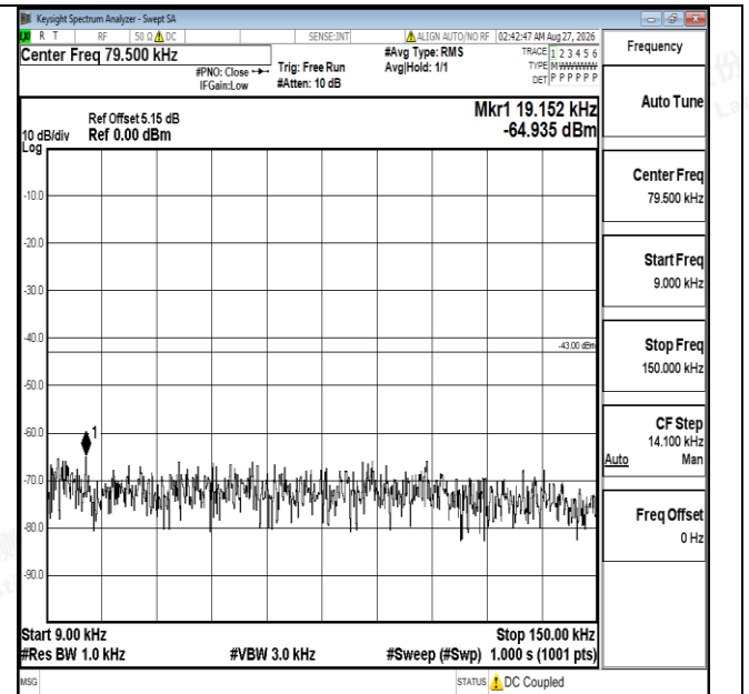
Band4-10MHz-16QAM-20000-1RB#0-0.009~0.15-PASS
