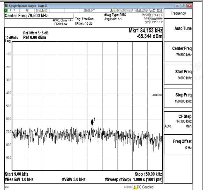
Band4-5MHz-16QAM-19975-1RB#0-0.009~0.15-PASS
