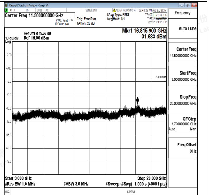
Band4-10MHz-16QAM-20000-1RB#0-3000~20000-PASS
