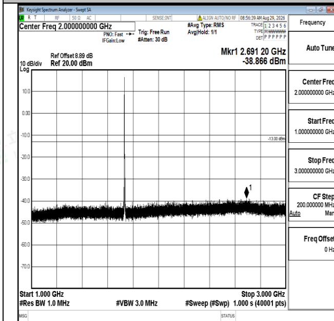
Band4-3MHz-16QAM-20175-1RB#0-1000~3000-PASS
