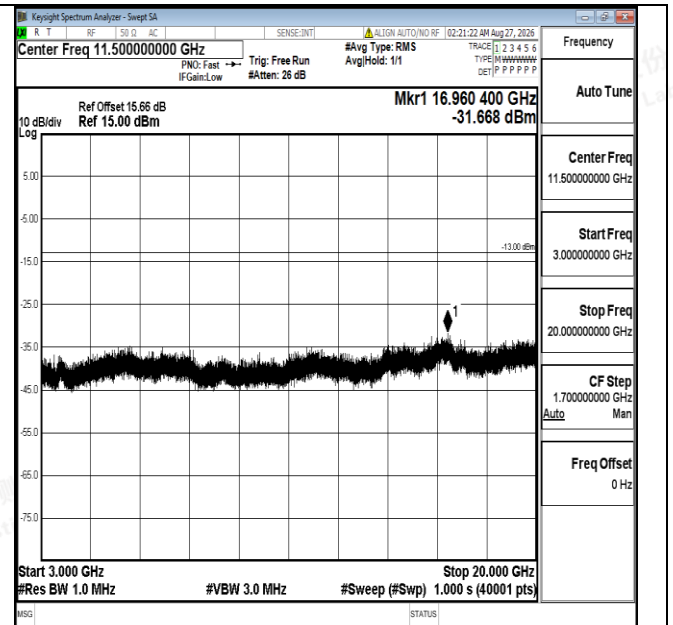
Band4-5MHz-16QAM-20175-1RB#0-3000~20000-PASS
