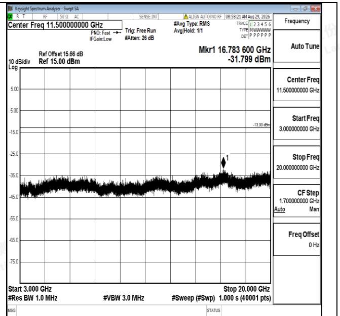
Band4-3MHz-16QAM-20385-1RB#0-3000~20000-PASS
