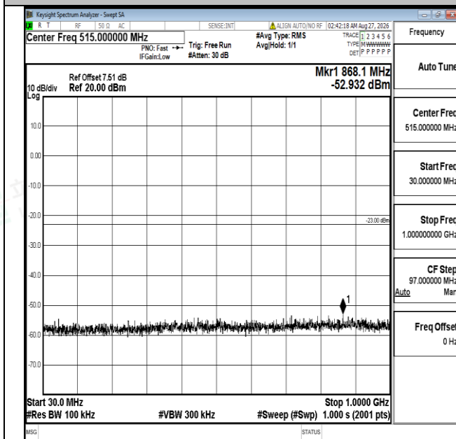
Band4-10MHz-QPSK-20000-1RB#0-30~1000-PASS
