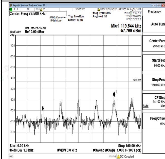
Band4-3MHz-QPSK-20175-1RB#0-0.009-0.15-PASS
