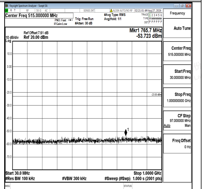
Band4-5MHz-16QAM-20175-1RB#0-30~1000-PASS
