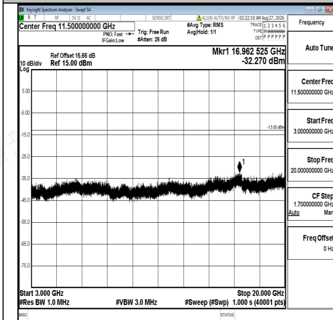
Band4-5MHz-QPSK-20375-1RB#0-3000~20000-PASS
