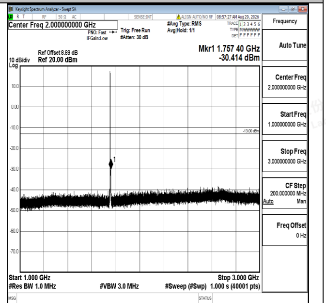
Band4-3MHz-QPSK-20385-1RB#0-1000~3000-PASS
