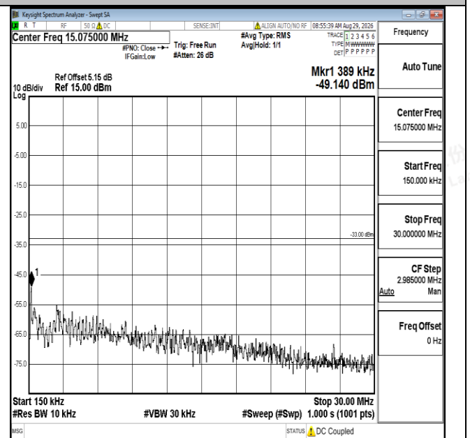
Band4-3MHz-QPSK-20175-1RB#0-0.15-30-PASS
