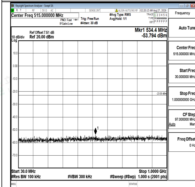
Band4-5MHz-QPSK-20175-1RB#0-30~1000-PASS
