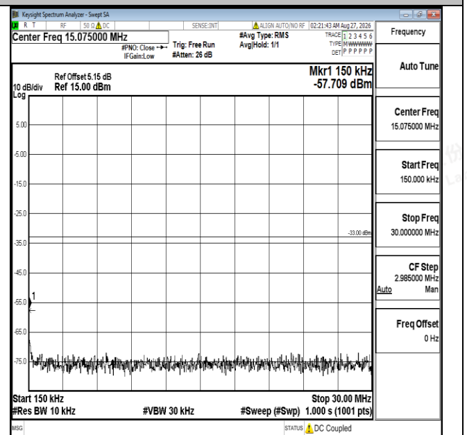
Band4-5MHz-QPSK-20375-1RB#0-0.15~30-PASS
