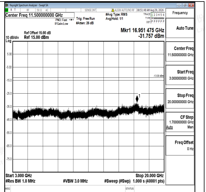
Band4-1.4MHz-16QAM-20175-1RB#0-3000~20000-PASS
