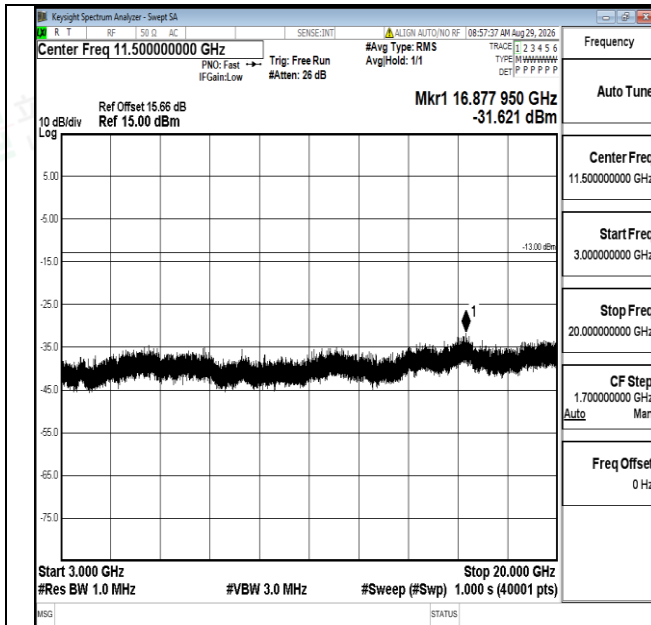
Band4-3MHz-QPSK-20385-1RB#0-3000~20000-PASS
