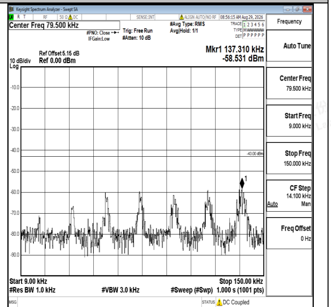
Band4-3MHz-16QAM-20175-1RB#0-0.009~0.15-PASS
