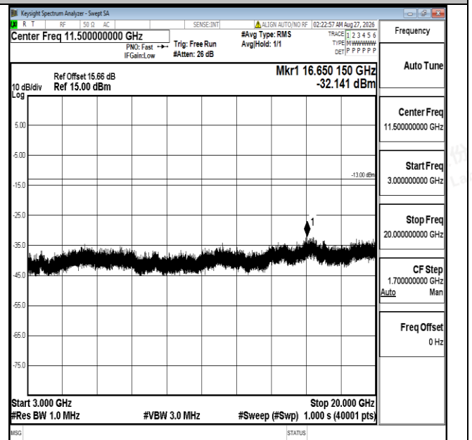
Band4-5MHz-16QAM-20375-1RB#0-3000~20000-PASS
