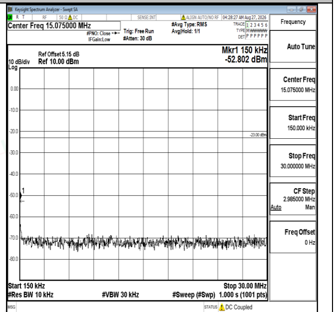
Band5-3MHz-QPSK-20635-1RB#0-0.15~30-PASS
