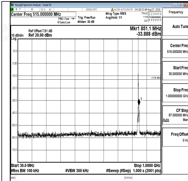
Band5-3MHz-QPSK-20635-1RB#0-30~1000-PASS
