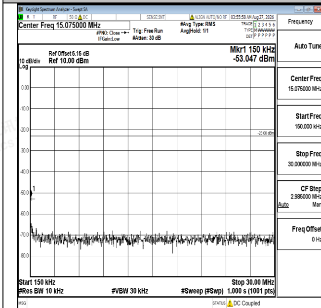
Band5-1.4MHz-16QAM-20643-1RB#0-0.15~30-PASS
