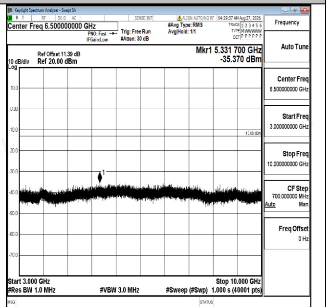
Band5-3MHz-16QAM-20635-1RB#0-3000~10000-PASS
