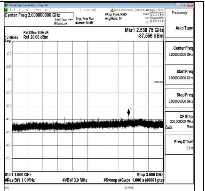
Band5-3MHz-QPSK-20635-1RB#0-1000~3000-PASS
