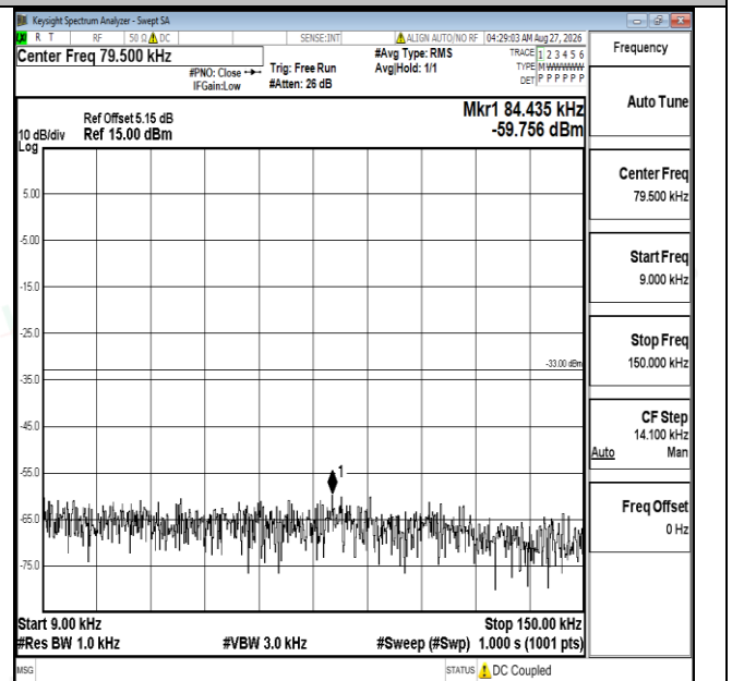
Band5-3MHz-16QAM-20635-1RB#0-0.009~0.15-PASS
