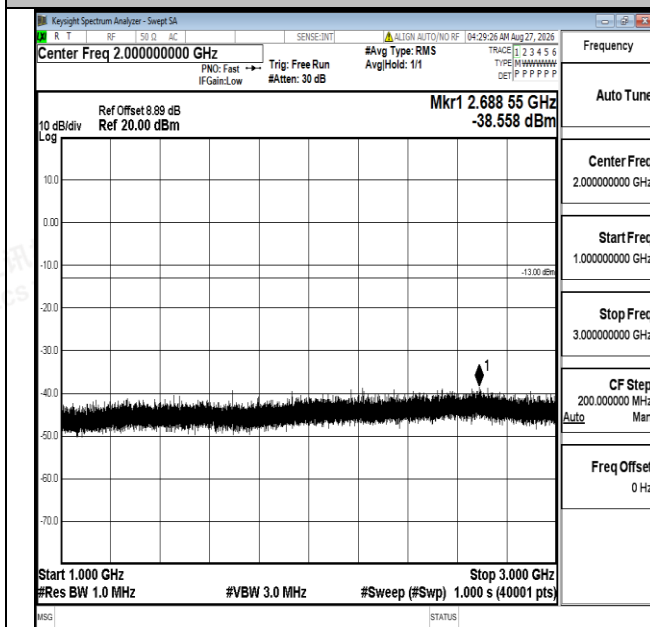
Band5-3MHz-16QAM-20635-1RB#0-1000~3000-PASS
