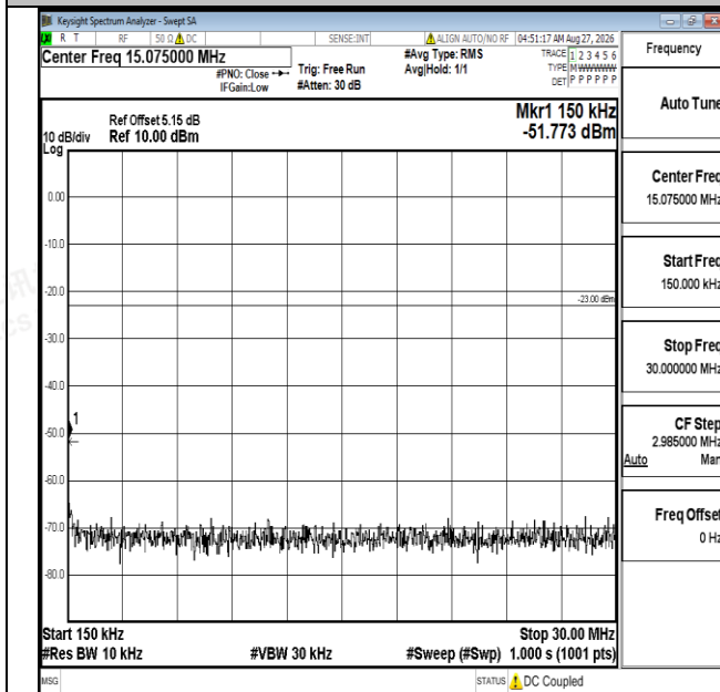
Band5-5MHz-16QAM-20425-1RB#0-0.15~30-PASS
