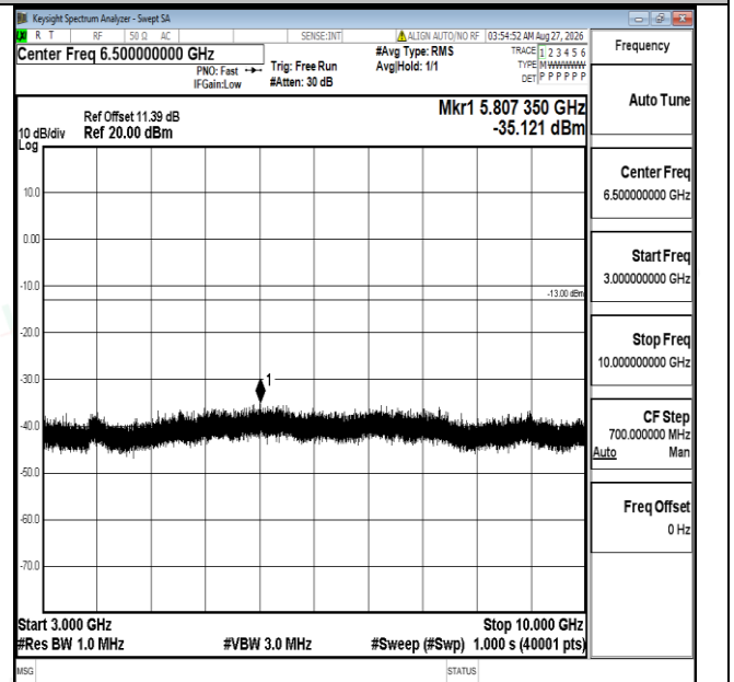
Band5-1.4MHz-16QAM-20525-1RB#0-3000~10000-PASS
