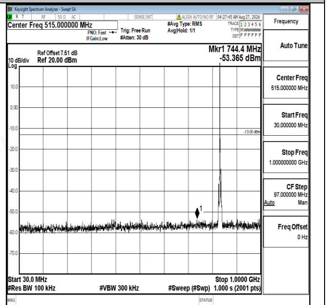
Band5-3MHz-16QAM-20525-1RB#0-30~1000-PASS
