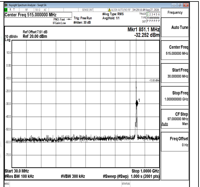
Band5-3MHz-16QAM-20635-1RB#0-30~1000-PASS
