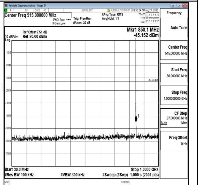
Band5-1.4MHz-16QAM-20643-1RB#0-30~1000-PASS
