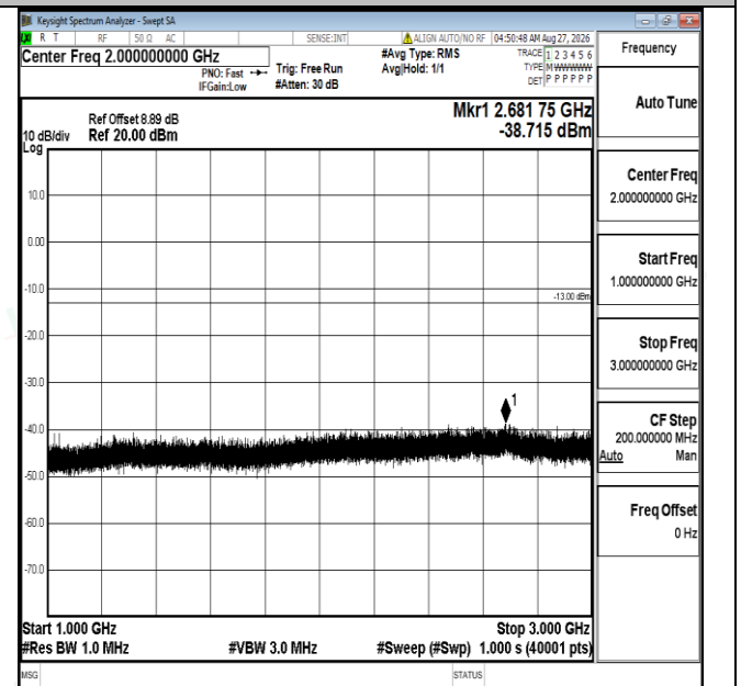
Band5-5MHz-QPSK-20425-1RB#0-1000~3000-PASS
