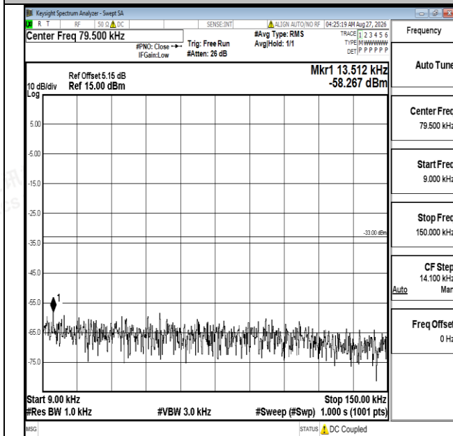
Band5-3MHz-QPSK-20415-1RB#0-0.009~0.15-PASS
