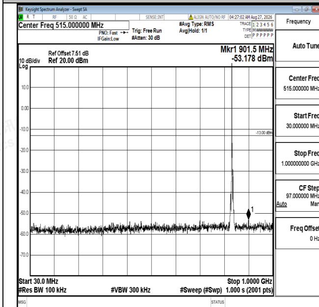
Band5-3MHz-QPSK-20525-1RB#0-30~1000-PASS
