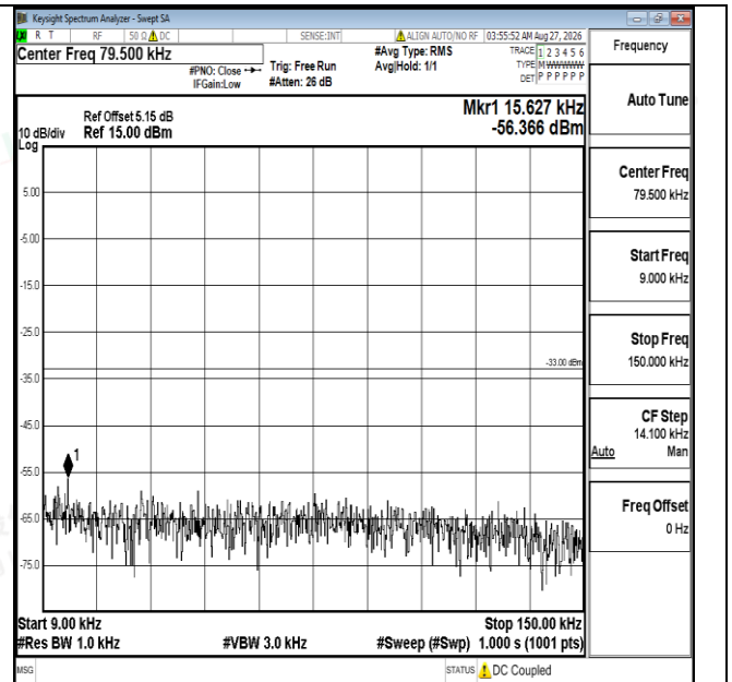
Band5-1.4MHz-16QAM-20643-1RB#0-0.009~0.15-PASS
