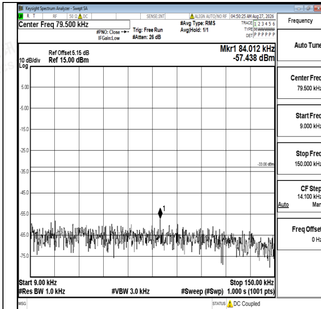
Band5-5MHz-QPSK-20425-1RB#0-0.009~0.15-PASS
