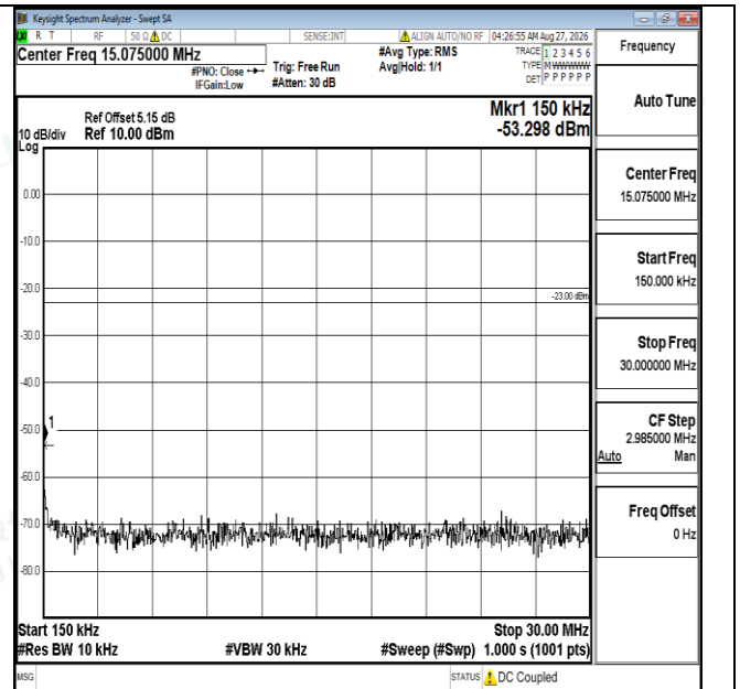
Band5-3MHz-QPSK-20525-1RB#0-0.15~30-PASS
