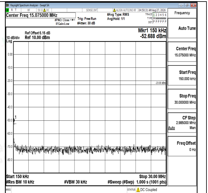
Band5-5MHz-QPSK-20425-1RB#0-0.15~30-PASS
