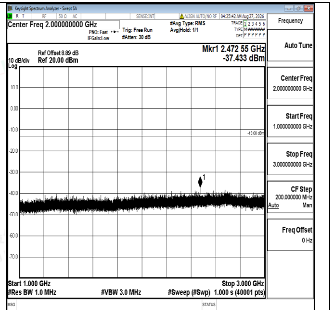
Band5-3MHz-QPSK-20415-1RB#0-1000~3000-PASS
