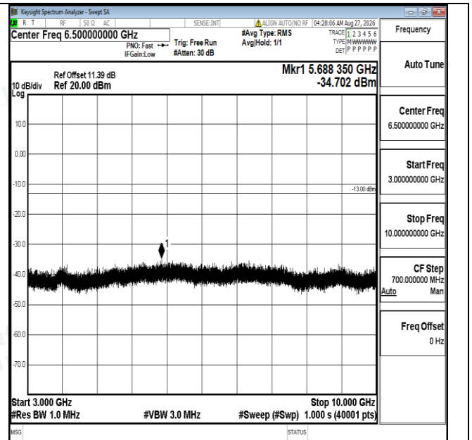
Band5-3MHz-16QAM-20525-1RB#0-3000~10000-PASS
