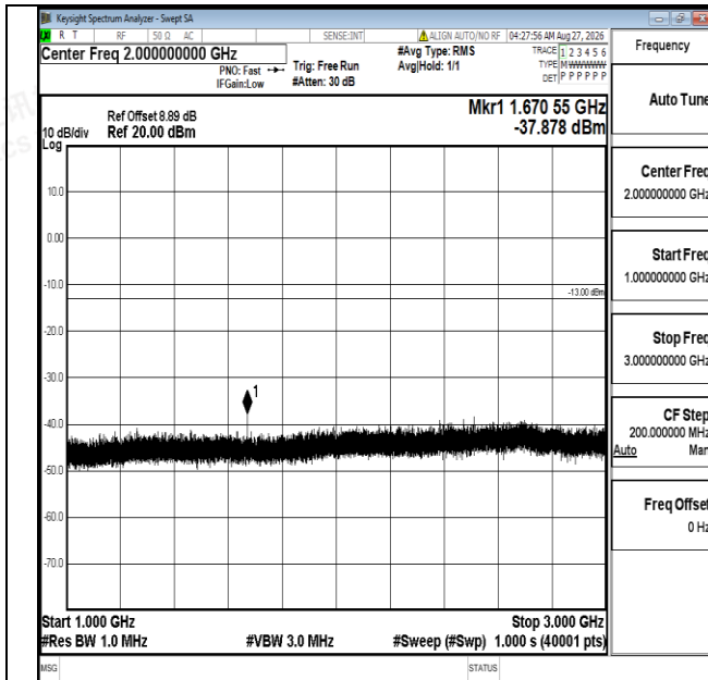
Band5-3MHz-16QAM-20525-1RB#0-1000~3000-PASS
