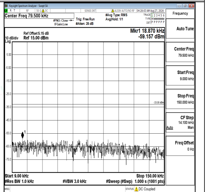
Band5-3MHz-16QAM-20415-1RB#0-0.009~0.15-PASS
