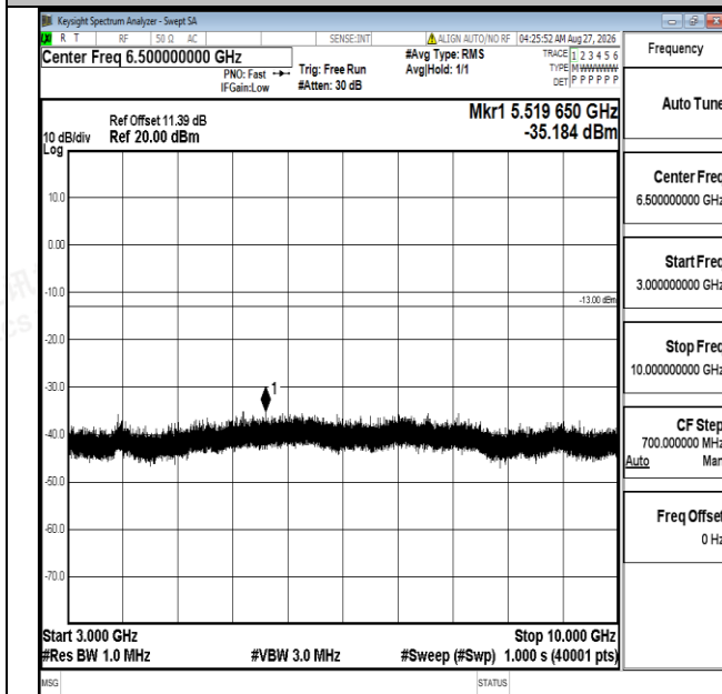
Band5-3MHz-QPSK-20415-1RB#0-3000~10000-PASS
