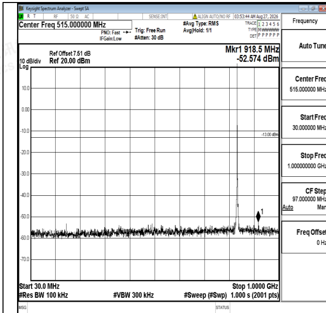
Band5-1.4MHz-QPSK-20525-1RB#0-30~1000-PASS
