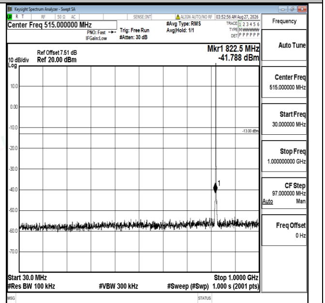
Band5-1.4MHz-16QAM-20407-1RB#0-30~1000-PASS
