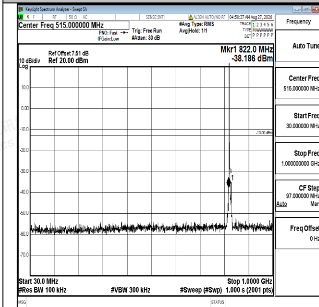
Band5-5MHz-QPSK-20425-1RB#0-30~1000-PASS
