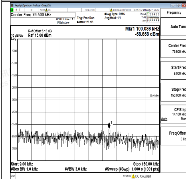
Band5-1.4MHz-QPSK-20525-1RB#0-0.009~0.15-PASS
