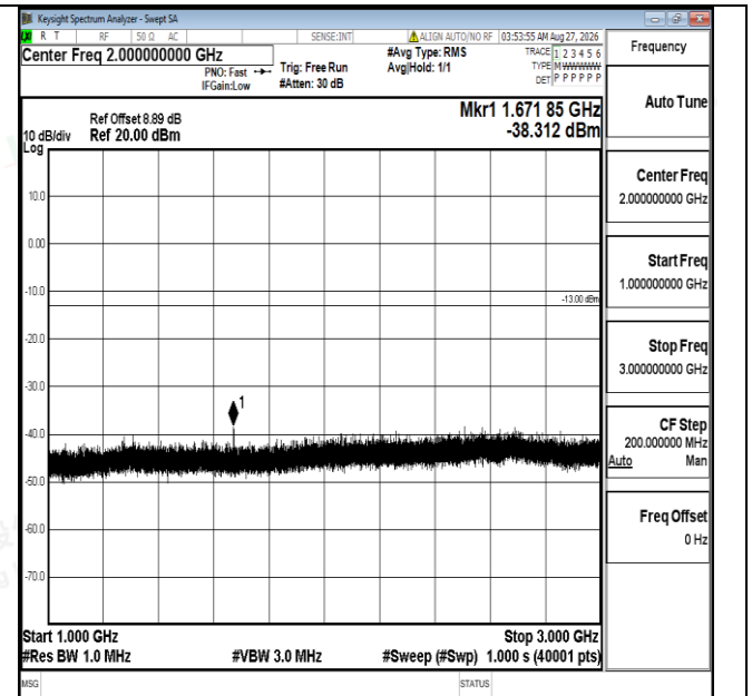
Band5-1.4MHz-QPSK-20525-1RB#0-1000~3000-PASS
