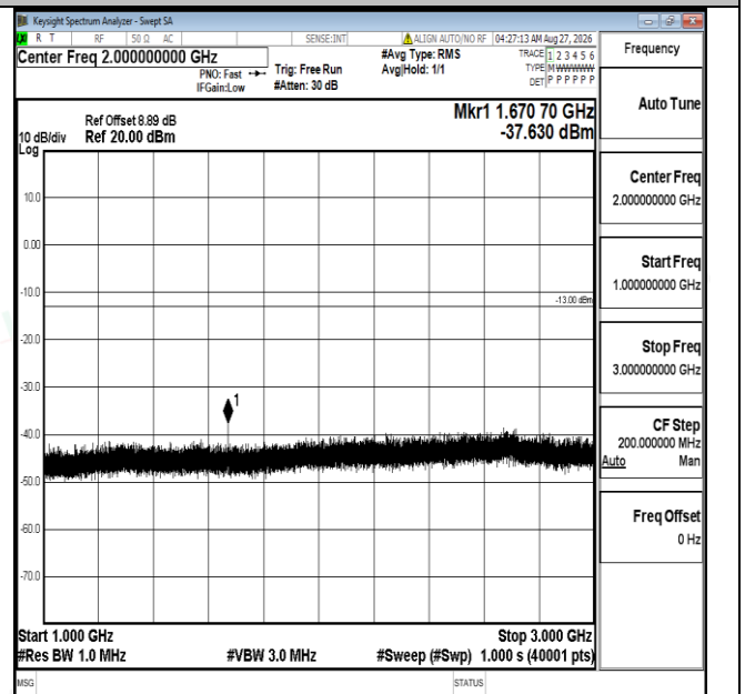
Band5-3MHz-QPSK-20525-1RB#0-1000~3000-PASS
