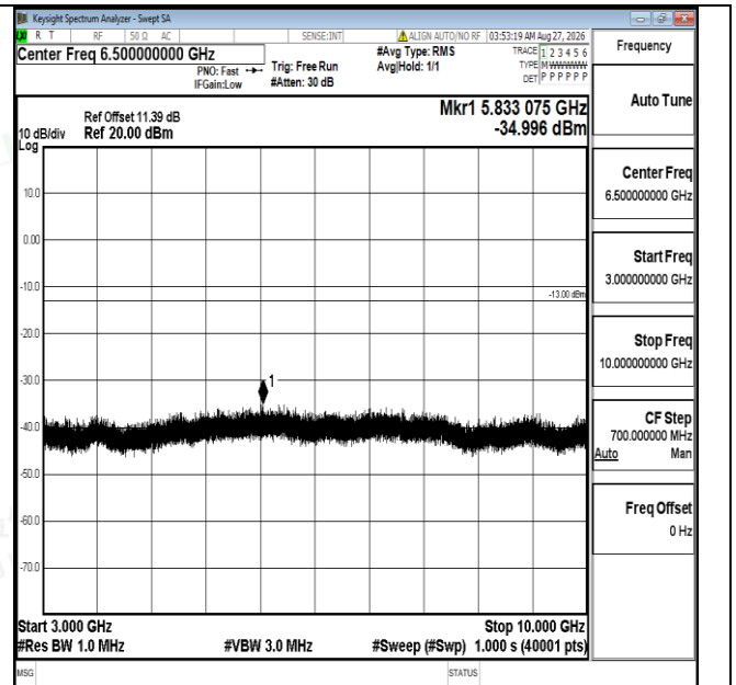
Band5-1.4MHz-16QAM-20407-1RB#0-3000~10000-PASS
