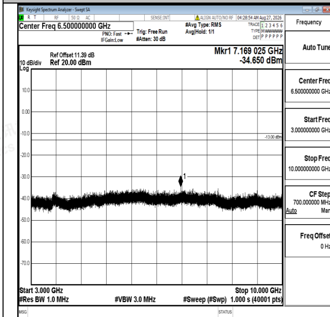
Band5-3MHz-QPSK-20635-1RB#0-3000~10000-PASS
