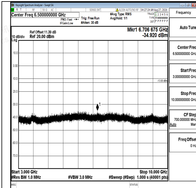
Band5-3MHz-QPSK-20525-1RB#0-3000~10000-PASS
