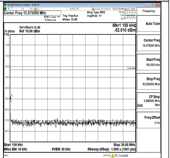
Band5-1.4MHz-QPSK-20525-1RB#0-0.15~30-PASS
