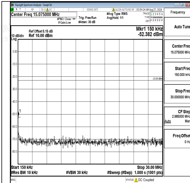
Band5-1.4MHz-16QAM-20525-1RB#0-0.15~30-PASS
