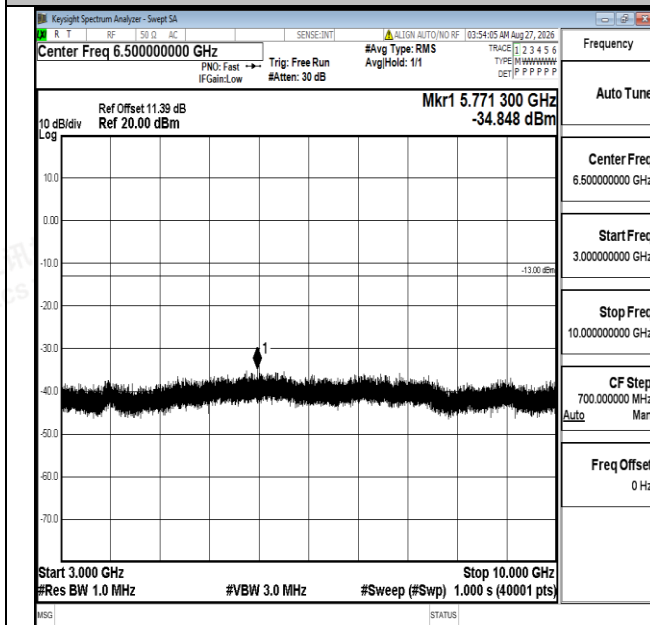
Band5-1.4MHz-QPSK-20525-1RB#0-3000~10000-PASS
