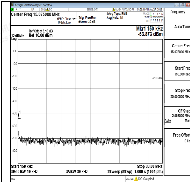
Band5-3MHz-16QAM-20415-1RB#0-0.15~30-PASS
