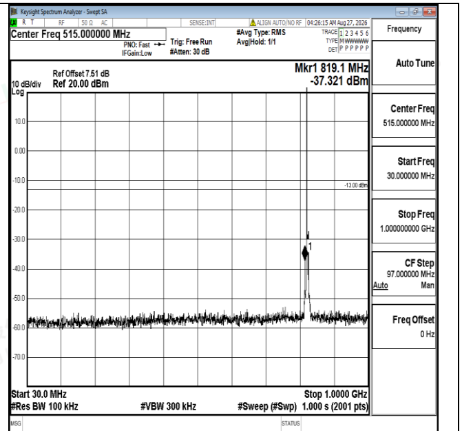
Band5-3MHz-16QAM-20415-1RB#0-30~1000-PASS
