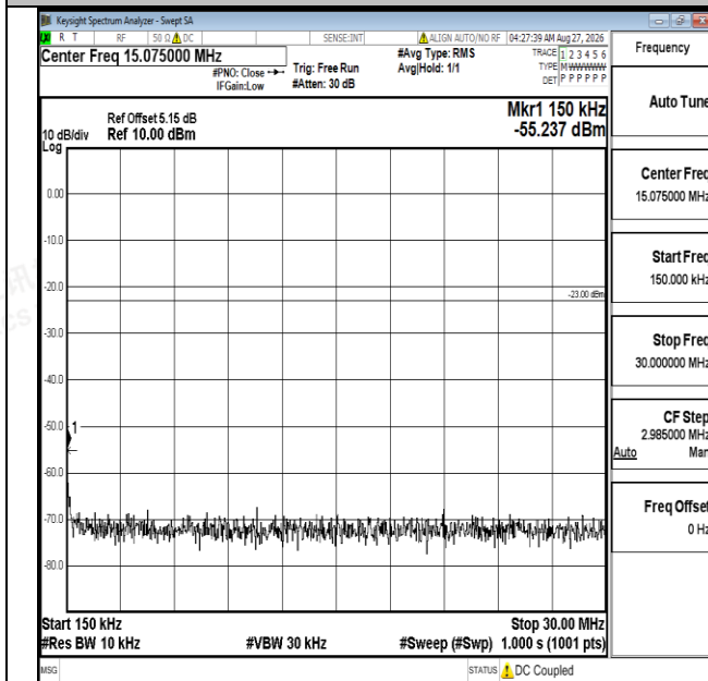
Band5-3MHz-16QAM-20525-1RB#0-0.15~30-PASS
