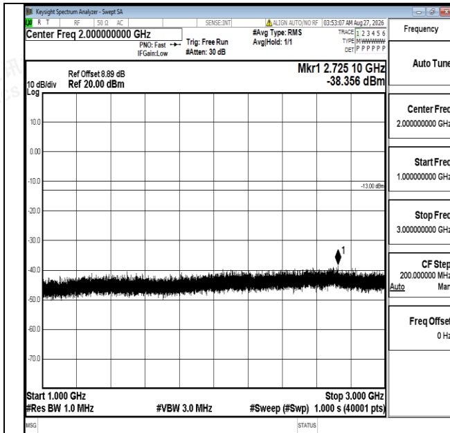
Band5-1.4MHz-16QAM-20407-1RB#0-1000~3000-PASS
