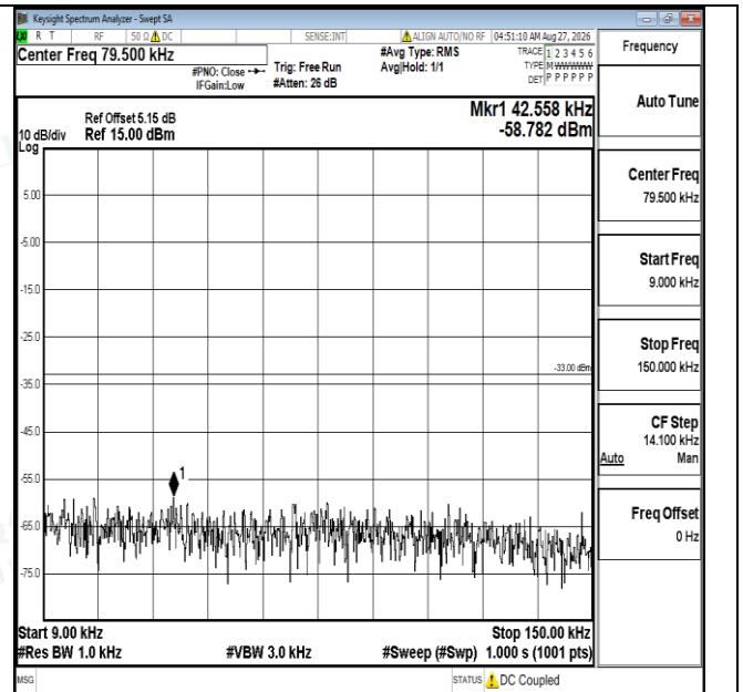
Band5-5MHz-16QAM-20425-1RB#0-0.009~0.15-PASS
