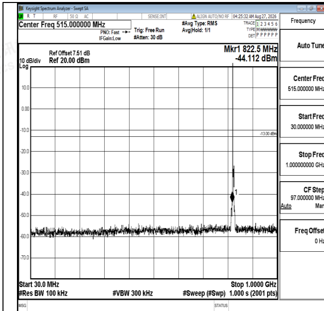
Band5-3MHz-QPSK-20415-1RB#0-30~1000-PASS
