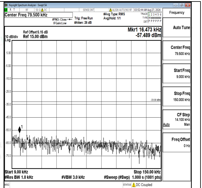
Band5-1.4MHz-16QAM-20407-1RB#0-0.009~0.15-PASS
