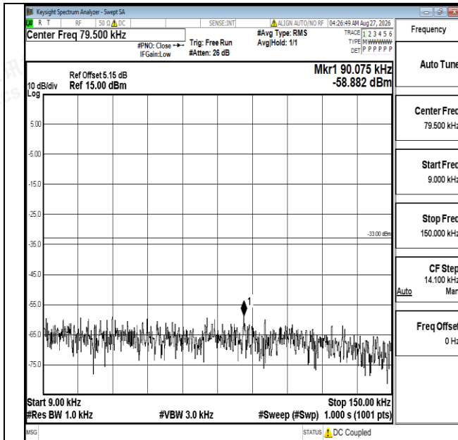
Band5-3MHz-QPSK-20525-1RB#0-0.009~0.15-PASS
