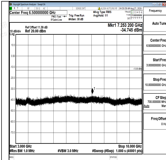
Band5-5MHz-QPSK-20425-1RB#0-3000~10000-PASS
