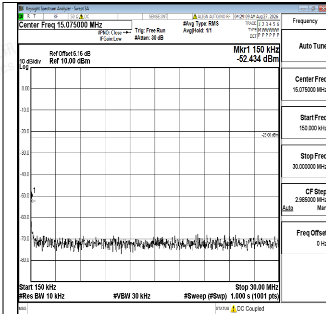
Band5-3MHz-16QAM-20635-1RB#0-0.15~30-PASS
