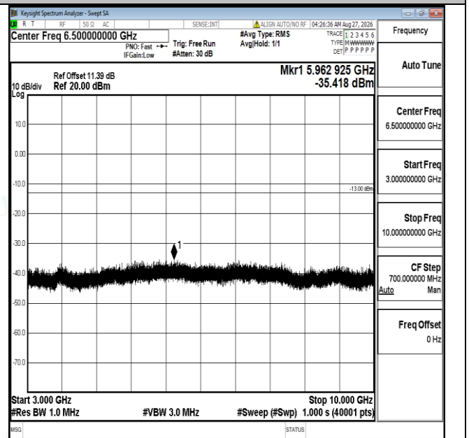
Band5-3MHz-16QAM-20415-1RB#0-3000~10000-PASS
