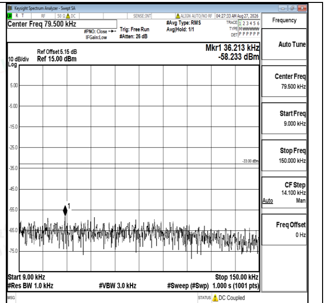
Band5-3MHz-16QAM-20525-1RB#0-0.009~0.15-PASS
