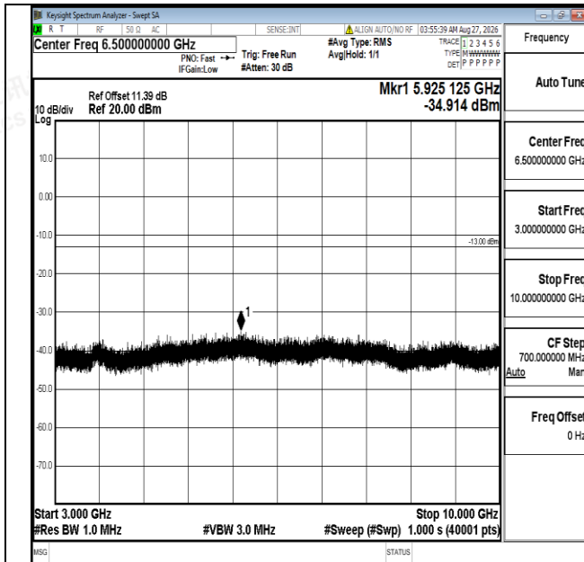
Band5-1.4MHz-QPSK-20643-1RB#0-3000~10000-PASS
