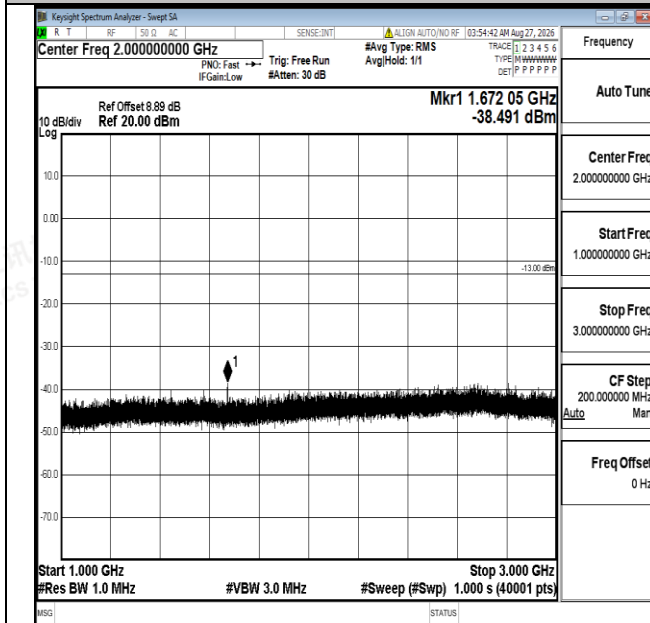
Band5-1.4MHz-16QAM-20525-1RB#0-1000~3000-PASS
