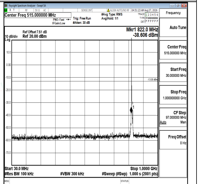
Band5-5MHz-16QAM-20425-1RB#0-30~1000-PASS
