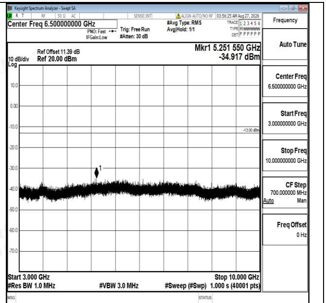
Band5-1.4MHz-16QAM-20643-1RB#0-3000~10000-PASS
