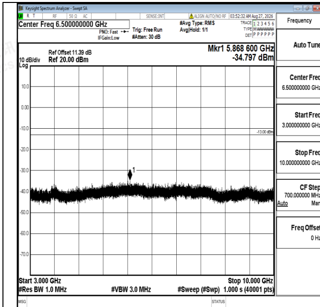
Band5-1.4MHz-QPSK-20407-1RB#0-3000~10000-PASS
