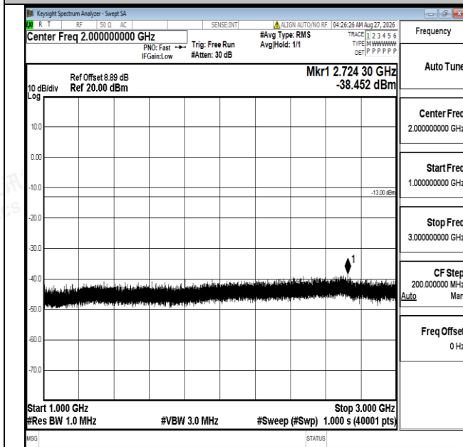
Band5-3MHz-16QAM-20415-1RB#0-1000~3000-PASS
