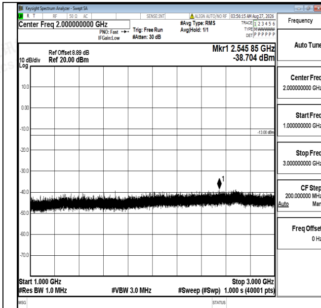
Band5-1.4MHz-16QAM-20643-1RB#0-1000~3000-PASS
