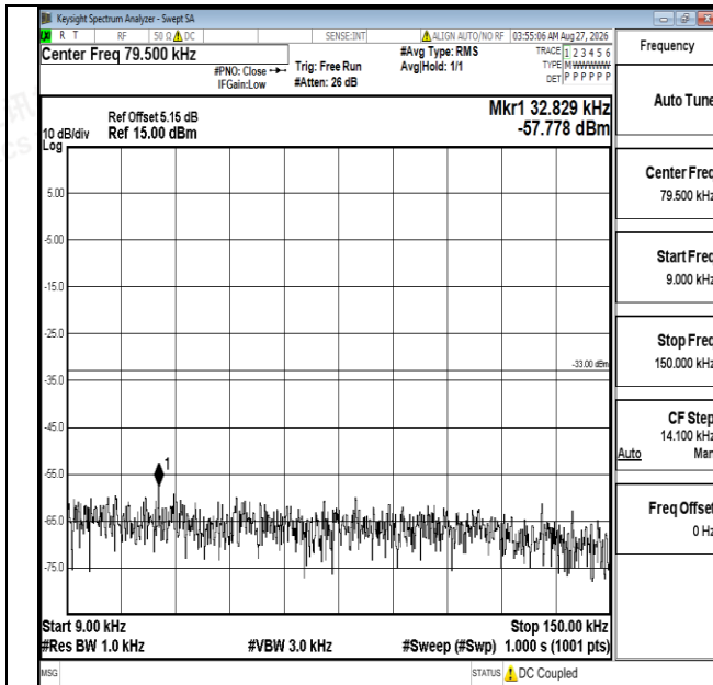
Band5-1.4MHz-QPSK-20643-1RB#0-0.009~0.15-PASS
