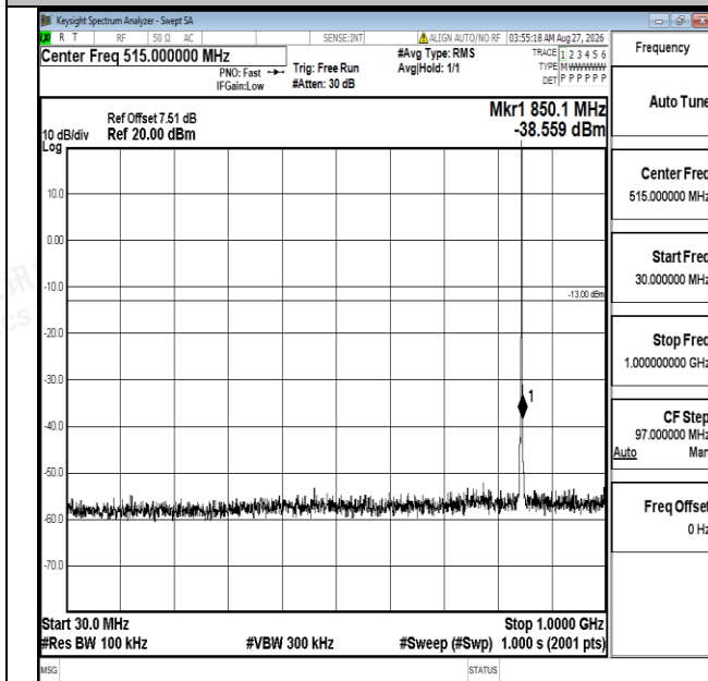
Band5-1.4MHz-QPSK-20643-1RB#0-30~1000-PASS
