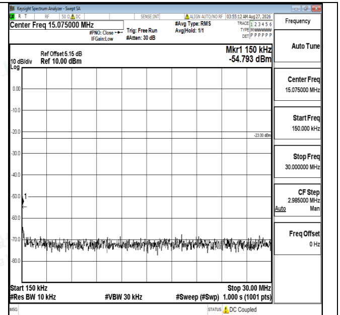
Band5-1.4MHz-QPSK-20643-1RB#0-0.15~30-PASS
