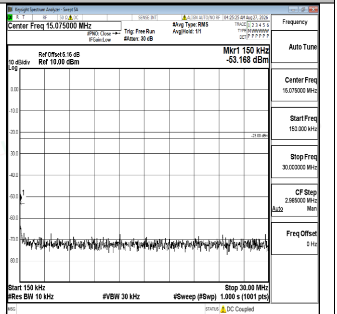
Band5-3MHz-QPSK-20415-1RB#0-0.15~30-PASS
