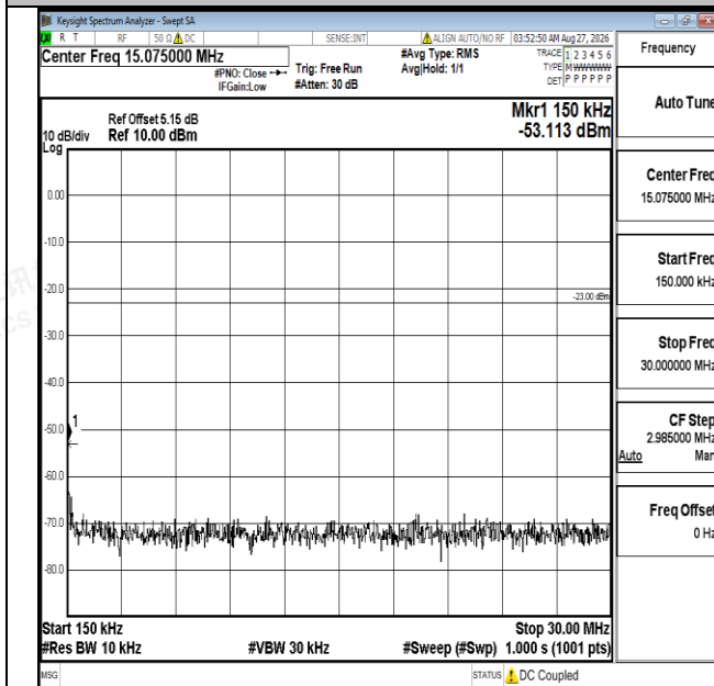
Band5-1.4MHz-16QAM-20407-1RB#0-0.15~30-PASS
