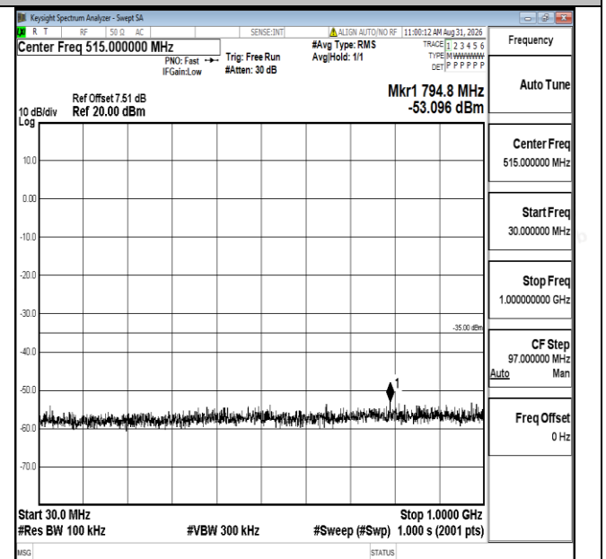
Band7-15MHz-16QAM-20825-1RB#0-30~1000-PASS
