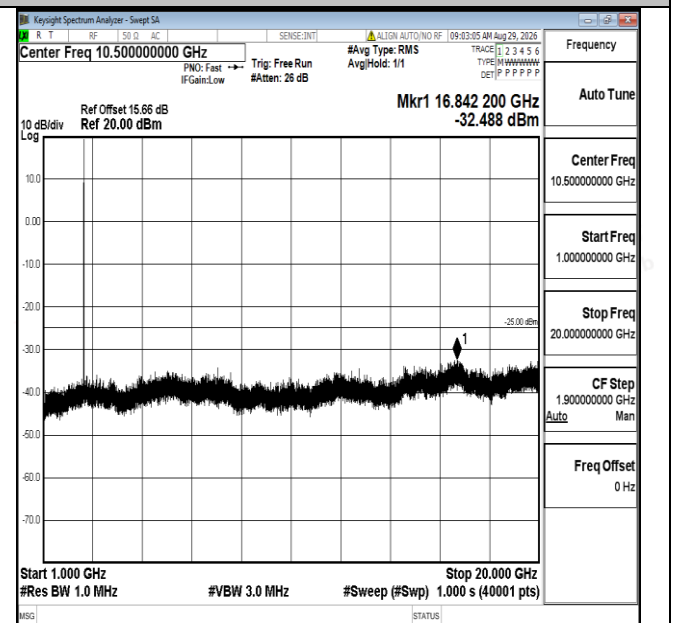
Band7-5MHz-QPSK-21425-1RB#0-1000~20000-PASS
