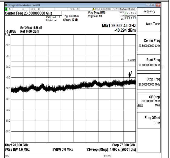
Band7-10MHz-16QAM-20800-1RB#0-20000~27000-PASS
