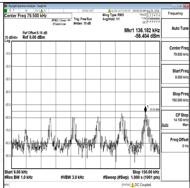
Band7-5MHz-16QAM-20775-1RB#0-0.009~0.15-PASS
