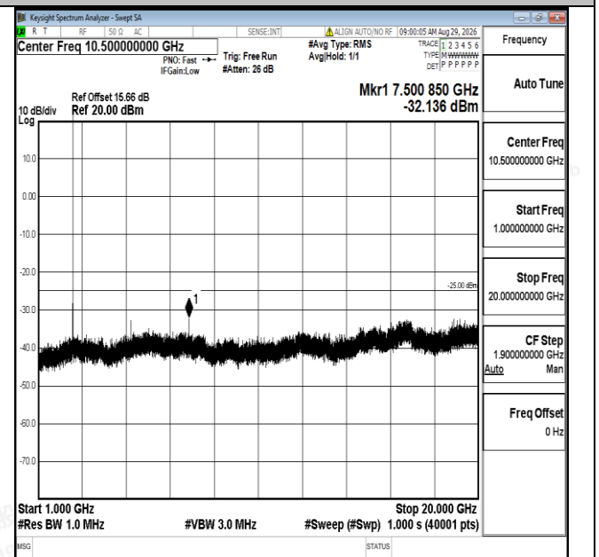
Band7-5MHz-QPSK-20775-1RB#0-1000~20000-PASS
