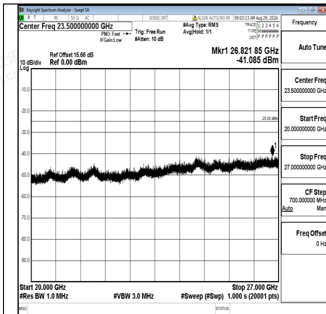
Band7-5MHz-QPSK-21425-1RB#0-20000~27000-PASS
