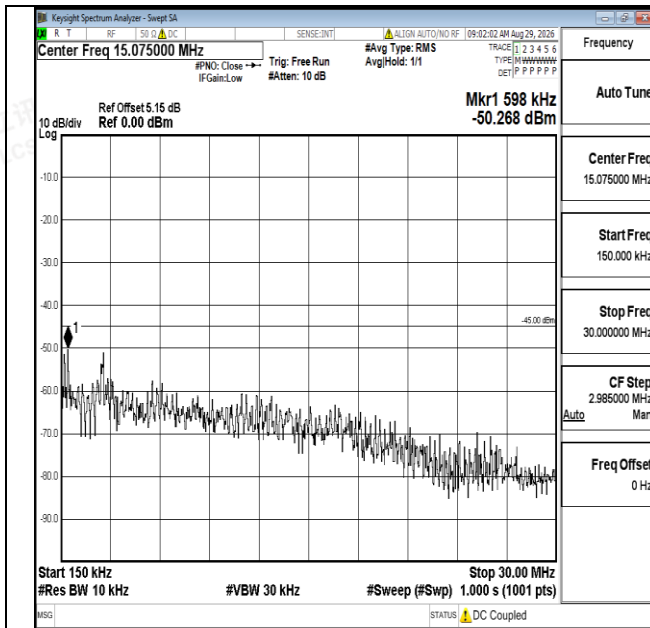
Band7-5MHz-16QAM-21100-1RB#0-0.15~30-PASS
