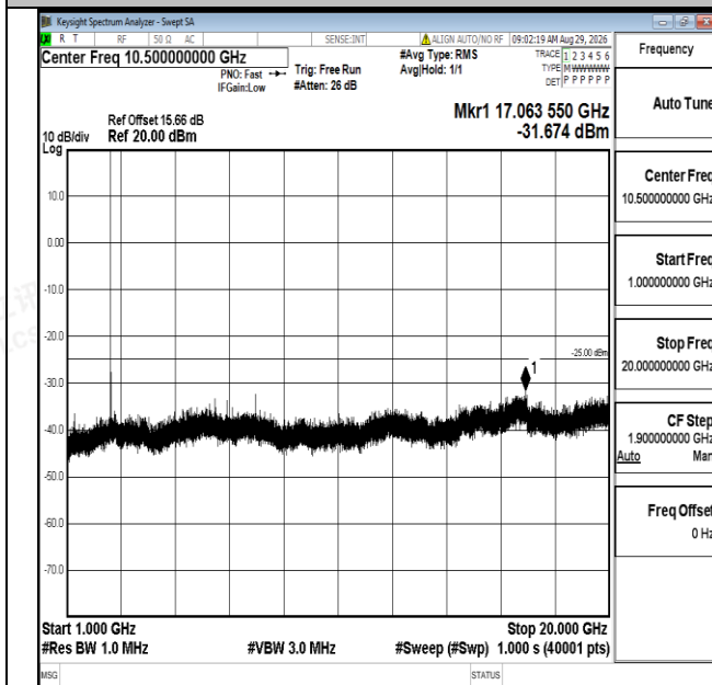
Band7-5MHz-16QAM-21100-1RB#0-1000~20000-PASS
