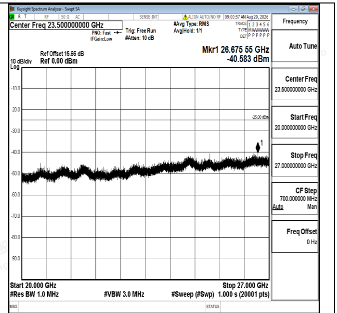
Band7-5MHz-16QAM-20775-1RB#0-20000~27000-PASS
