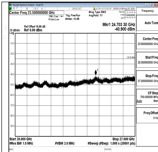
Band7-5MHz-QPSK-20775-1RB#0-20000~27000-PASS
