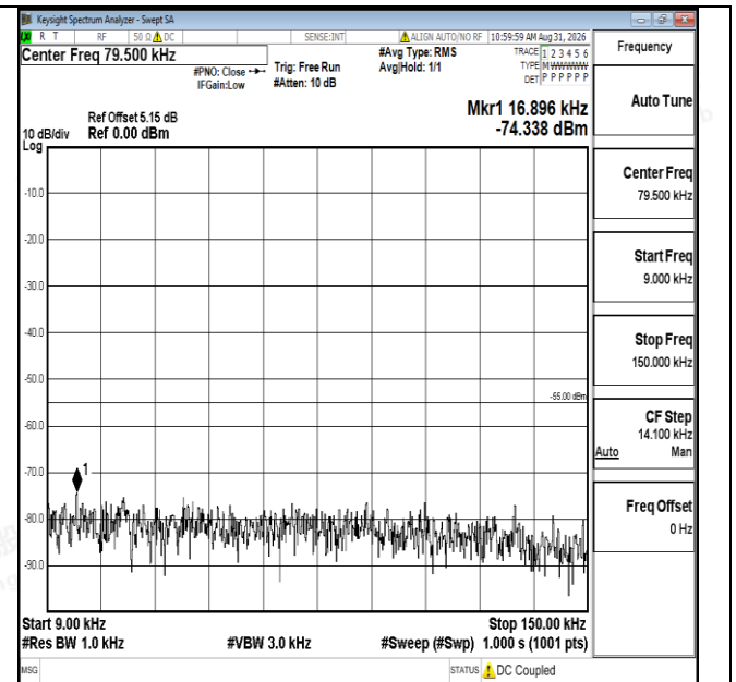
Band7-15MHz-16QAM-20825-1RB#0-0.009~0.15-PASS
