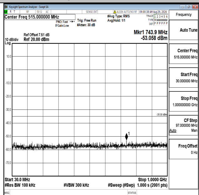
Band7-5MHz-16QAM-20775-1RB#0-30~1000-PASS
