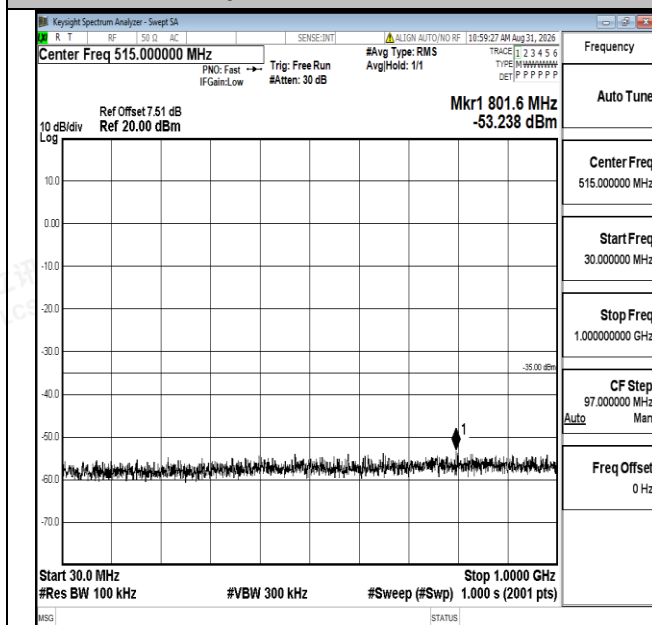
Band7-15MHz-QPSK-20825-1RB#0-30~1000-PASS
