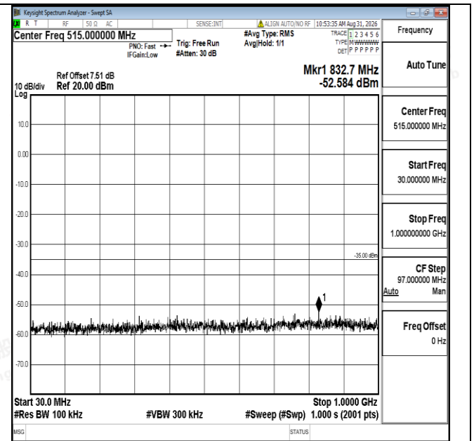
Band7-10MHz-16QAM-20800-1RB#0-30~1000-PASS
