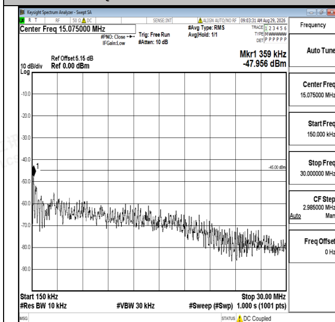
Band7-5MHz-16QAM-21425-1RB#0-0.15~30-PASS
