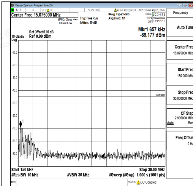
Band7-10MHz-16QAM-21400-1RB#0-0.15~30-PASS
