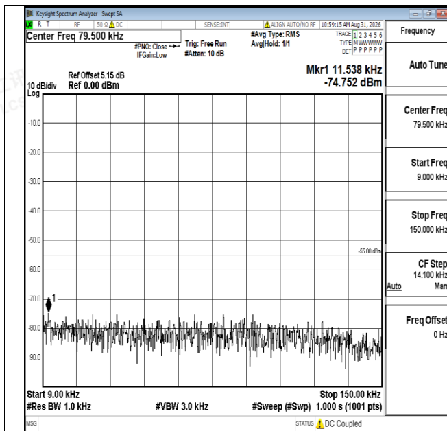
Band7-15MHz-QPSK-20825-1RB#0-0.009~0.15-PASS
