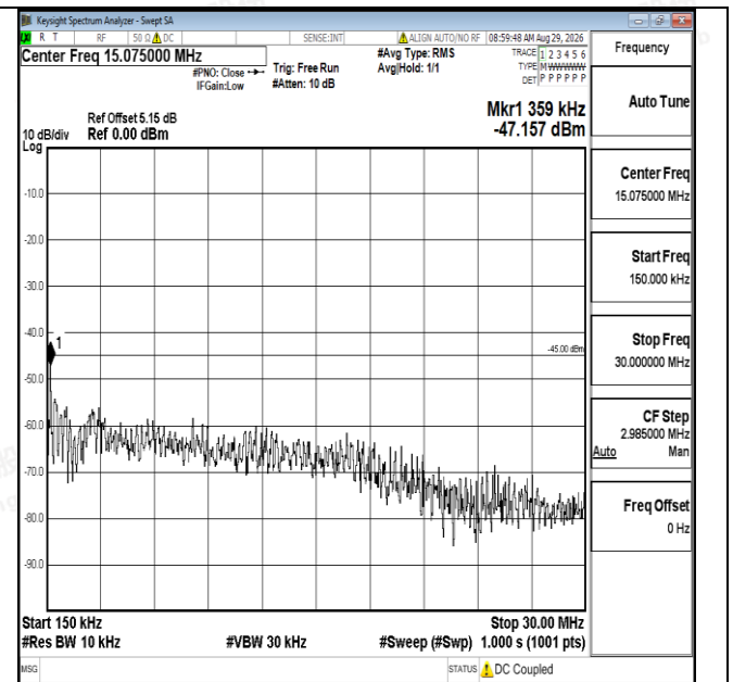
Band7-5MHz-QPSK-20775-1RB#0-0.15~30-PASS
