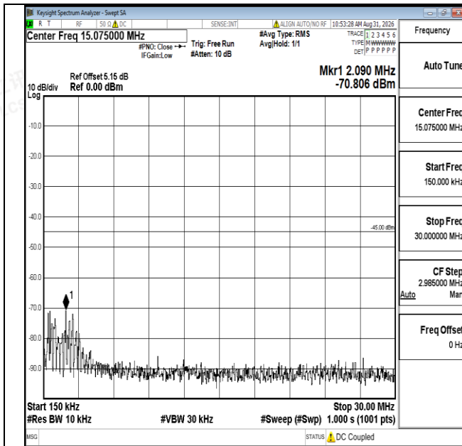
Band7-10MHz-16QAM-20800-1RB#0-0.15~30-PASS
