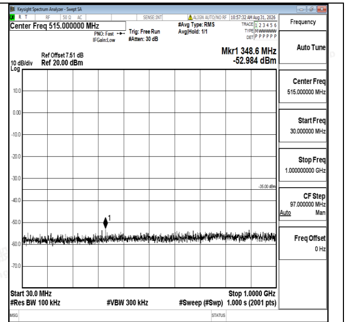
Band7-10MHz-16QAM-21400-1RB#0-30~1000-PASS
