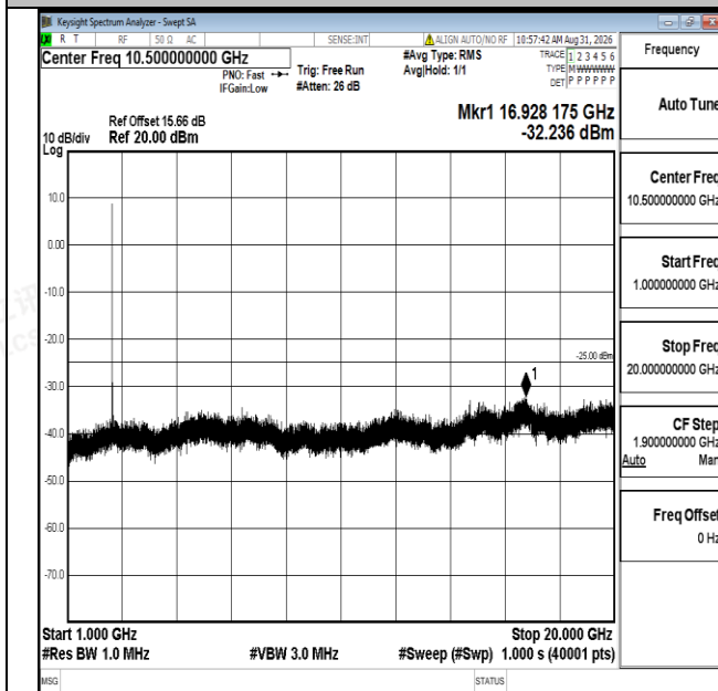
Band7-10MHz-16QAM-21400-1RB#0-1000~20000-PASS
