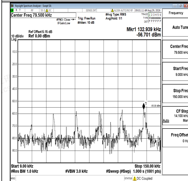
Band7-5MHz-QPSK-21100-1RB#0-0.009~0.15-PASS
