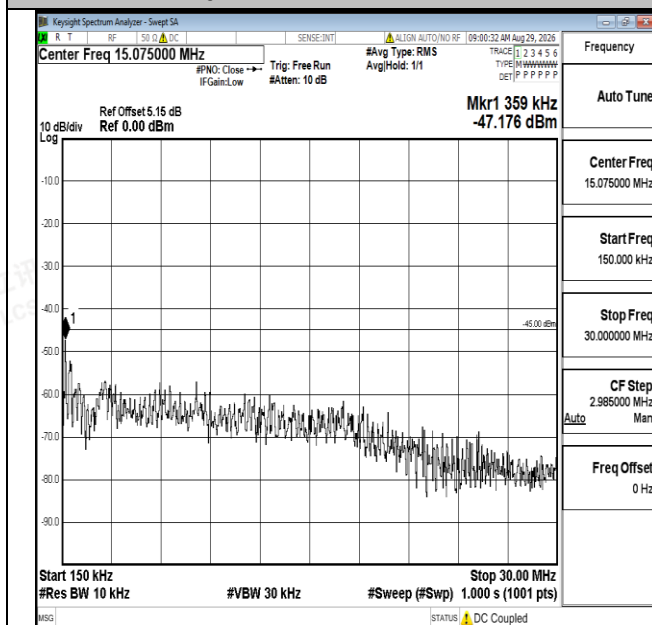
Band7-5MHz-16QAM-20775-1RB#0-0.15~30-PASS
