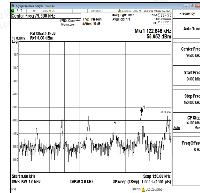
Band7-5MHz-QPSK-20775-1RB#0-0.009~0.15-PASS
