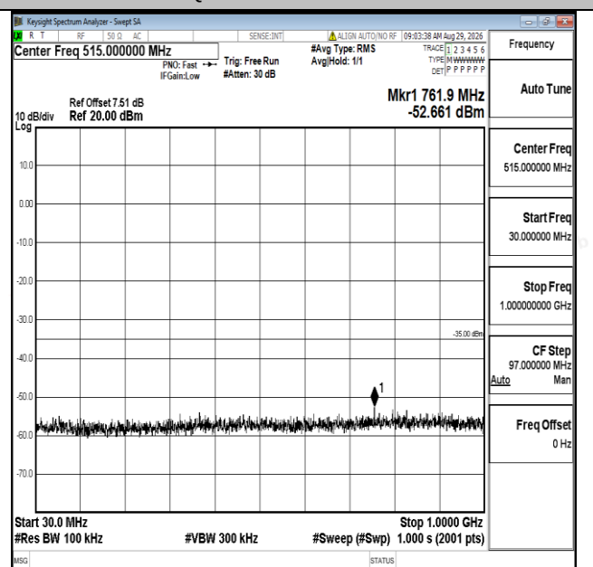
Band7-5MHz-16QAM-21425-1RB#0-30~1000-PASS
