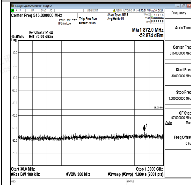
Band7-5MHz-QPSK-20775-1RB#0-30~1000-PASS
