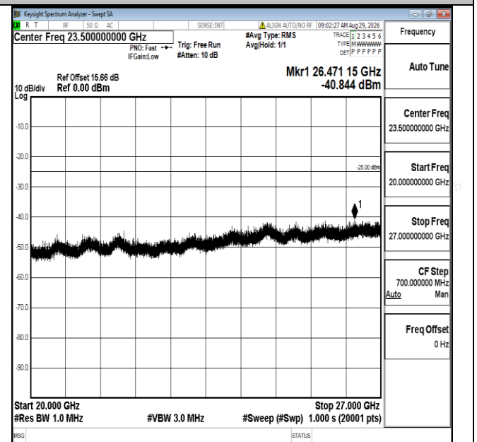
Band7-5MHz-16QAM-21100-1RB#0-20000~27000-PASS
