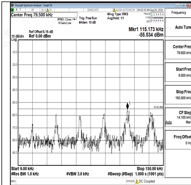
Band7-5MHz-QPSK-21425-1RB#0-0.009~0.15-PASS
