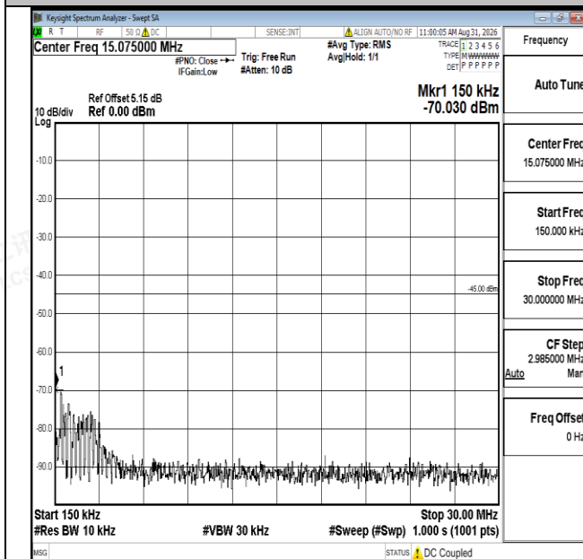
Band7-15MHz-16QAM-20825-1RB#0-0.15~30-PASS
