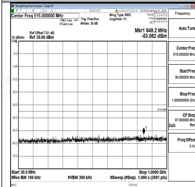
Band7-10MHz-QPSK-21100-1RB#0-30~1000-PASS
