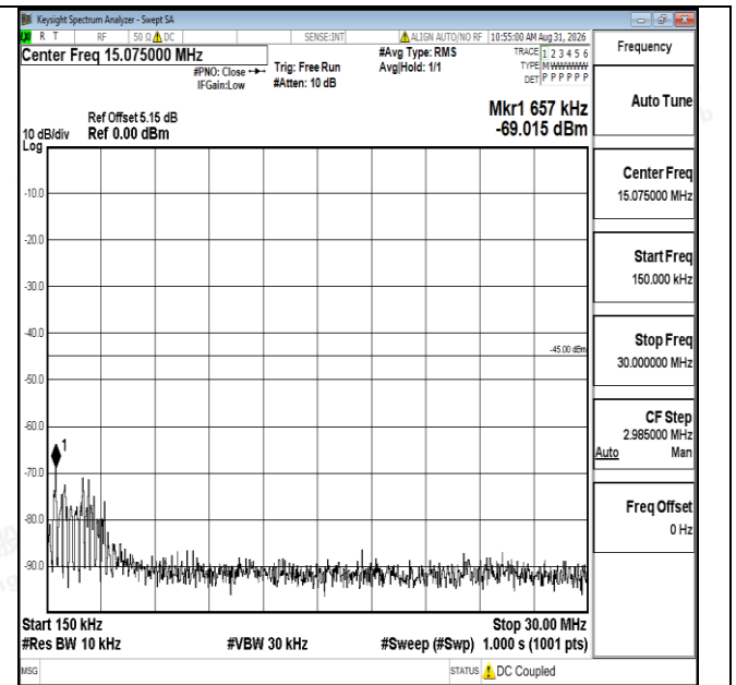
Band7-10MHz-QPSK-21100-1RB#0-0.15~30-PASS
