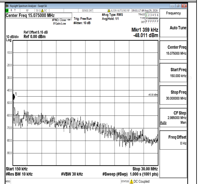
Band7-5MHz-QPSK-21100-1RB#0-0.15~30-PASS
