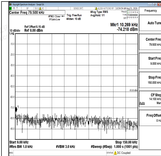
Band7-10MHz-QPSK-21100-1RB#0-0.009~0.15-PASS
