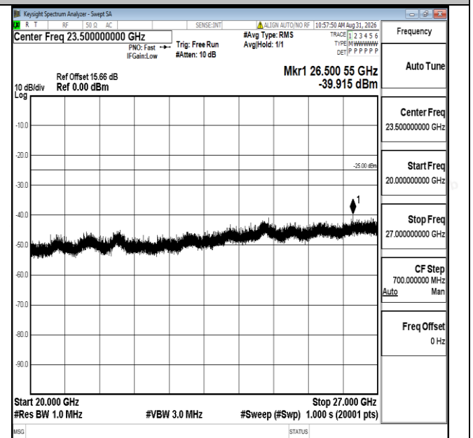
Band7-10MHz-16QAM-21400-1RB#0-20000~27000-PASS
