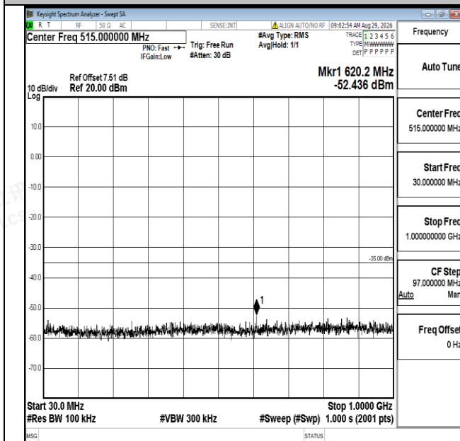
Band7-5MHz-QPSK-21425-1RB#0-30~1000-PASS
