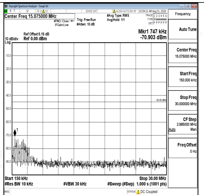
Band7-15MHz-QPSK-20825-1RB#0-0.15~30-PASS
