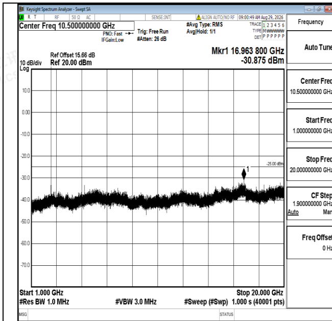
Band7-5MHz-16QAM-20775-1RB#0-1000~20000-PASS
