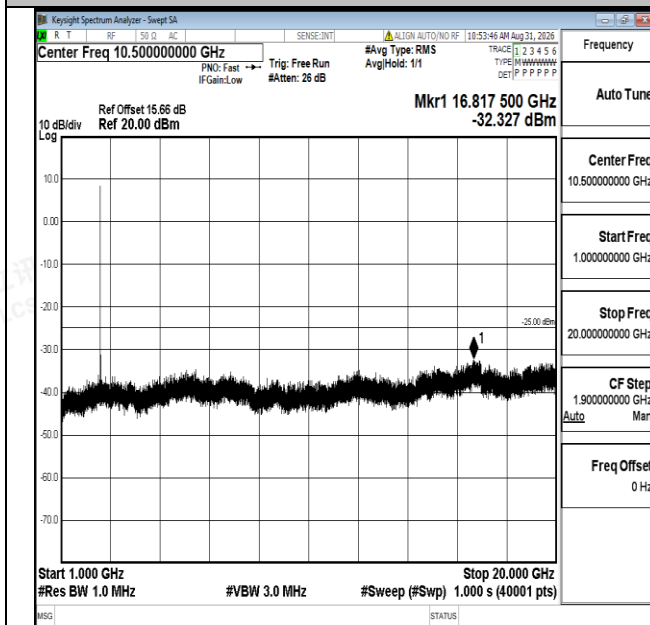
Band7-10MHz-16QAM-20800-1RB#0-1000~20000-PASS
