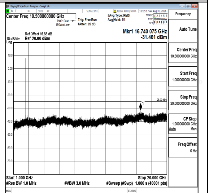
Band7-10MHz-QPSK-21100-1RB#0-1000~20000-PASS
