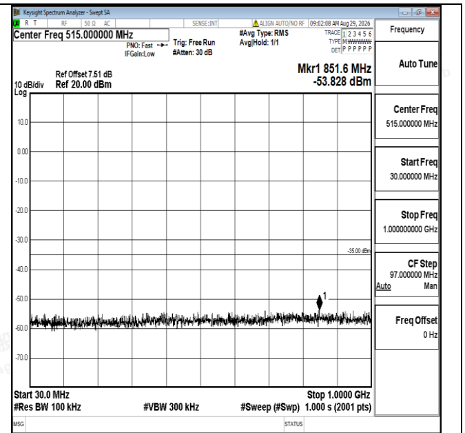
Band7-5MHz-16QAM-21100-1RB#0-30~1000-PASS
