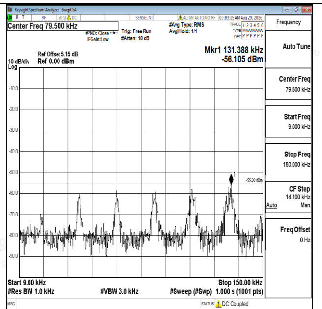
Band7-5MHz-16QAM-21425-1RB#0-0.009~0.15-PASS
