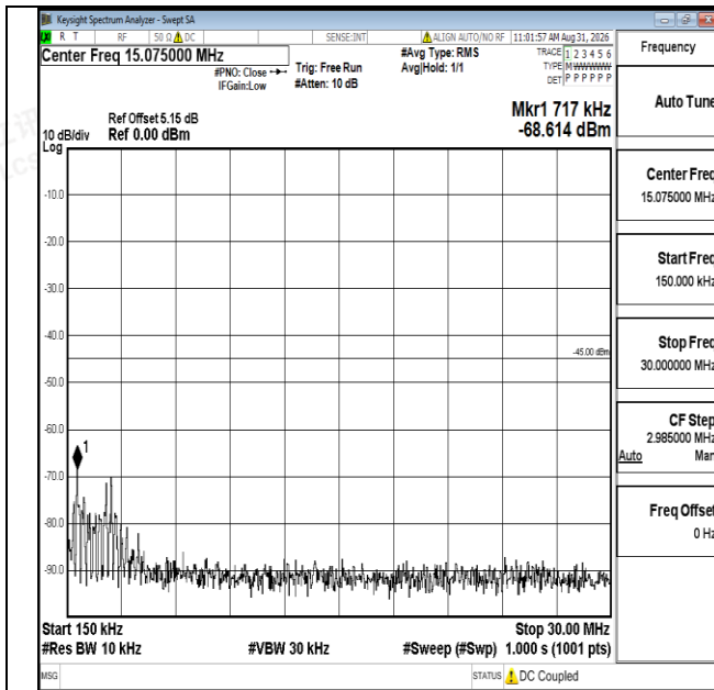
Band7-15MHz-16QAM-21100-1RB#0-0.15~30-PASS
