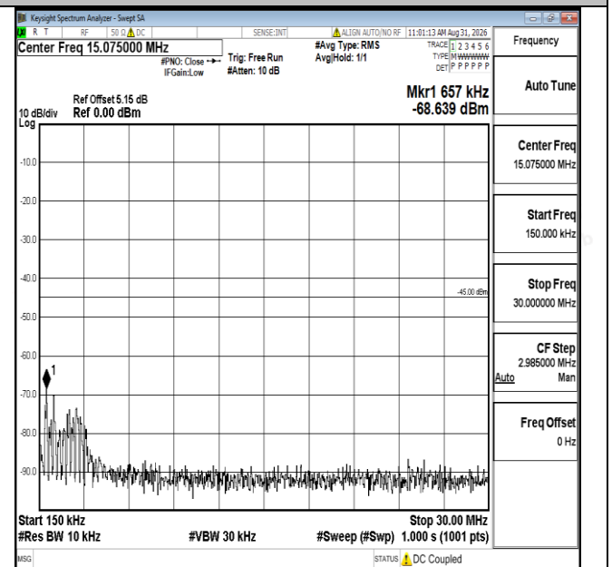
Band7-15MHz-QPSK-21100-1RB#0-0.15~30-PASS
