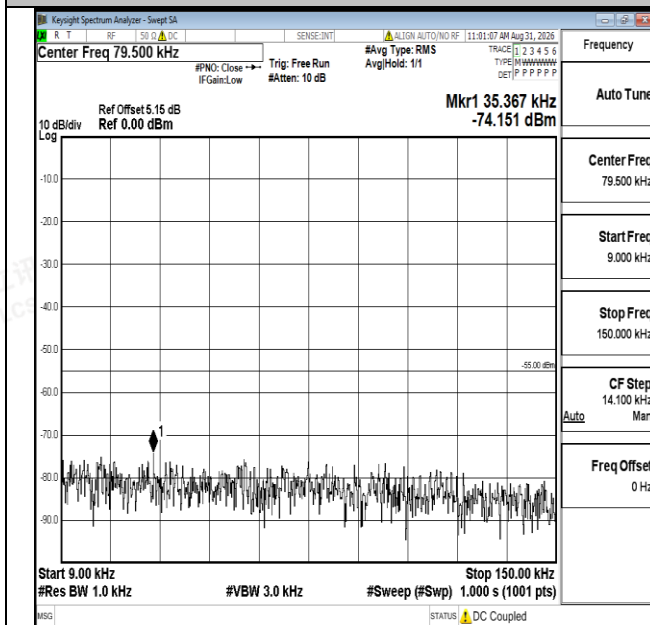
Band7-15MHz-QPSK-21100-1RB#0-0.009~0.15-PASS
