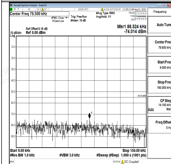
Band7-20MHz-QPSK-20850-1RB#0-0.009~0.15-PASS
