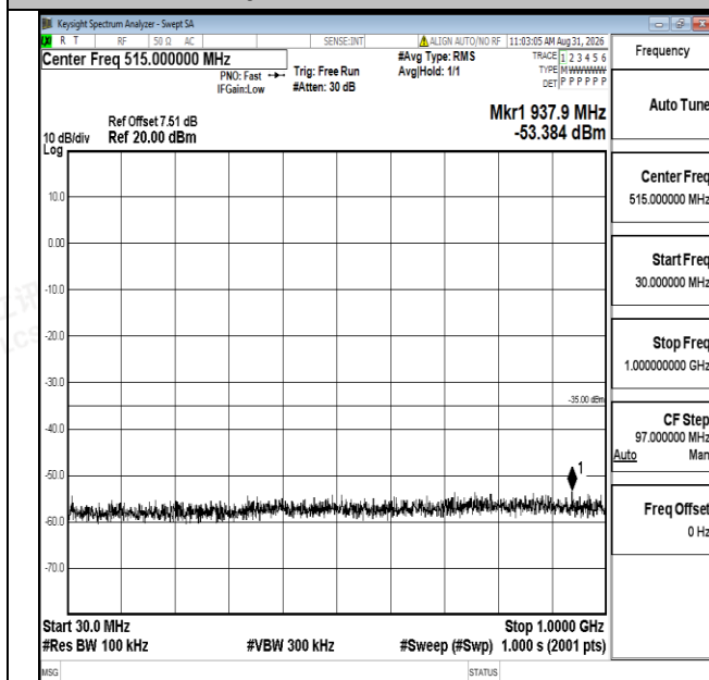
Band7-15MHz-QPSK-21375-1RB#0-30~1000-PASS
