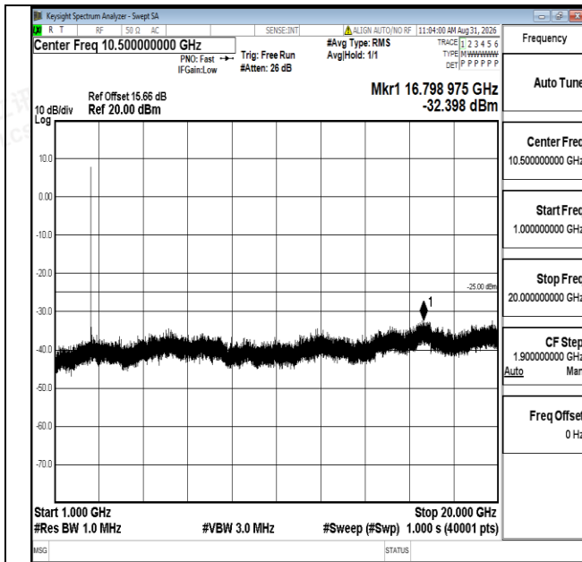
Band7-15MHz-16QAM-21375-1RB#0-1000~20000-PASS
