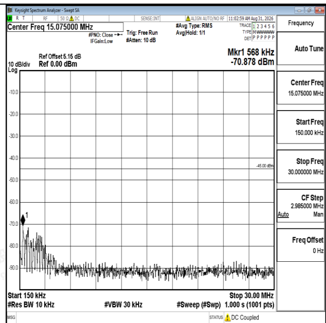
Band7-15MHz-QPSK-21375-1RB#0-0.15~30-PASS
