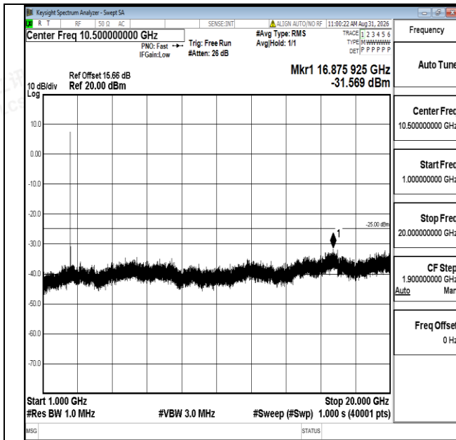
Band7-15MHz-16QAM-20825-1RB#0-1000~20000-PASS
