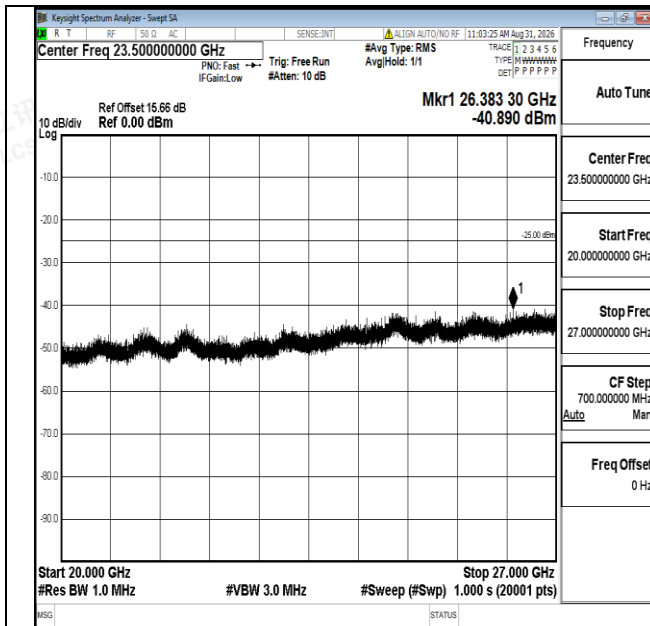
Band7-15MHz-QPSK-21375-1RB#0-20000~27000-PASS
