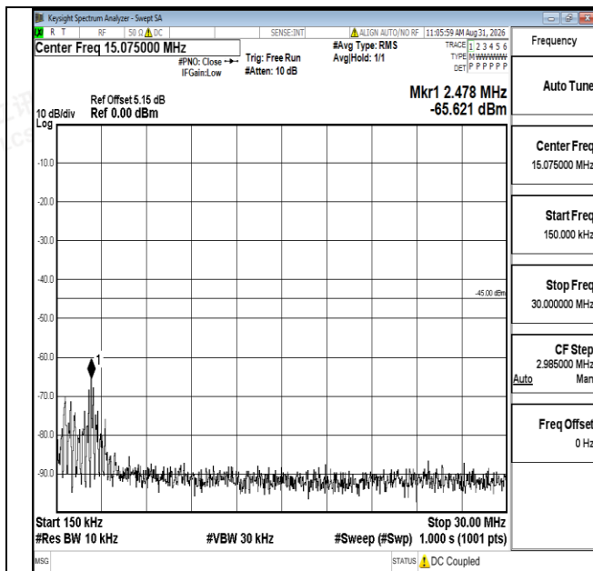
Band7-20MHz-16QAM-20850-1RB#0-0.15~30-PASS
