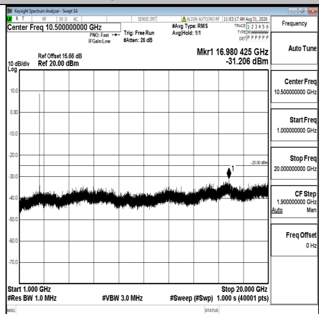
Band7-15MHz-QPSK-21375-1RB#0-1000~20000-PASS
