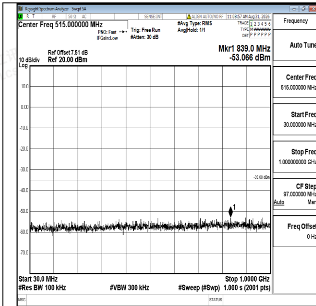
Band7-20MHz-QPSK-21350-1RB#0-30~1000-PASS
