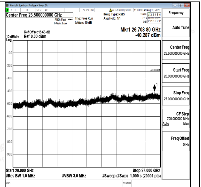
Band7-15MHz-16QAM-21375-1RB#0-20000~27000-PASS
