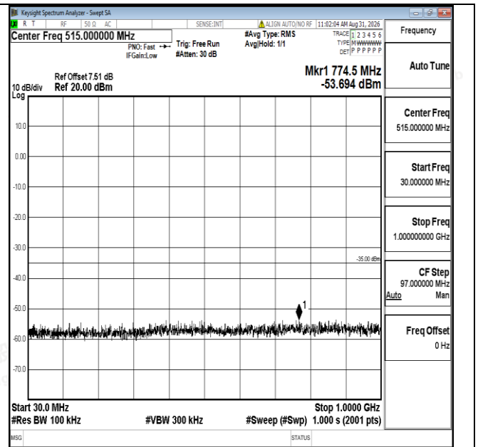
Band7-15MHz-16QAM-21100-1RB#0-30~1000-PASS
