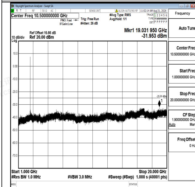
Band7-15MHz-16QAM-21100-1RB#0-1000~20000-PASS
