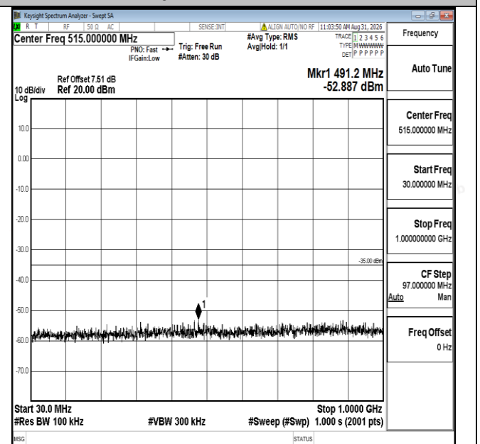
Band7-15MHz-16QAM-21375-1RB#0-30~1000-PASS
