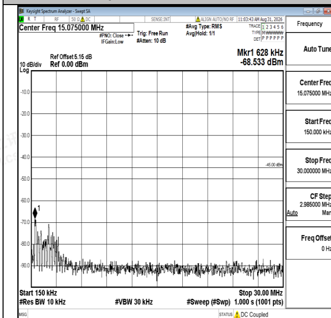
Band7-15MHz-16QAM-21375-1RB#0-0.15~30-PASS
