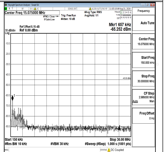
Band7-20MHz-QPSK-20850-1RB#0-0.15~30-PASS
