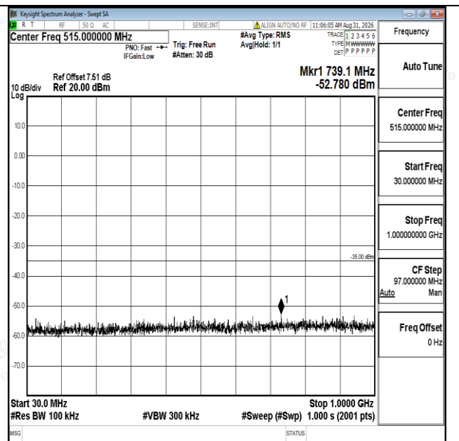
Band7-20MHz-16QAM-20850-1RB#0-30~1000-PASS
