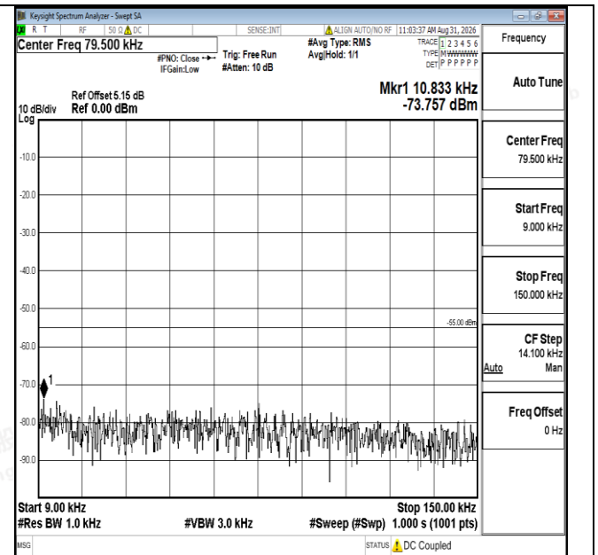
Band7-15MHz-16QAM-21375-1RB#0-0.009~0.15-PASS
