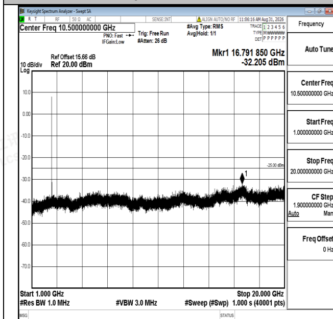
Band7-20MHz-16QAM-20850-1RB#0-1000~20000-PASS
