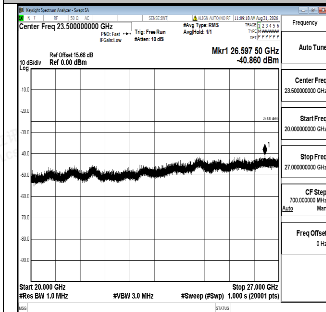
Band7-20MHz-QPSK-21350-1RB#0-20000~27000-PASS
