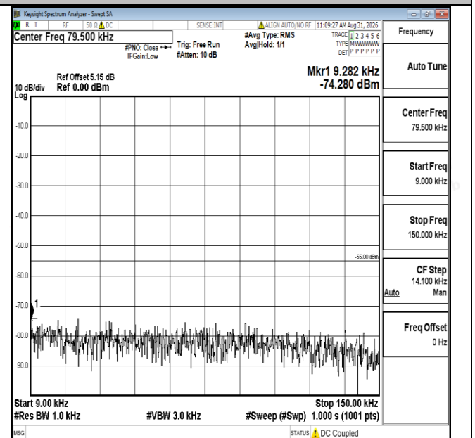
Band7-20MHz-16QAM-21350-1RB#0-0.009~0.15-PASS
