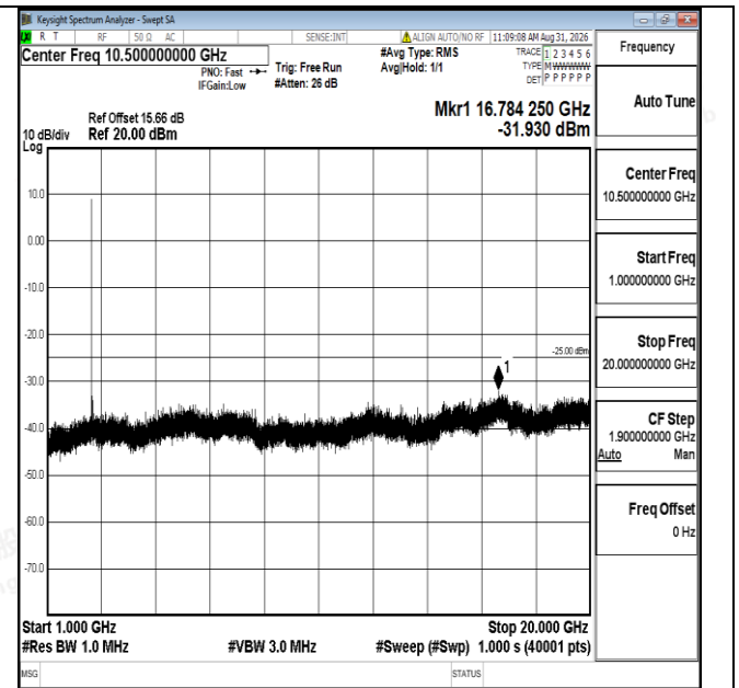
Band7-20MHz-QPSK-21350-1RB#0-1000~20000-PASS
