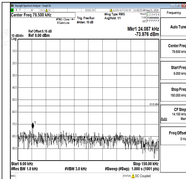
Band7-15MHz-QPSK-21375-1RB#0-0.009~0.15-PASS
