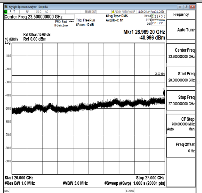
Band7-20MHz-16QAM-20850-1RB#0-20000~27000-PASS
