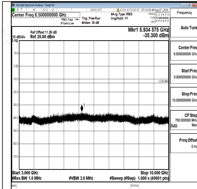
Band12-1.4MHz-QPSK-23017-1RB#0-3000~10000-PASS
