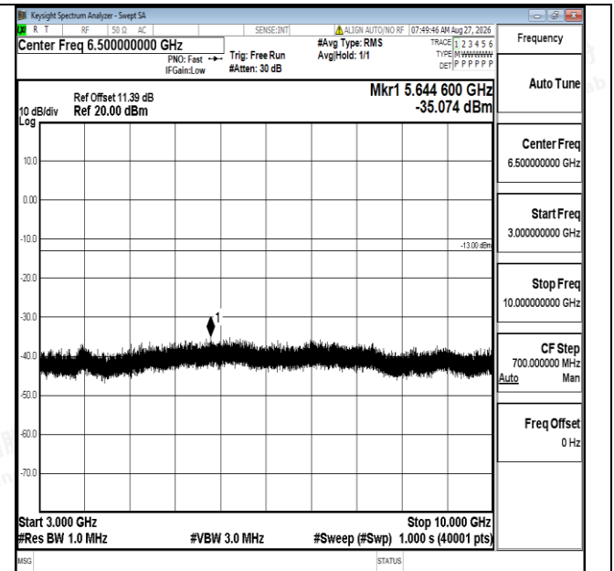
Band12-3MHz-16QAM-23095-1RB#0-3000~10000-PASS
