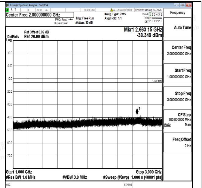
Band12-1.4MHz-QPSK-23095-1RB#0-1000~3000-PASS
