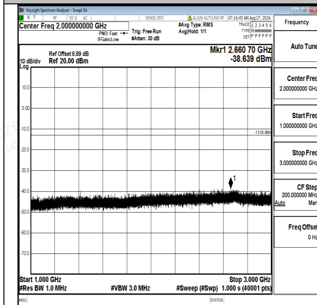
Band12-1.4MHz-16QAM-23095-1RB#0-1000~3000-PASS
