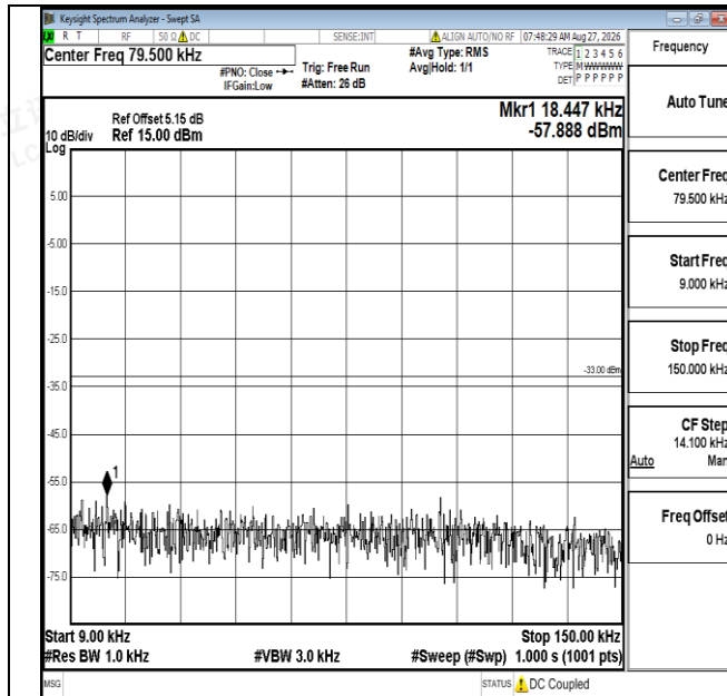
Band12-3MHz-QPSK-23095-1RB#0-0.009~0.15-PASS
