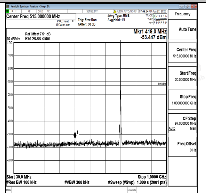
Band12-3MHz-16QAM-23095-1RB#0-30~1000-PASS
