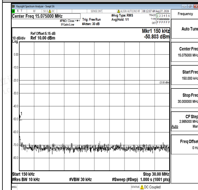
Band12-5MHz-16QAM-23035-1RB#0-0.15~30-PASS
