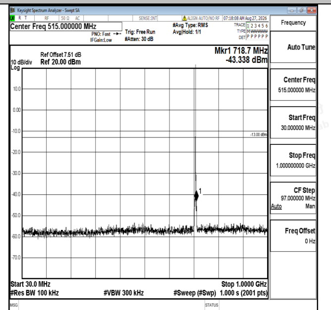
Band12-1.4MHz-16QAM-23173-1RB#0-30~1000-PASS
