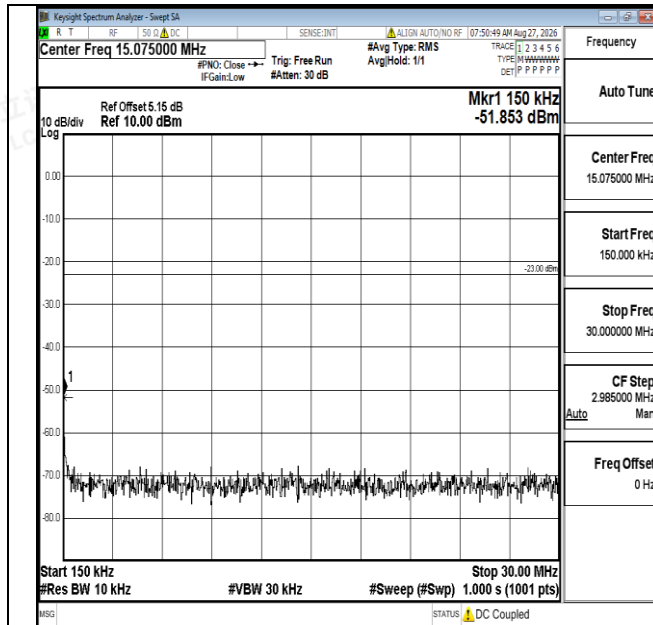
Band12-3MHz-16QAM-23165-1RB#0-0.15~30-PASS
