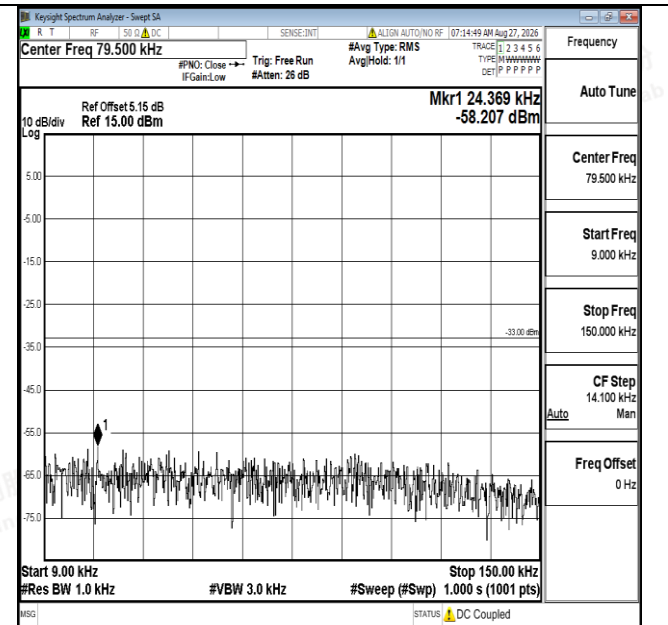
Band12-1.4MHz-16QAM-23017-1RB#0-0.009~0.15-PASS
