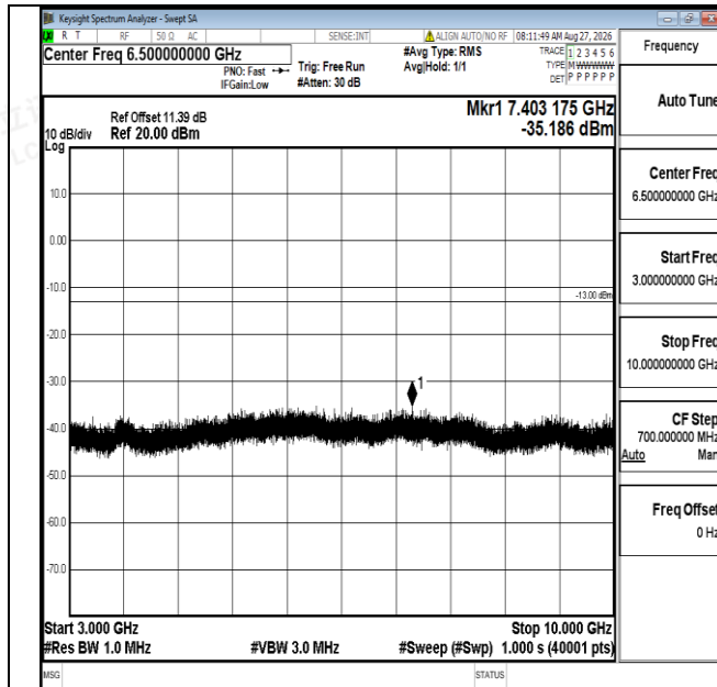
Band12-5MHz-QPSK-23035-1RB#0-3000~10000-PASS
