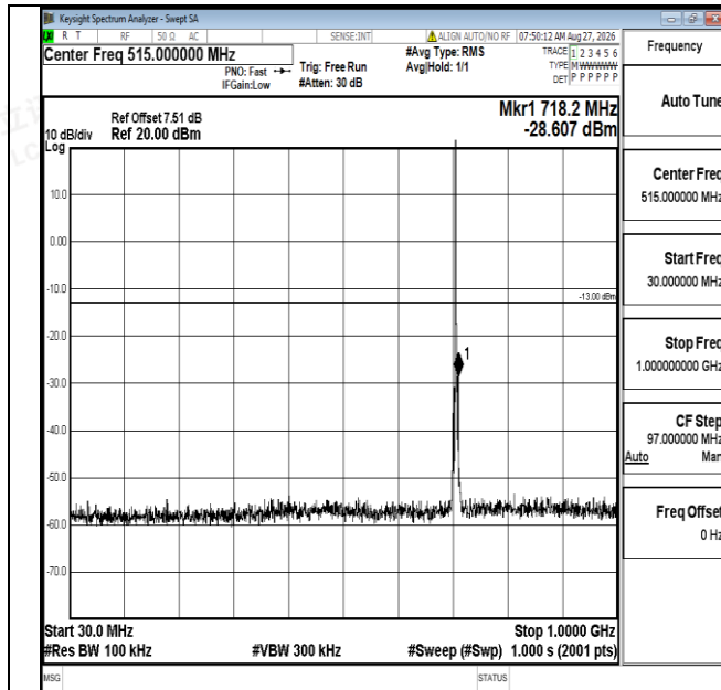
Band12-3MHz-QPSK-23165-1RB#0-30~1000-PASS
