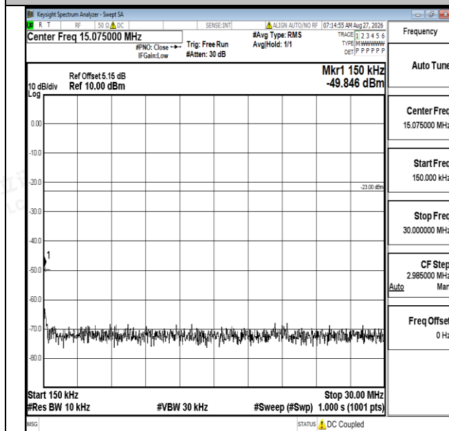
Band12-1.4MHz-16QAM-23017-1RB#0-0.15~30-PASS
