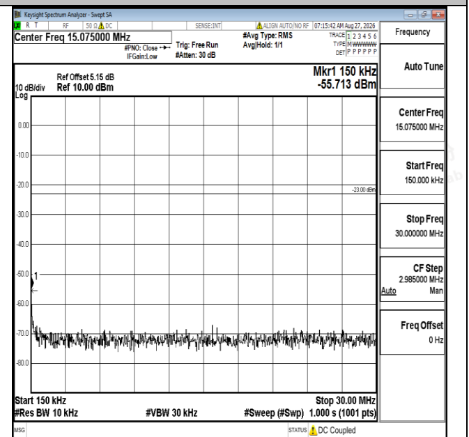
Band12-1.4MHz-QPSK-23095-1RB#0-0.15~30-PASS
