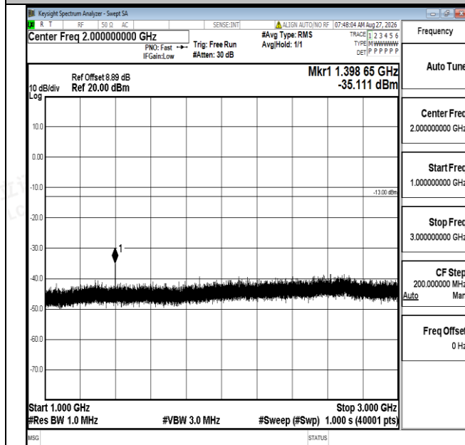
Band12-3MHz-16QAM-23025-1RB#0-1000~3000-PASS
