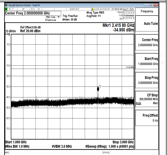
Band12-3MHz-QPSK-23095-1RB#0-1000~3000-PASS
