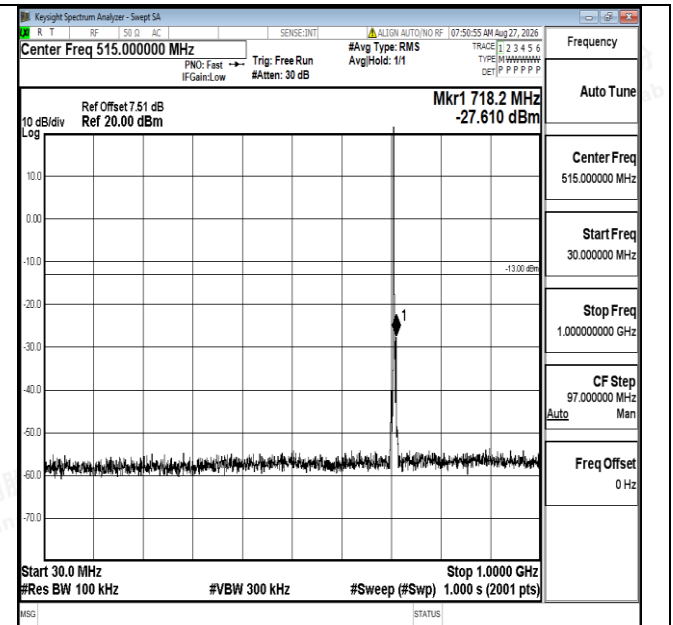
Band12-3MHz-16QAM-23165-1RB#0-30~1000-PASS
