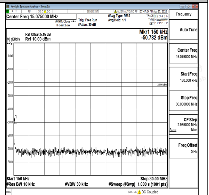
Band12-3MHz-QPSK-23025-1RB#0-0.15~30-PASS
