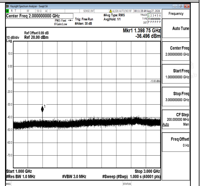
Band12-5MHz-QPSK-23035-1RB#0-1000~3000-PASS
