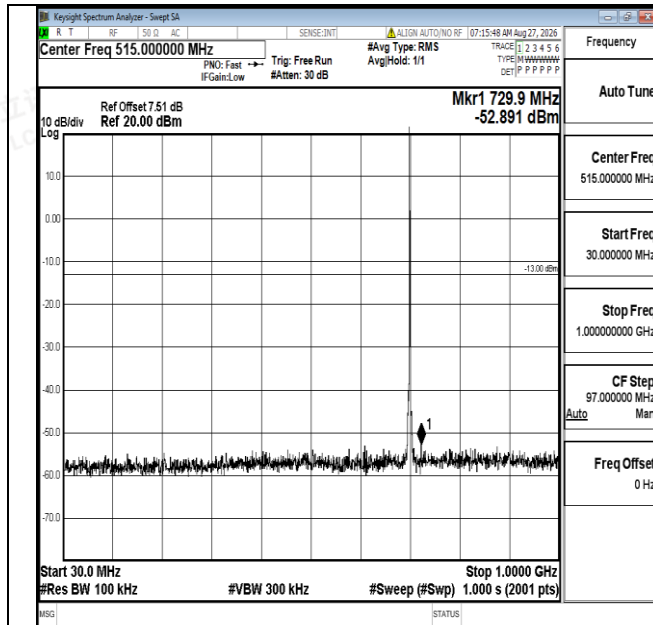
Band12-1.4MHz-QPSK-23095-1RB#0-30~1000-PASS
