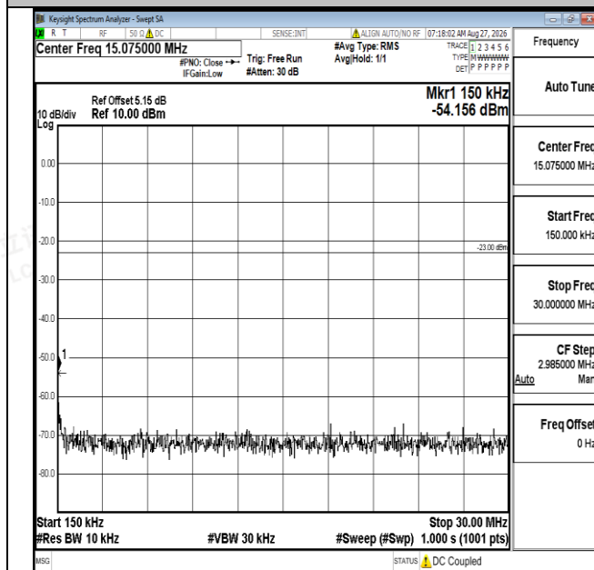
Band12-1.4MHz-16QAM-23173-1RB#0-0.15~30-PASS
