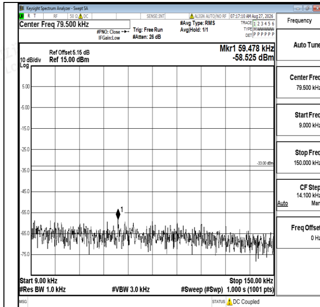
Band12-1.4MHz-QPSK-23173-1RB#0-0.009~0.15-PASS
