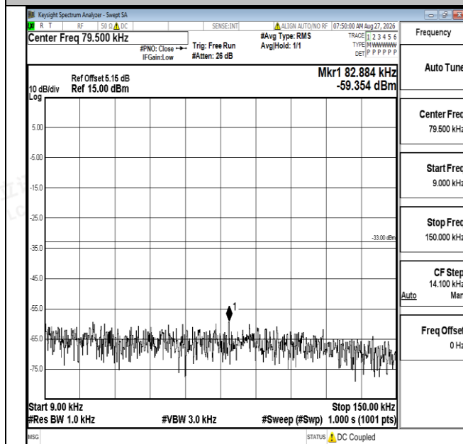
Band12-3MHz-QPSK-23165-1RB#0-0.009~0.15-PASS
