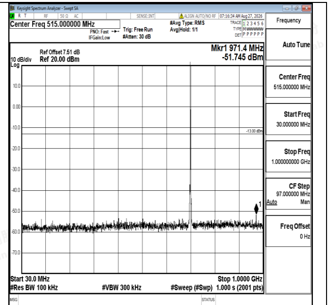
Band12-1.4MHz-16QAM-23095-1RB#0-30~1000-PASS
