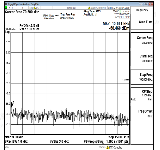
Band12-3MHz-16QAM-23095-1RB#0-0.009~0.15-PASS
