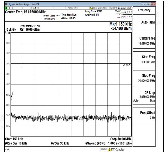
Band12-3MHz-QPSK-23095-1RB#0-0.15~30-PASS
