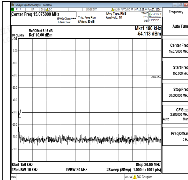
Band12-1.4MHz-16QAM-23095-1RB#0-0.15~30-PASS
