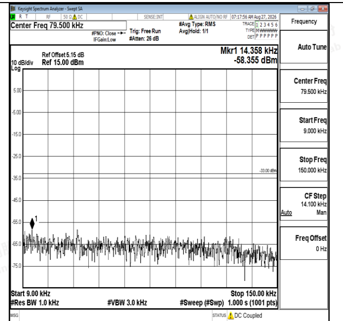
Band12-1.4MHz-16QAM-23173-1RB#0-0.009~0.15-PASS
