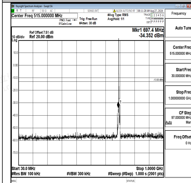
Band12-5MHz-QPSK-23035-1RB#0-30~1000-PASS
