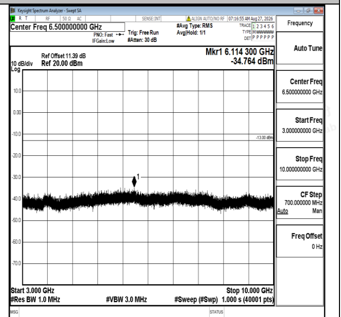
Band12-1.4MHz-16QAM-23095-1RB#0-3000~10000-PASS
