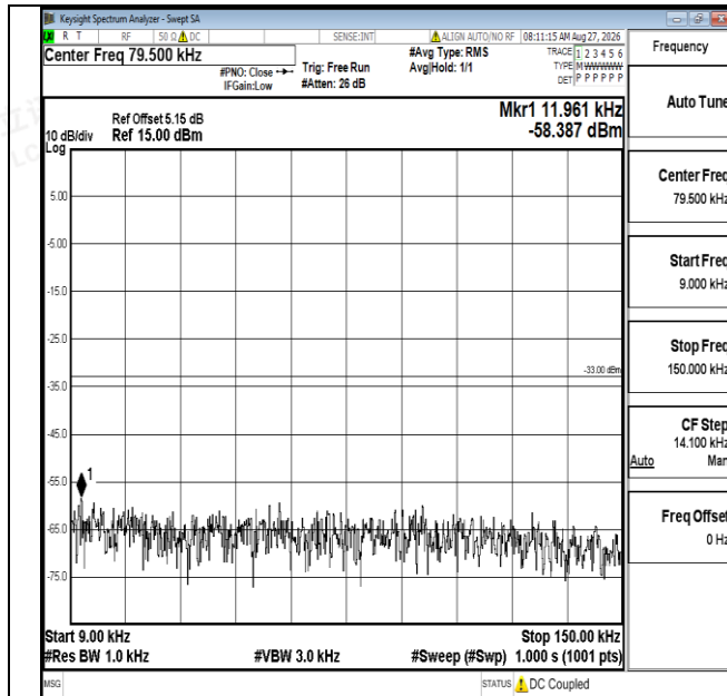
Band12-5MHz-QPSK-23035-1RB#0-0.009~0.15-PASS
