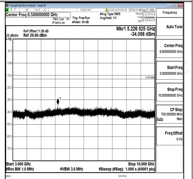
Band12-3MHz-16QAM-23165-1RB#0-3000~10000-PASS
