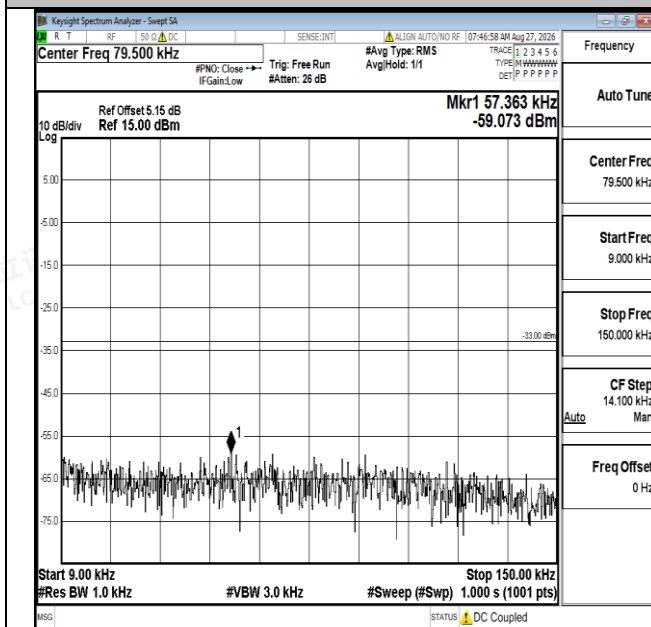
Band12-3MHz-QPSK-23025-1RB#0-0.009~0.15-PASS
