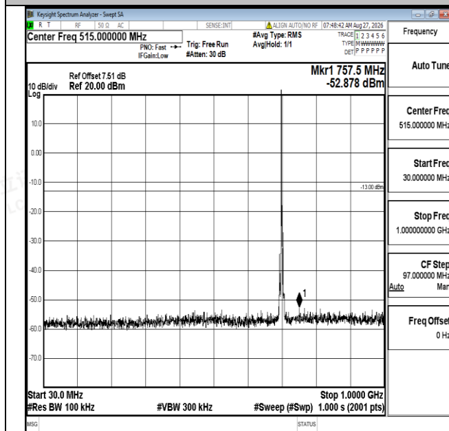
Band12-3MHz-QPSK-23095-1RB#0-30~1000-PASS
