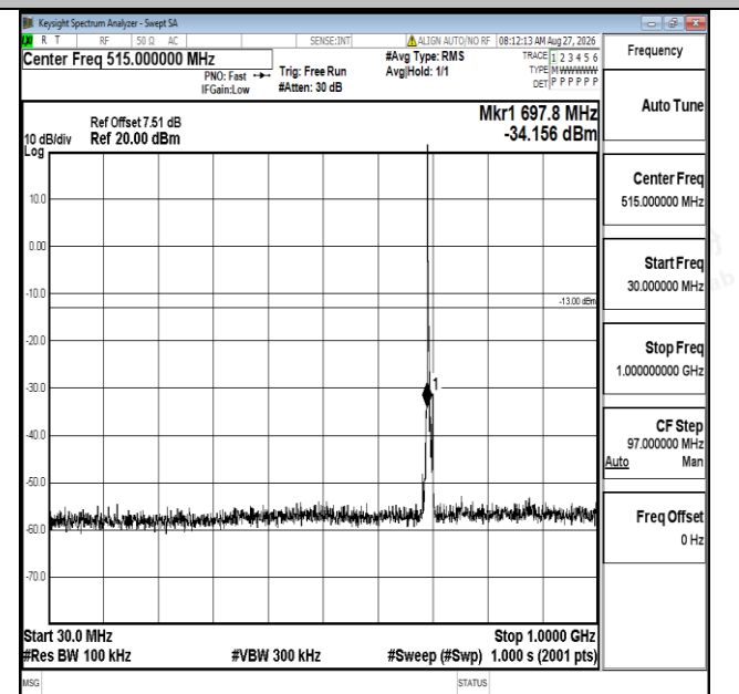
Band12-5MHz-16QAM-23035-1RB#0-30~1000-PASS
