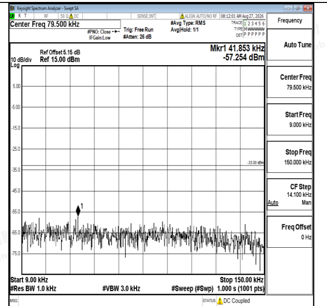
Band12-5MHz-16QAM-23035-1RB#0-0.009~0.15-PASS
