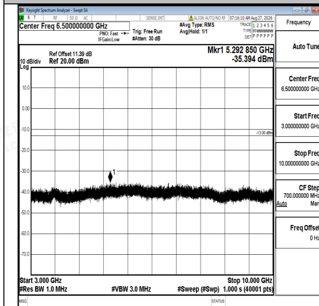
Band12-1.4MHz-QPSK-23095-1RB#0-3000~10000-PASS
