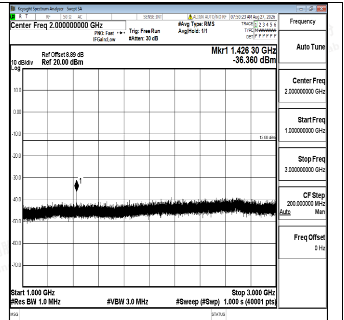
Band12-3MHz-QPSK-23165-1RB#0-1000~3000-PASS
