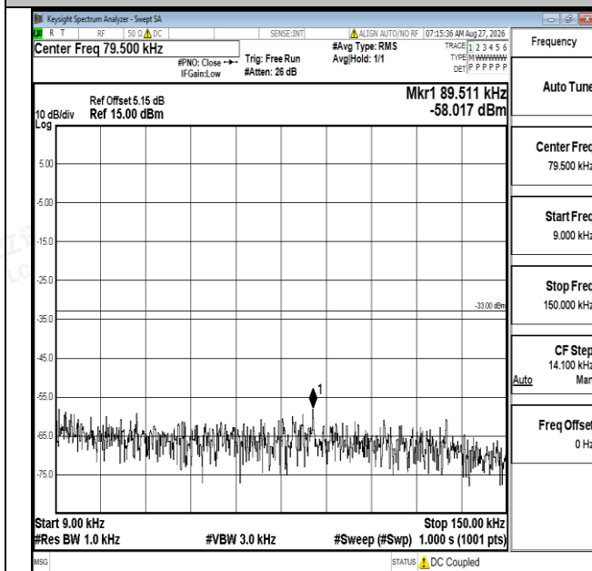
Band12-1.4MHz-QPSK-23095-1RB#0-0.009~0.15-PASS
