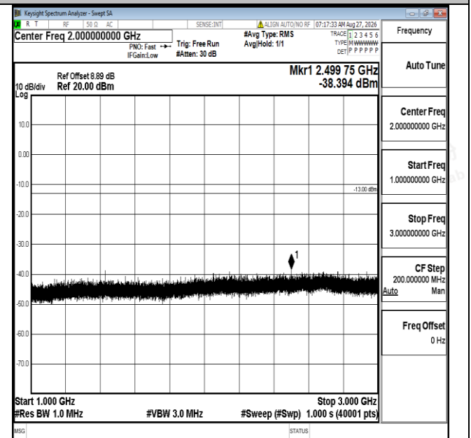
Band12-1.4MHz-QPSK-23173-1RB#0-1000~3000-PASS
