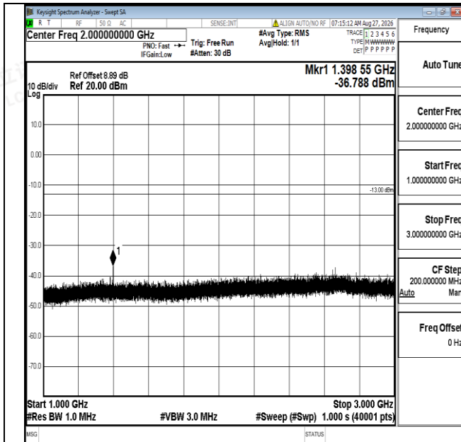
Band12-1.4MHz-16QAM-23017-1RB#0-1000~3000-PASS
