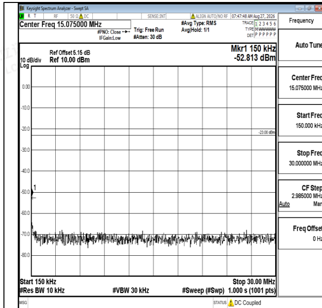
Band12-3MHz-16QAM-23025-1RB#0-0.15~30-PASS
