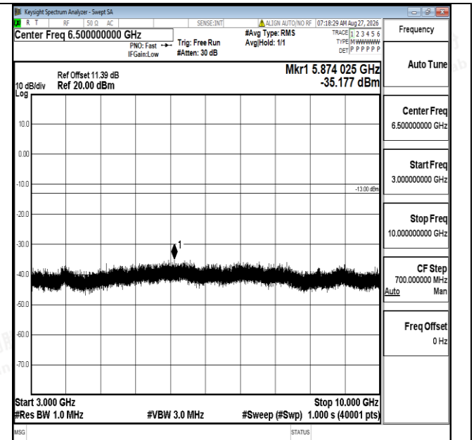
Band12-1.4MHz-16QAM-23173-1RB#0-3000~10000-PASS
