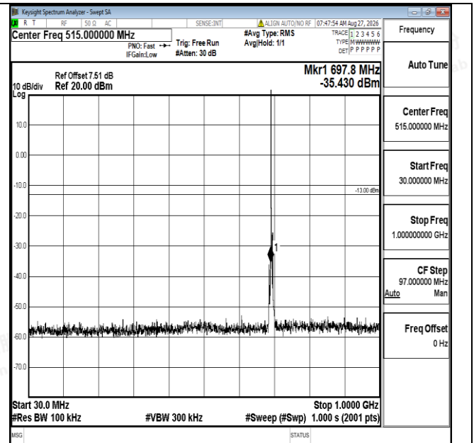
Band12-3MHz-16QAM-23025-1RB#0-30~1000-PASS
