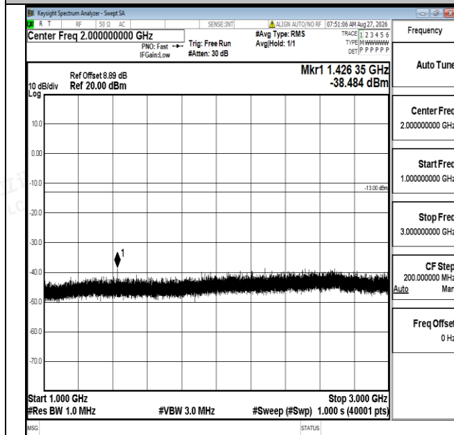
Band12-3MHz-16QAM-23165-1RB#0-1000~3000-PASS
