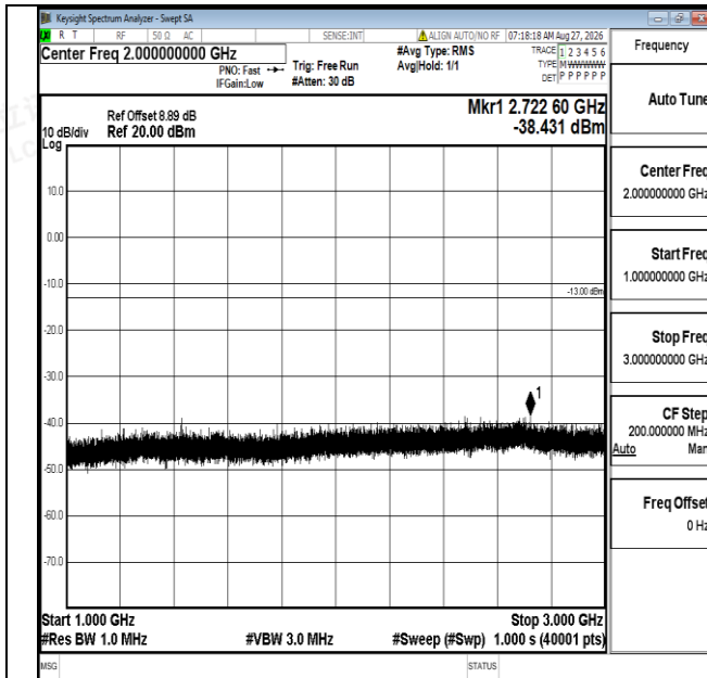
Band12-1.4MHz-16QAM-23173-1RB#0-1000~3000-PASS
