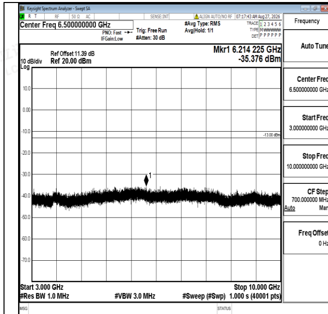
Band12-1.4MHz-QPSK-23173-1RB#0-3000~10000-PASS
