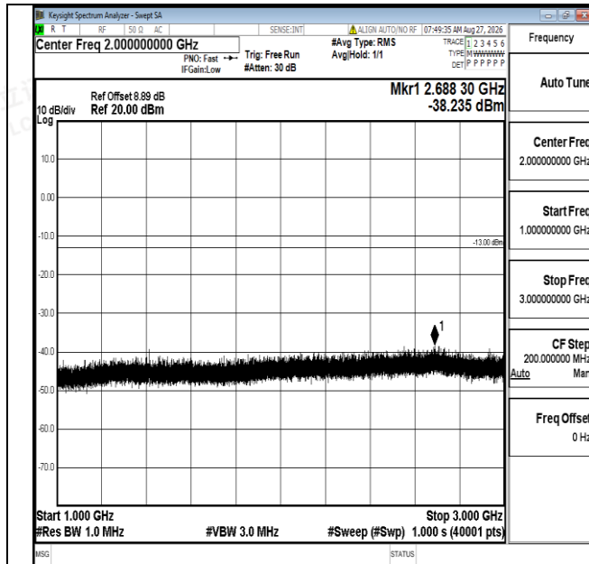
Band12-3MHz-16QAM-23095-1RB#0-1000~3000-PASS
