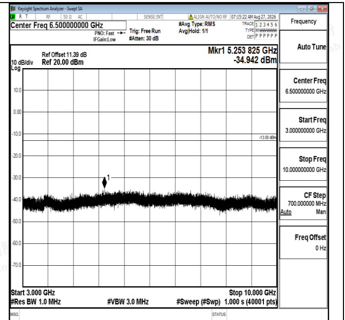
Band12-1.4MHz-16QAM-23017-1RB#0-3000~10000-PASS
