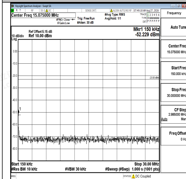
Band12-3MHz-16QAM-23095-1RB#0-0.15~30-PASS
