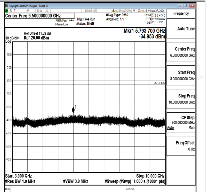
Band12-3MHz-16QAM-23025-1RB#0-3000~10000-PASS
