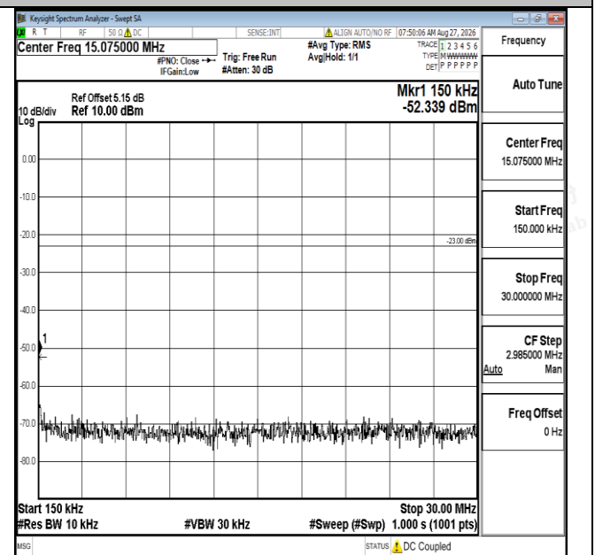
Band12-3MHz-QPSK-23165-1RB#0-0.15~30-PASS
