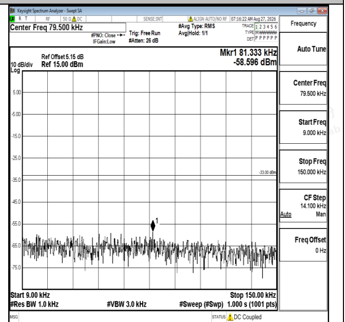
Band12-1.4MHz-16QAM-23095-1RB#0-0.009~0.15-PASS
