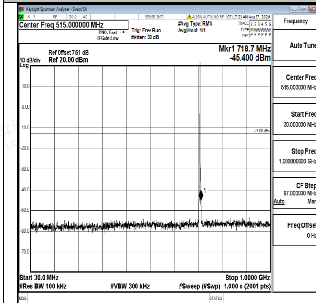
Band12-1.4MHz-QPSK-23173-1RB#0-30~1000-PASS
