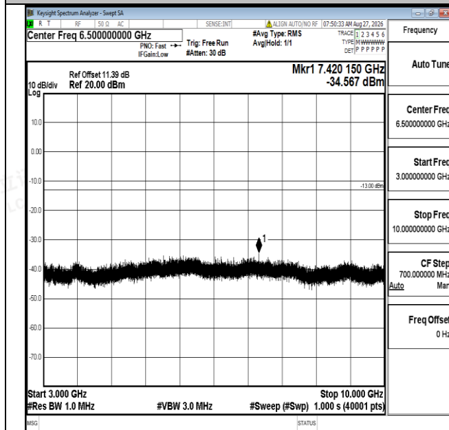
Band12-3MHz-QPSK-23165-1RB#0-3000~10000-PASS
