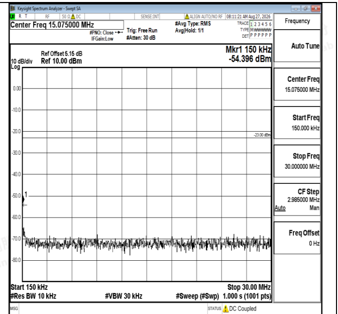
Band12-5MHz-QPSK-23035-1RB#0-0.15~30-PASS
