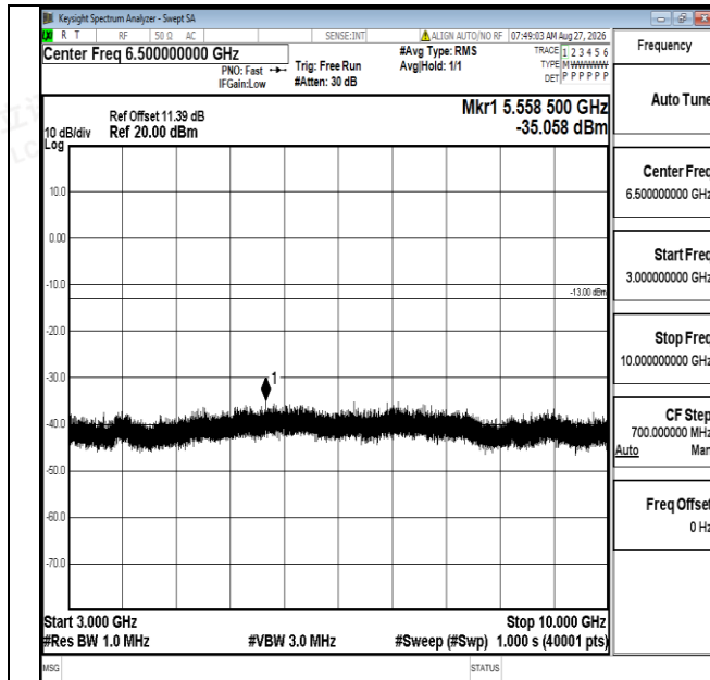
Band12-3MHz-QPSK-23095-1RB#0-3000~10000-PASS
