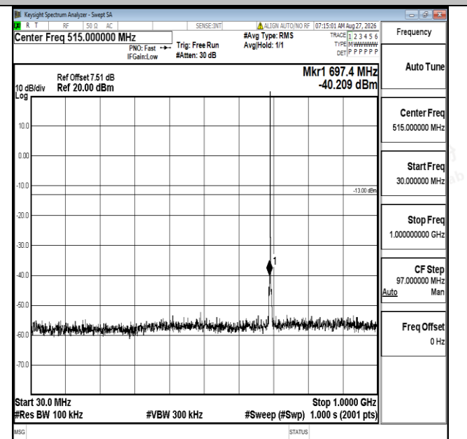
Band12-1.4MHz-16QAM-23017-1RB#0-30~1000-PASS
