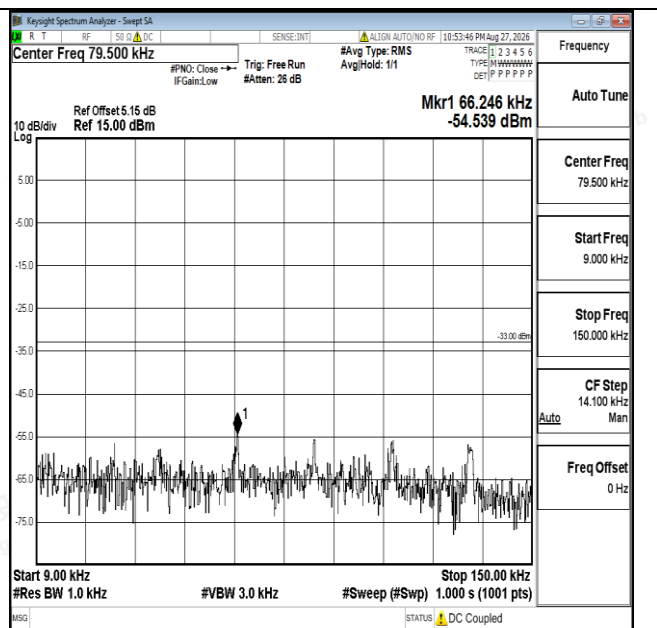
Band17-10MHz-16QAM-23780-1RB#0-0.009~0.15-PASS
