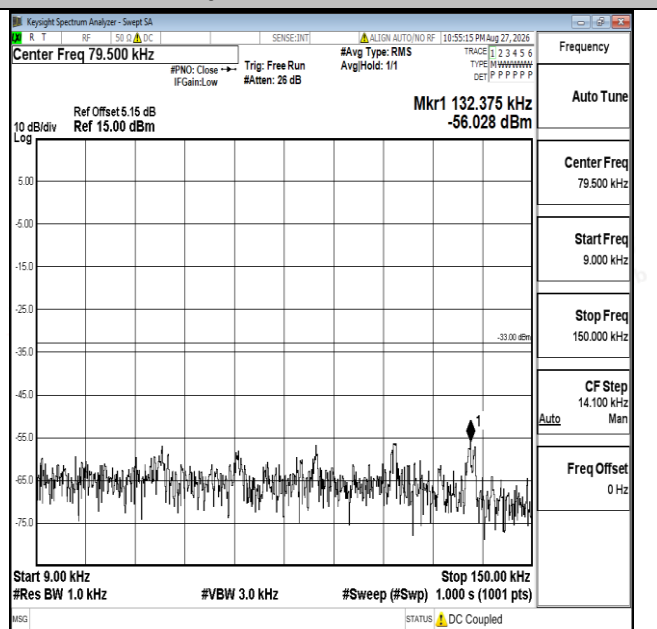
Band17-10MHz-16QAM-23790-1RB#0-0.009~0.15-PASS
