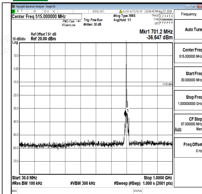
Band17-10MHz-QPSK-23790-1RB#0-30~1000-PASS
