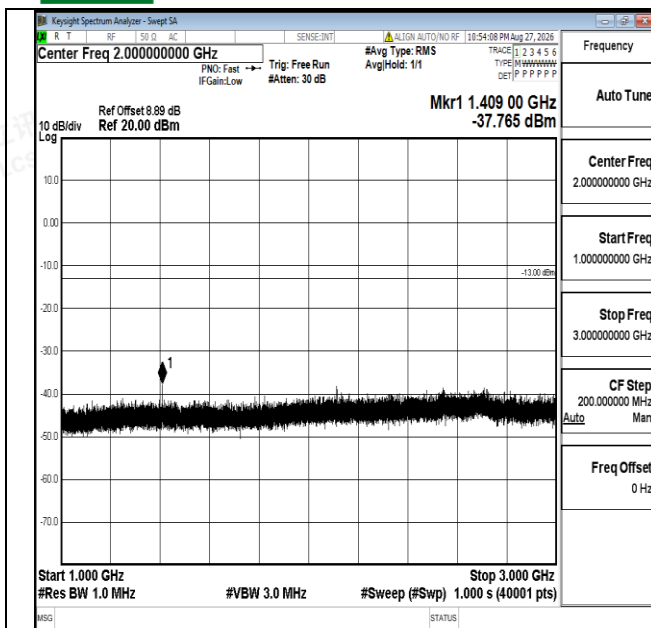
Band17-10MHz-16QAM-23780-1RB#0-1000~3000-PASS
