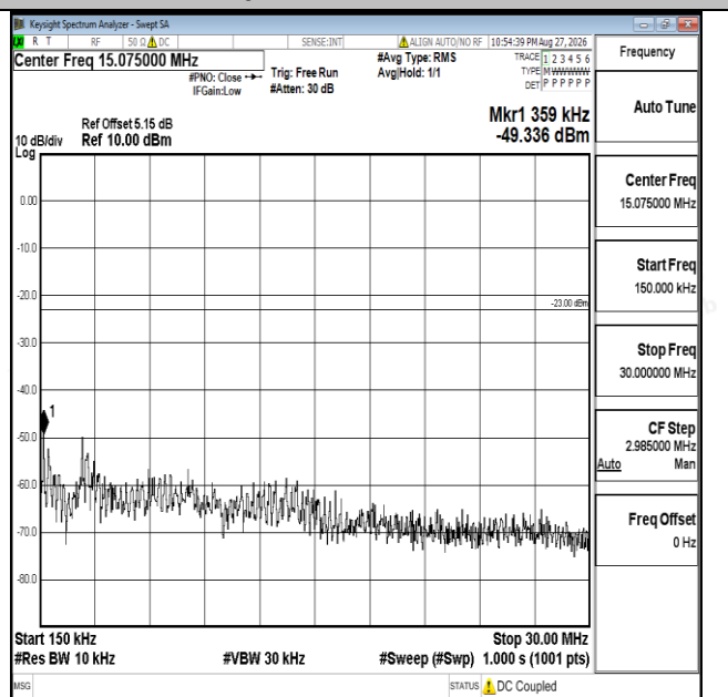
Band17-10MHz-QPSK-23790-1RB#0-0.15~30-PASS
