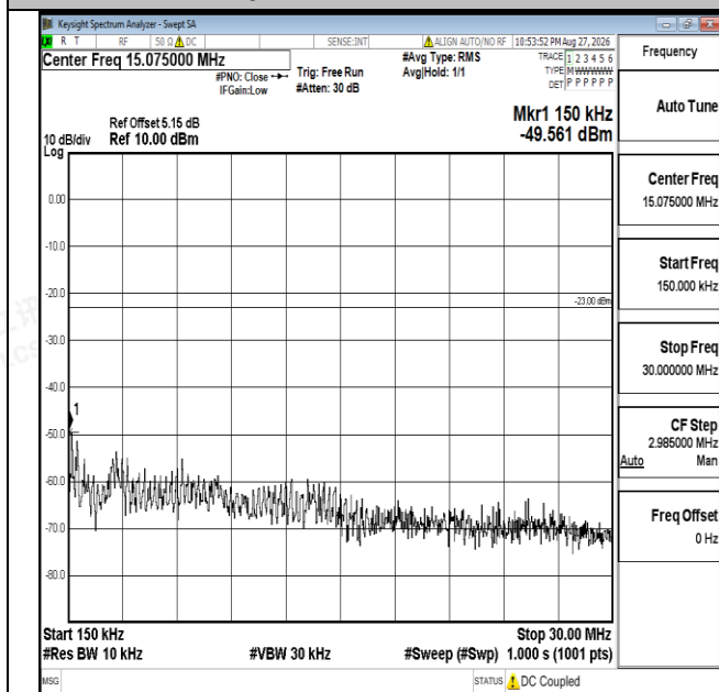
Band17-10MHz-16QAM-23780-1RB#0-0.15~30-PASS
