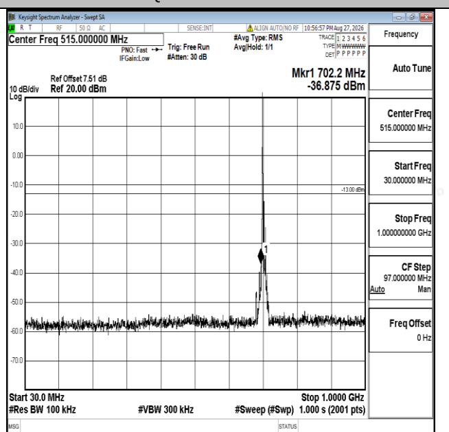
Band17-10MHz-16QAM-23800-1RB#0-30~1000-PASS
