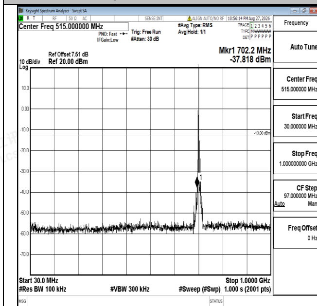
Band17-10MHz-QPSK-23800-1RB#0-30~1000-PASS
