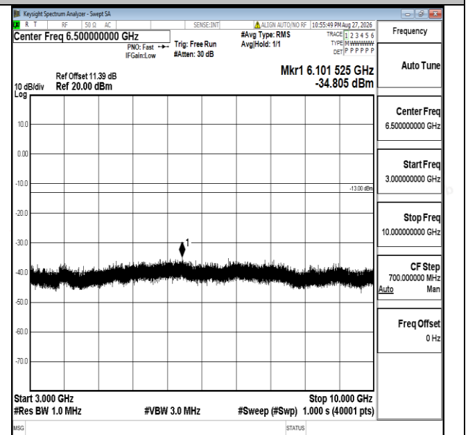
Band17-10MHz-16QAM-23790-1RB#0-3000~10000-PASS
