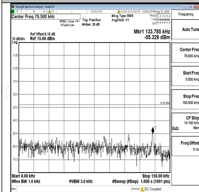
Band17-10MHz-QPSK-23790-1RB#0-0.009~0.15-PASS
