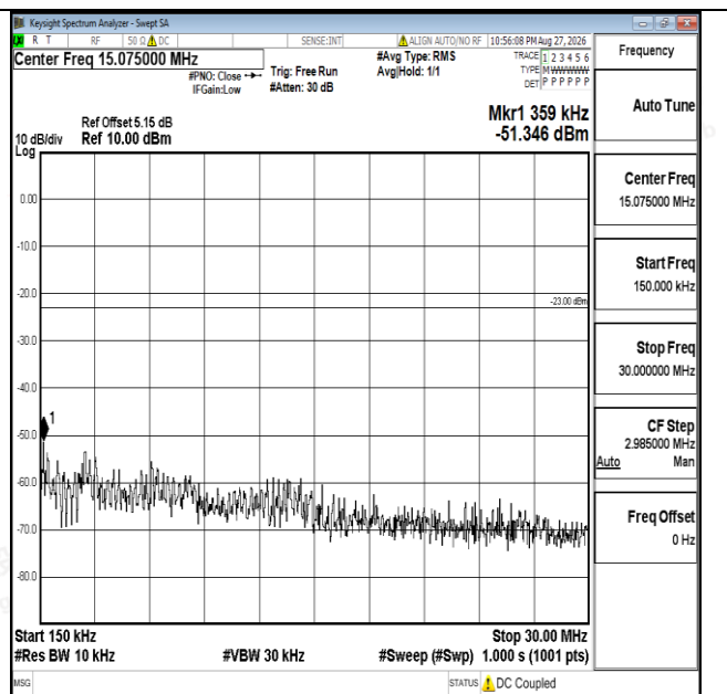
Band17-10MHz-QPSK-23800-1RB#0-0.15~30-PASS
