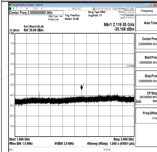
Band17-10MHz-16QAM-23790-1RB#0-1000~3000-PASS
