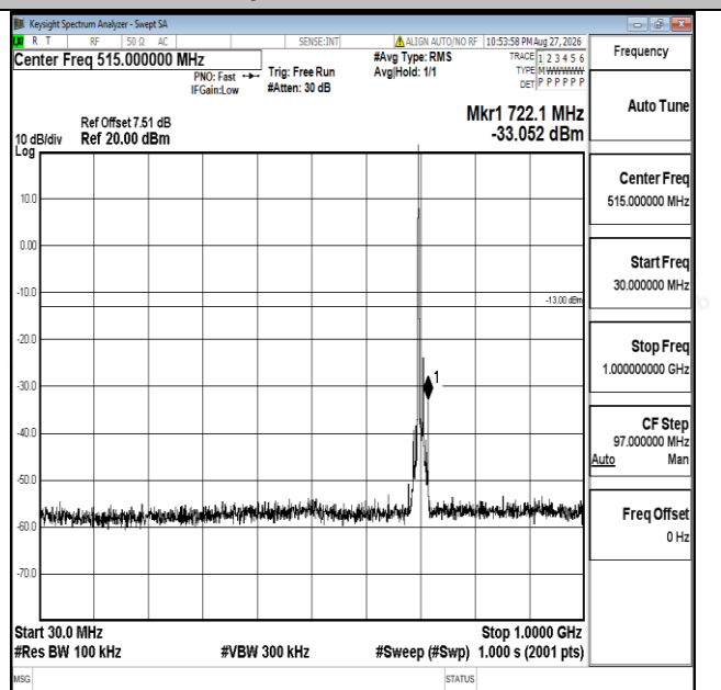
Band17-10MHz-16QAM-23780-1RB#0-30~1000-PASS
