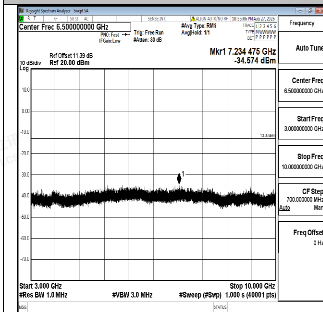
Band17-10MHz-QPSK-23790-1RB#0-3000~10000-PASS
