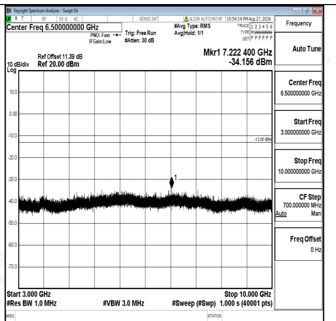
Band17-10MHz-16QAM-23780-1RB#0-3000~10000-PASS
