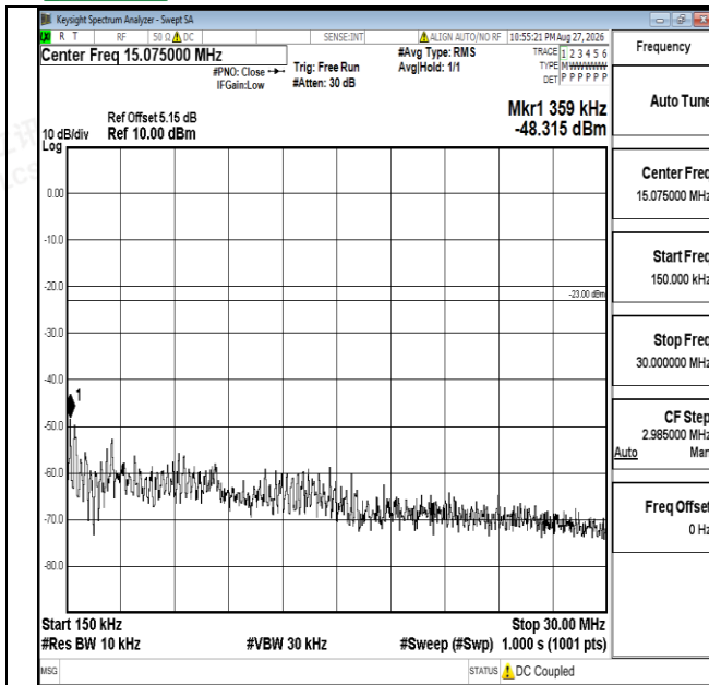
Band17-10MHz-16QAM-23790-1RB#0-0.15~30-PASS
