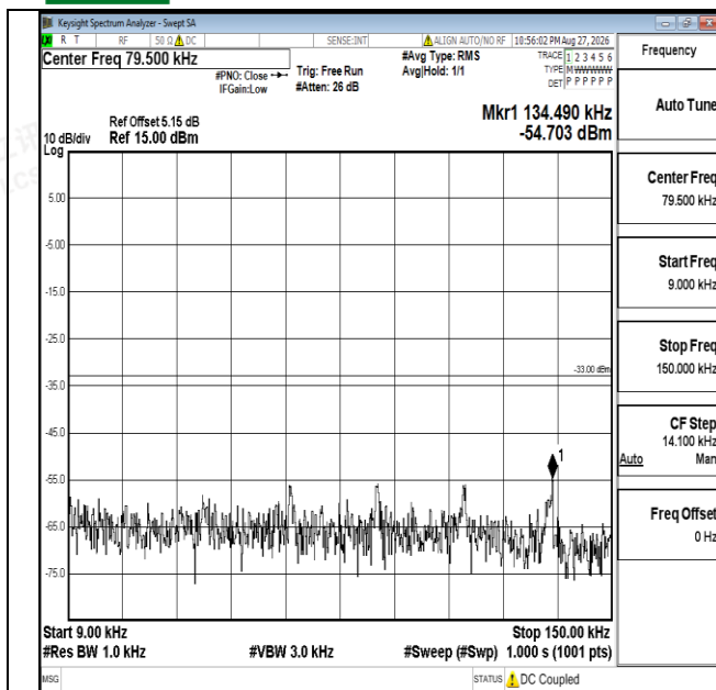
Band17-10MHz-QPSK-23800-1RB#0-0.009~0.15-PASS
