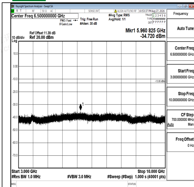
Band17-10MHz-QPSK-23780-1RB#0-3000~10000-PASS
