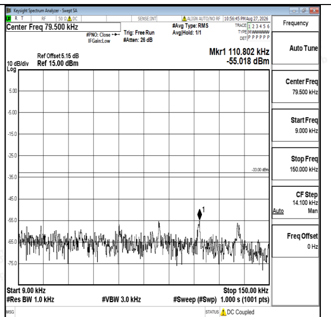
Band17-10MHz-16OAM-23800-1RB#0-0.009~0.15-PASS
