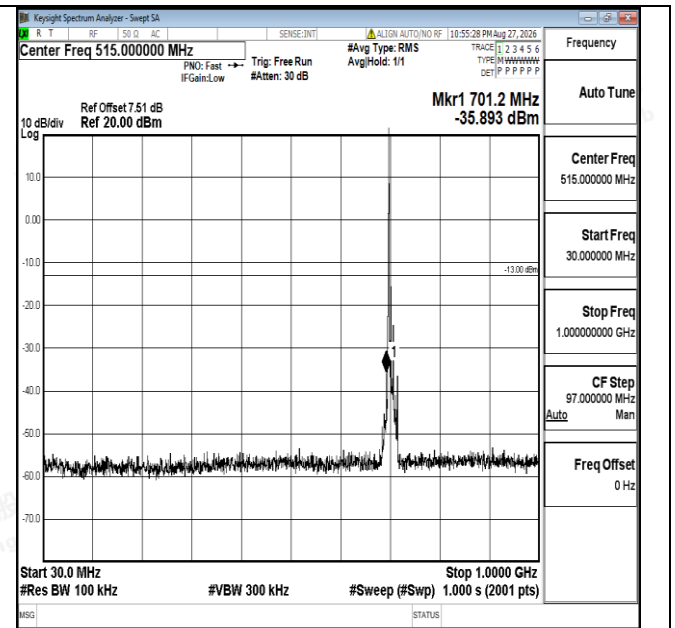
Band17-10MHz-16QAM-23790-1RB#0-30~1000-PASS
