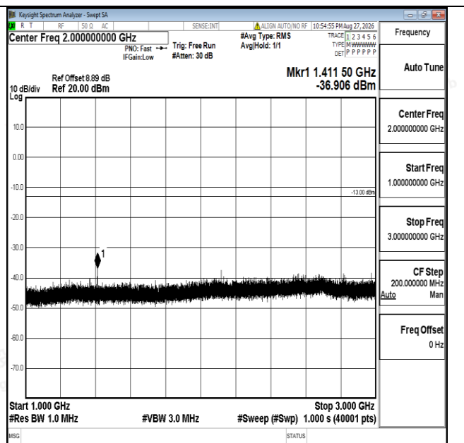
Band17-10MHz-QPSK-23790-1RB#0-1000~3000-PASS
