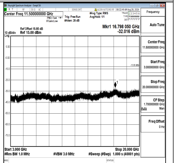
Band25-10MHz-16QAM-26365-1RB#0-3000~20000-PASS
