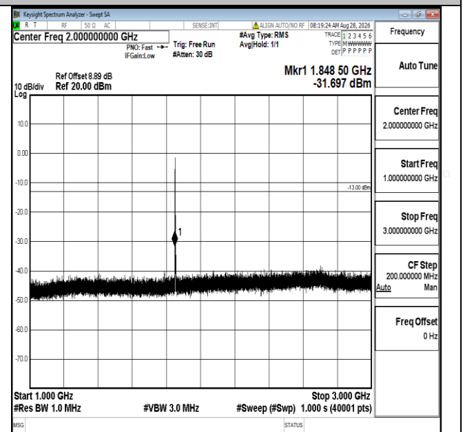
Band25-10MHz-QPSK-26090-1RB#0-1000~3000-PASS
