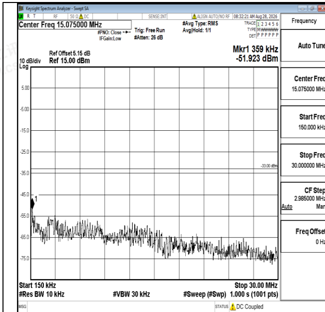
Band25-10MHz-16QAM-26365-1RB#0-0.15~30-PASS
