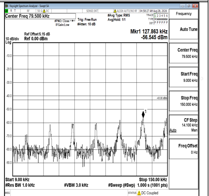
Band25-5MHz-16QAM-26665-1RB#0-0.009~0.15-PASS
