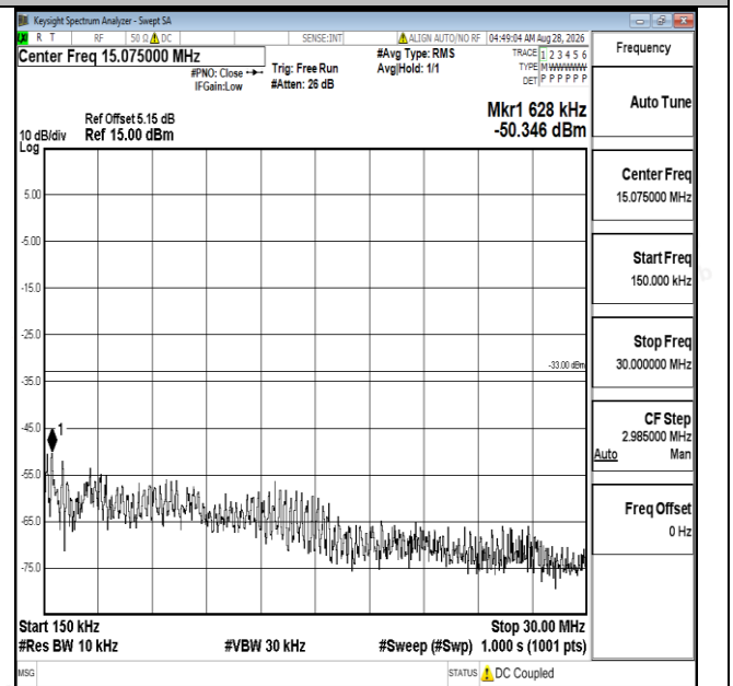
Band25-5MHz-QPSK-26065-1RB#0-0.15~30-PASS
