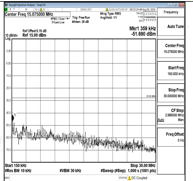
Band25-10MHz-QPSK-26640-1RB#0-0.15~30-PASS
