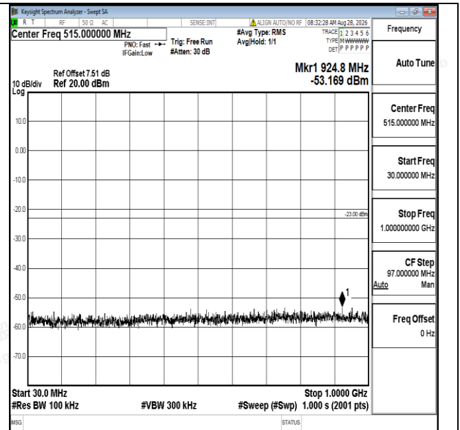
Band25-10MHz-16QAM-26365-1RB#0-30~1000-PASS
