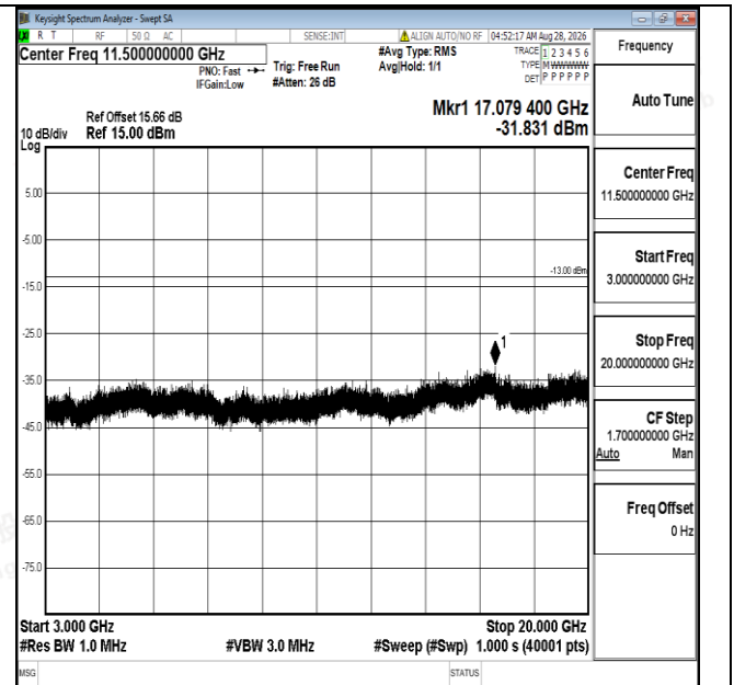
Band25-5MHz-16QAM-26365-1RB#0-3000~20000-PASS
