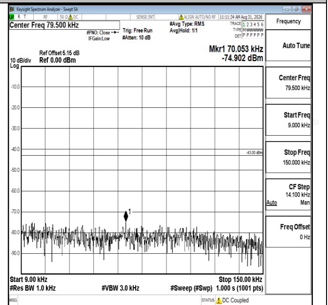
Band25-15MHz-16QAM-26115-1RB#0-0.009~0.15-PASS
