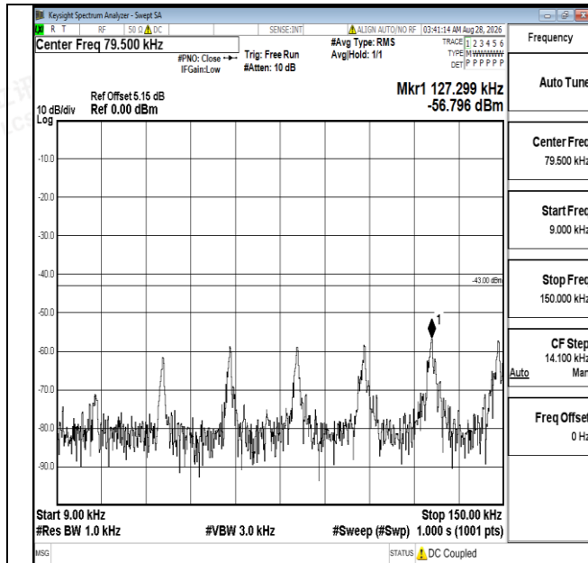
Band25-3MHz-QPSK-26675-1RB#0-0.009~0.15-PASS
