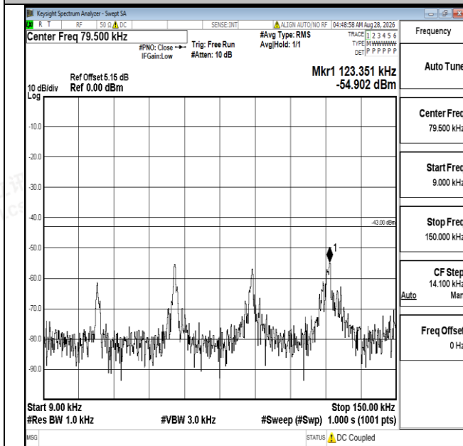
Band25-5MHz-QPSK-26065-1RB#0-0.009~0.15-PASS
