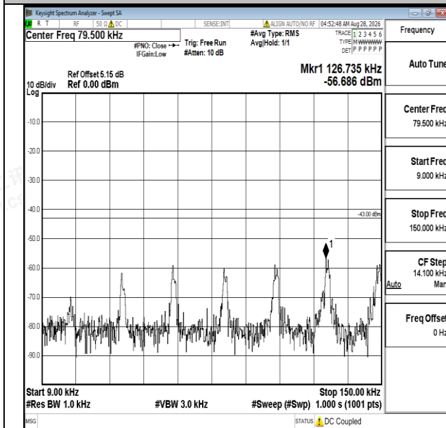
Band25-5MHz-QPSK-26665-1RB#0-0.009~0.15-PASS
