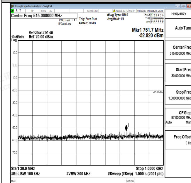
Band25-5MHz-QPSK-26365-1RB#0-30~1000-PASS
