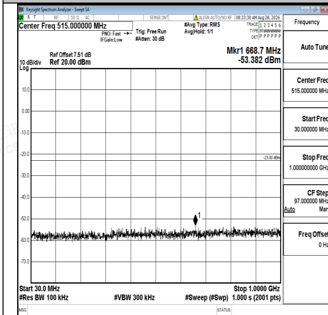
Band25-10MHz-QPSK-26640-1RB#0-30~1000-PASS
