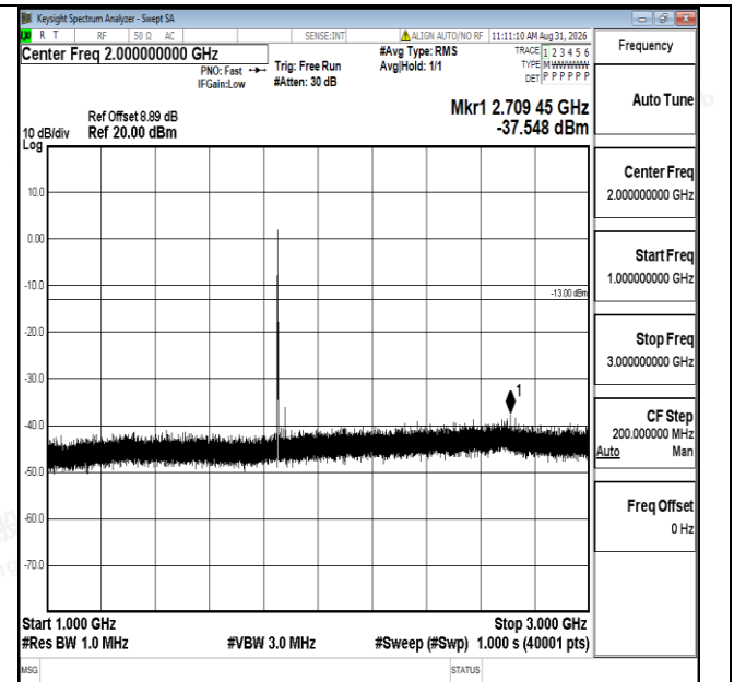
Band25-15MHz-QPSK-26115-1RB#0-1000~3000-PASS
