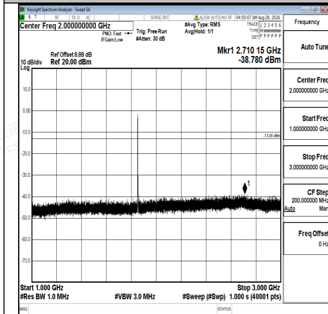
Band25-5MHz-16QAM-26065-1RB#0-1000~3000-PASS
