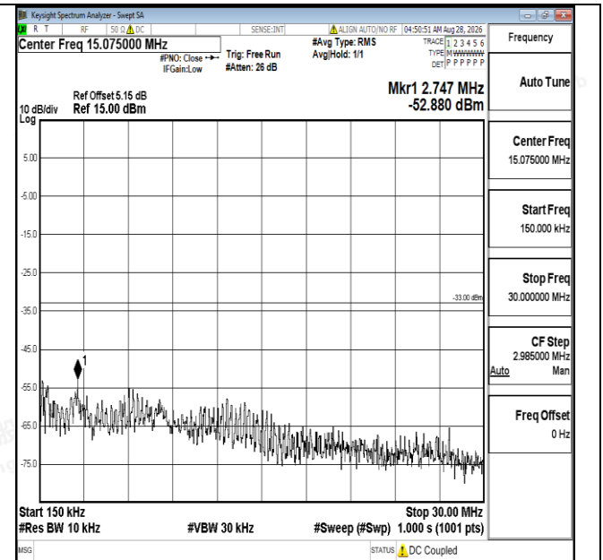
Band25-5MHz-QPSK-26365-1RB#0-0.15~30-PASS
