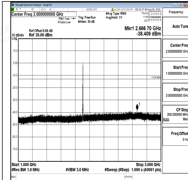
Band25-10MHz-16QAM-26640-1RB#0-1000-3000-PASS
