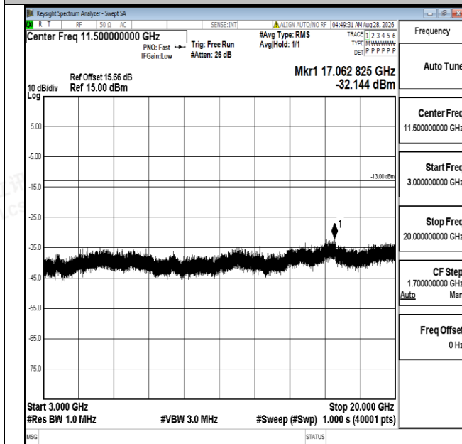
Band25-5MHz-QPSK-26065-1RB#0-3000~20000-PASS
