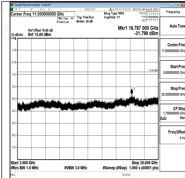
Band25-10MHz-QPSK-26640-1RB#0-3000~20000-PASS
