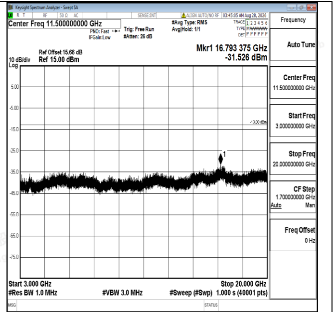
Band25-3MHz-16QAM-26675-1RB#0-3000~20000-PASS
