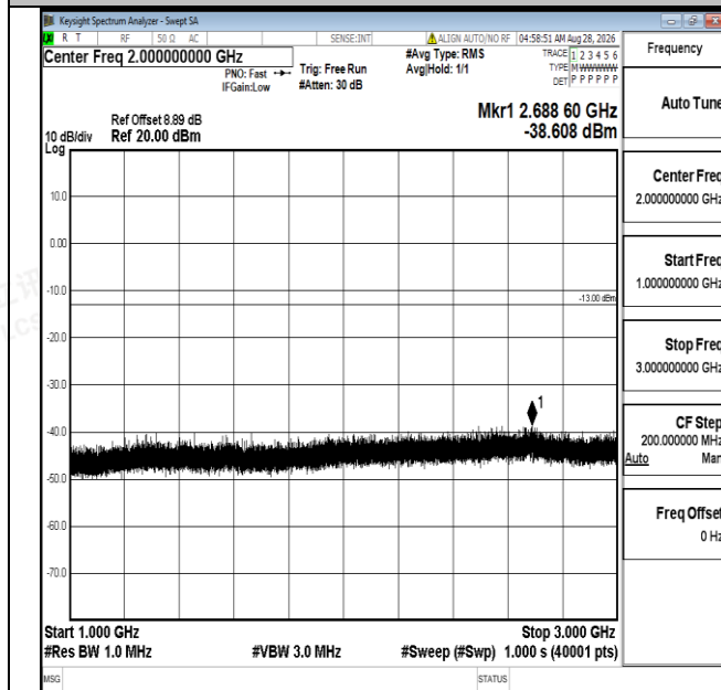
Band25-5MHz-16QAM-26665-1RB#0-1000~3000-PASS
