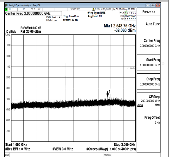
Band25-5MHz-QPSK-26365-1RB#0-1000~3000-PASS
