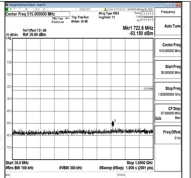
Band25-5MHz-16QAM-26065-1RB#0-30~1000-PASS
