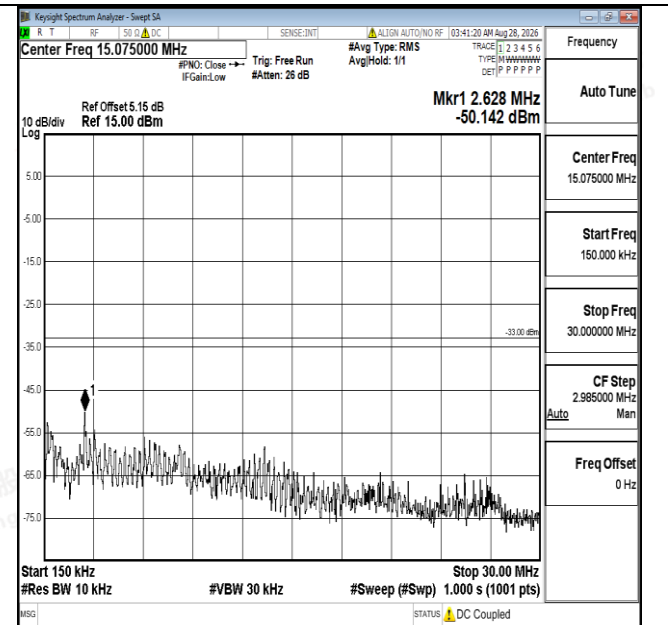
Band25-3MHz-QPSK-26675-1RB#0-0.15~30-PASS
