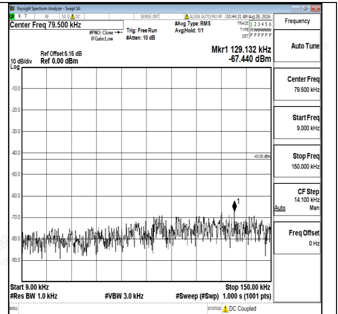
Band25-3MHz-16QAM-26675-1RB#0-0.009~0.15-PASS
