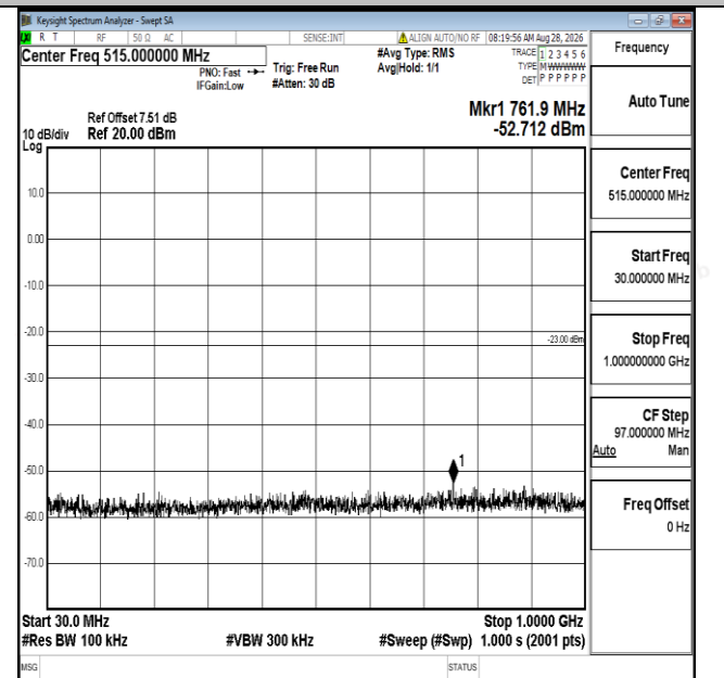
Band25-10MHz-16QAM-26090-1RB#0-30~1000-PASS
