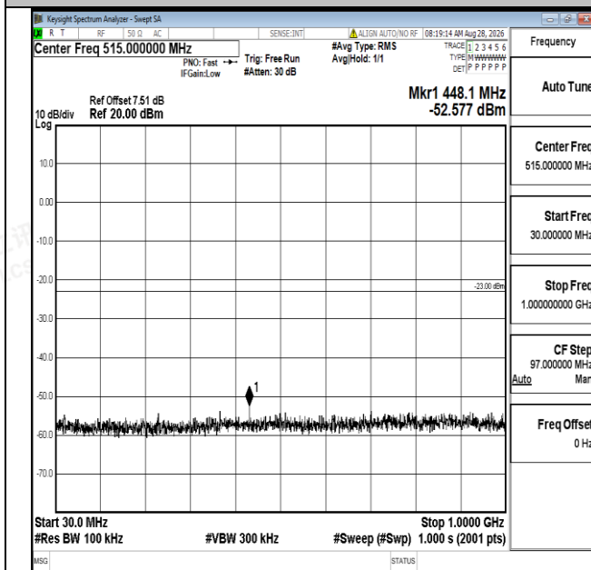
Band25-10MHz-QPSK-26090-1RB#0-30~1000-PASS
