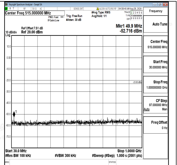
Band25-5MHz-16QAM-26665-1RB#0-30~1000-PASS
