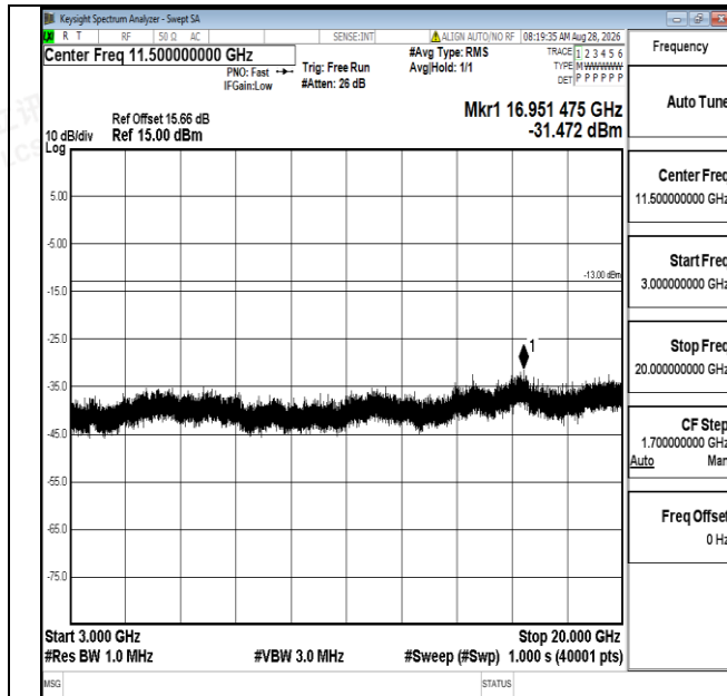
Band25-10MHz-QPSK-26090-1RB#0-3000~20000-PASS
