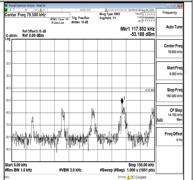
Band25-5MHz-16QAM-26065-1RB#0-0.009~0.15-PASS
