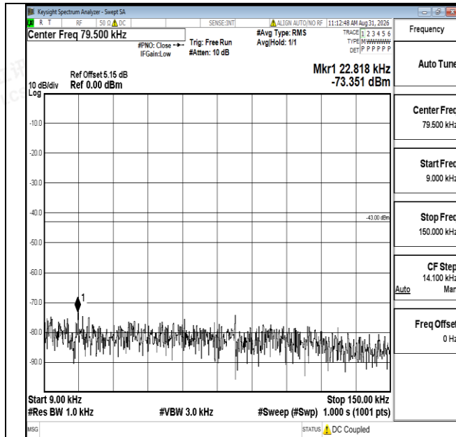
Band25-15MHz-QPSK-26365-1RB#0-0.009~0.15-PASS
