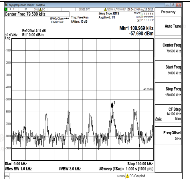
Band25-10MHz-16QAM-26640-1RB#0-0.009~0.15-PASS
