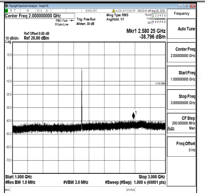
Band25-10MHz-QPSK-26640-1RB#0-1000~3000-PASS
