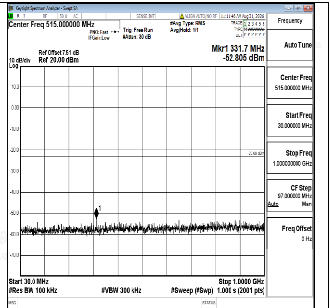
Band25-15MHz-16QAM-26115-1RB#0-30~1000-PASS
