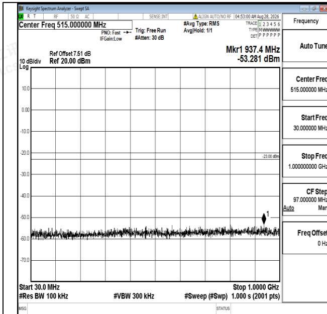
Band25-5MHz-QPSK-26665-1RB#0-30~1000-PASS
