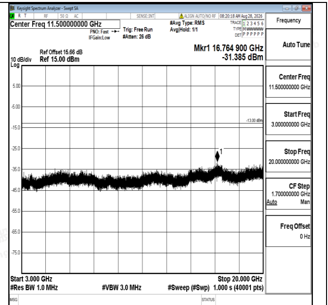
Band25-10MHz-16QAM-26090-1RB#0-3000~20000-PASS
