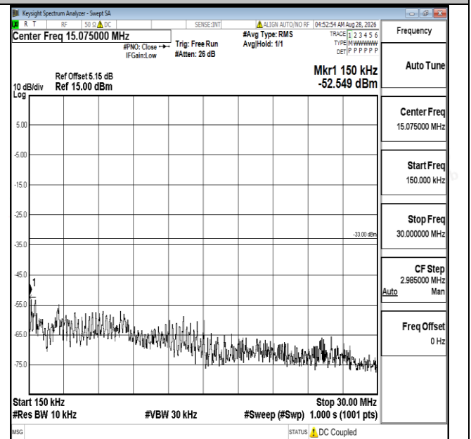
Band25-5MHz-QPSK-26665-1RB#0-0.15~30-PASS
