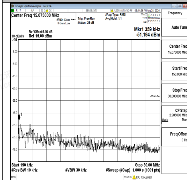
Band25-3MHz-16QAM-26675-1RB#0-0.15~30-PASS
