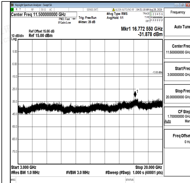
Band25-5MHz-QPSK-26365-1RB#0-3000~20000-PASS
