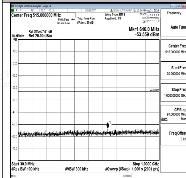
Band25-15MHz-QPSK-26365-1RB#0-30~1000-PASS
