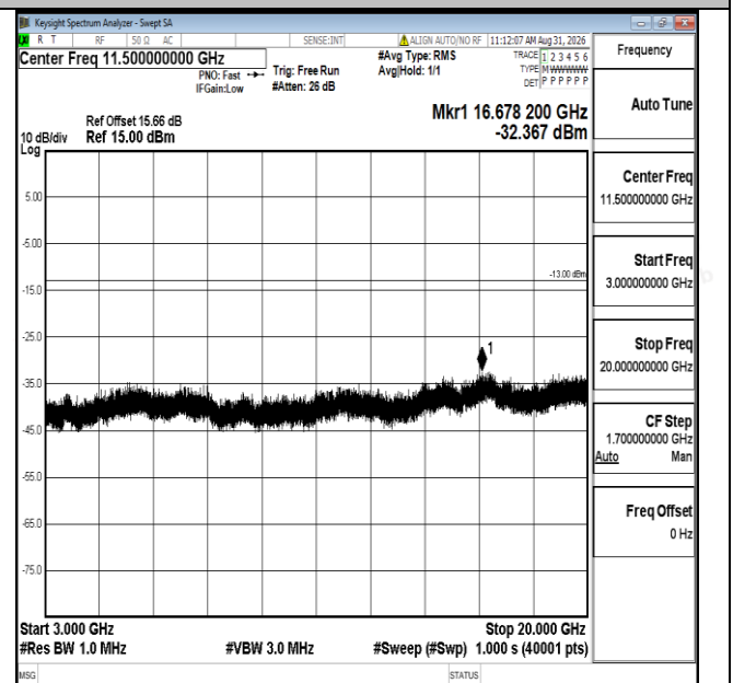
Band25-15MHz-16QAM-26115-1RB#0-3000~20000-PASS
