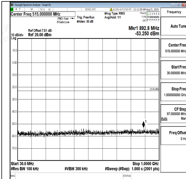
Band25-15MHz-QPSK-26115-1RB#0-30~1000-PASS
