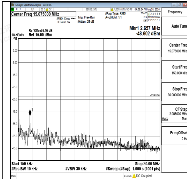
Band25-5MHz-16QAM-26665-1RB#0-0.15~30-PASS
