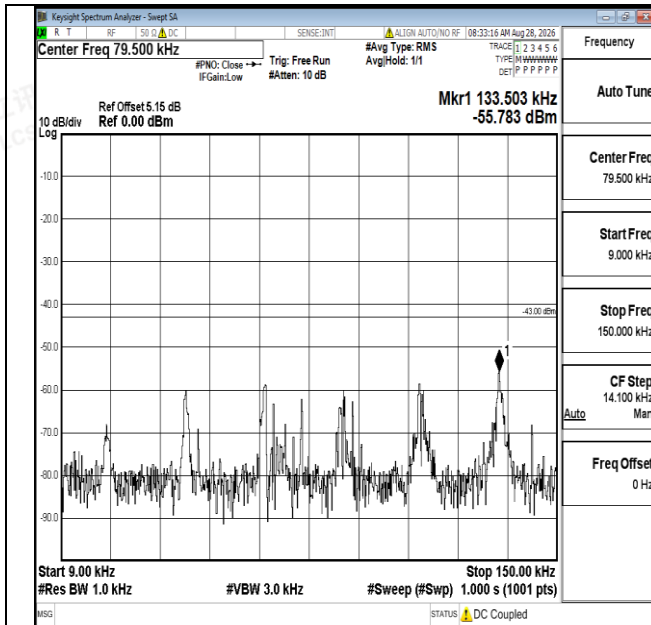
Band25-10MHz-QPSK-26640-1RB#0-0.009~0.15-PASS
