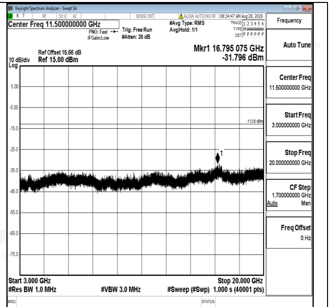
Band25-10MHz-16QAM-26640-1RB#0-3000-20000-PASS
