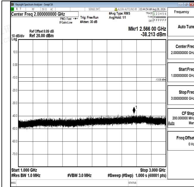
Band25-3MHz-16QAM-26675-1RB#0-1000~3000-PASS
