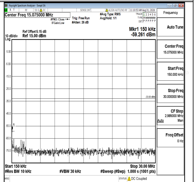
Band25-15MHz-QPSK-26115-1RB#0-0.15-30-PASS
