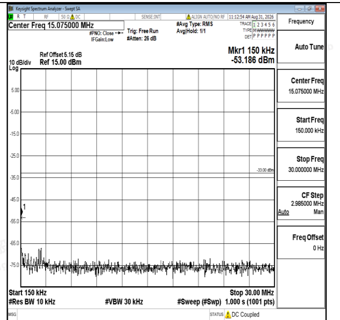
Band25-15MHz-QPSK-26365-1RB#0-0.15~30-PASS
