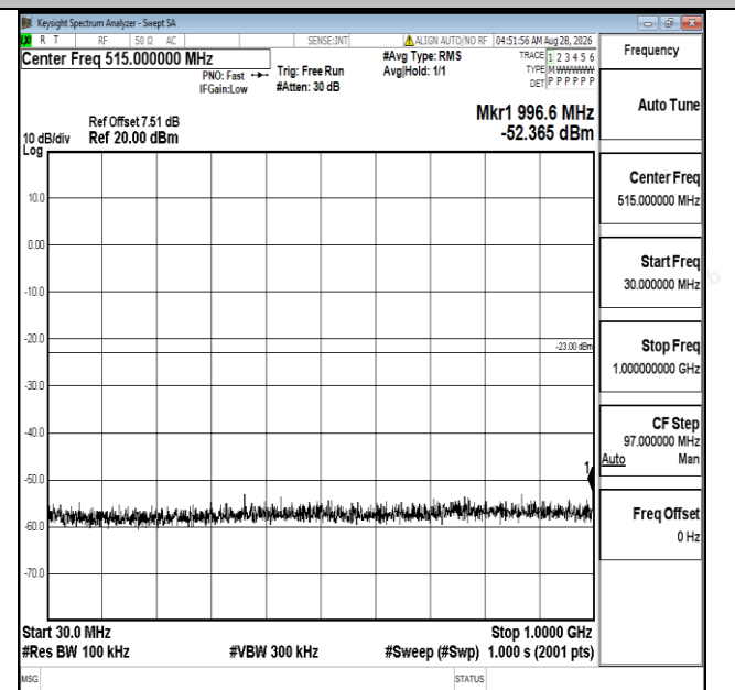
Band25-5MHz-16QAM-26365-1RB#0-30~1000-PASS
