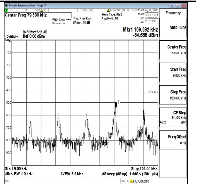
Band25-10MHz-16QAM-26365-1RB#0-0.009~0.15-PASS
