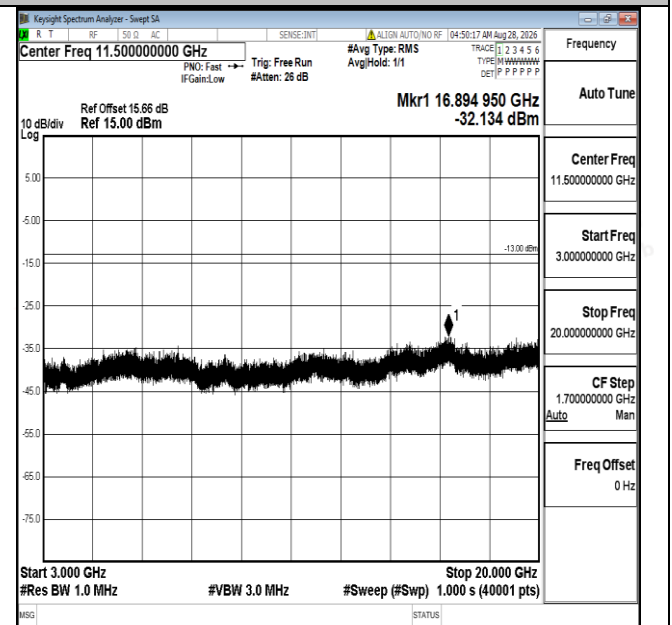
Band25-5MHz-16QAM-26065-1RB#0-3000~20000-PASS
