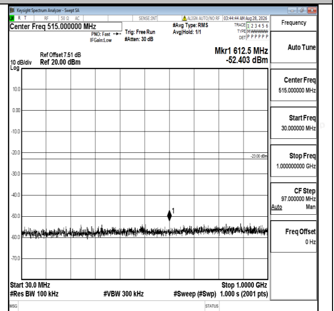
Band25-3MHz-16QAM-26675-1RB#0-30~1000-PASS
