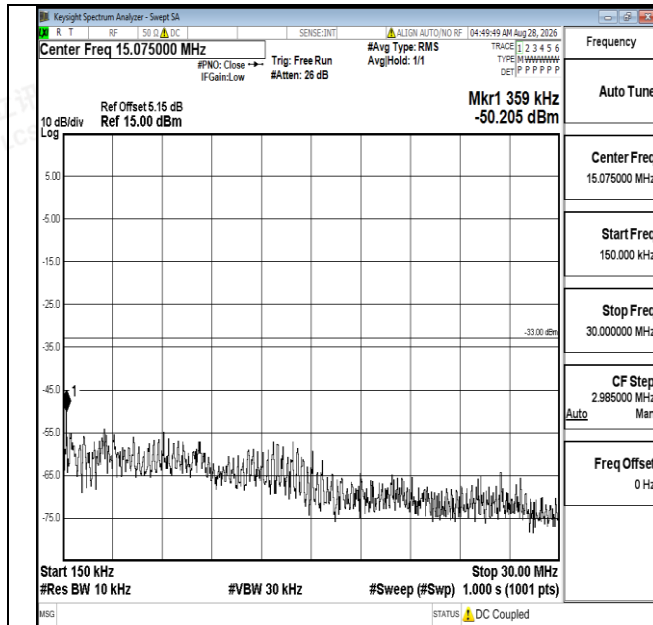
Band25-5MHz-16QAM-26065-1RB#0-0.15~30-PASS
