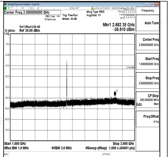
Band25-5MHz-QPSK-26665-1RB#0-1000~3000-PASS
