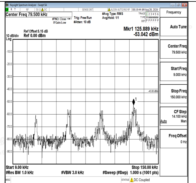
Band25-10MHz-16QAM-26090-1RB#0-0.009~0.15-PASS
