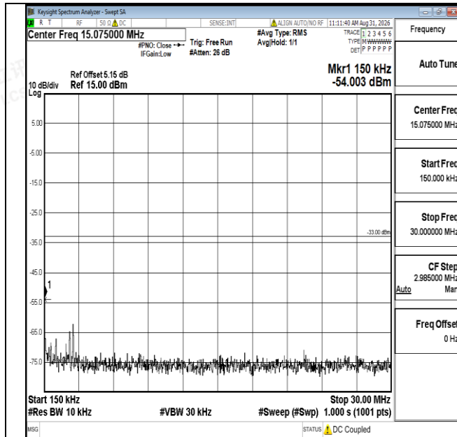
Band25-15MHz-16QAM-26115-1RB#0-0.15~30-PASS
