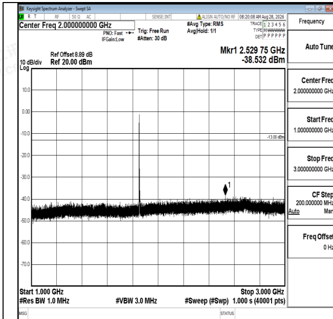
Band25-10MHz-16QAM-26090-1RB#0-1000~3000-PASS
