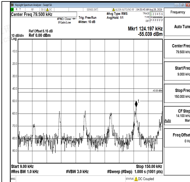
Band25-5MHz-QPSK-26365-1RB#0-0.009~0.15-PASS
