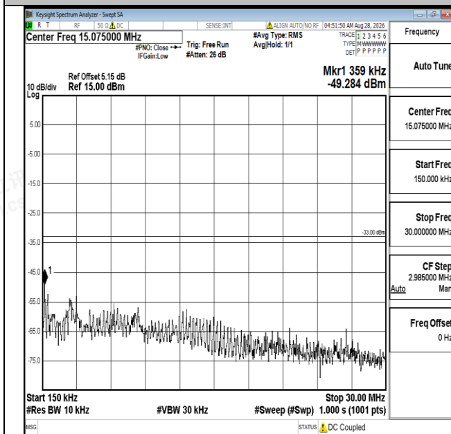
Band25-5MHz-16QAM-26365-1RB#0-0.15~30-PASS
