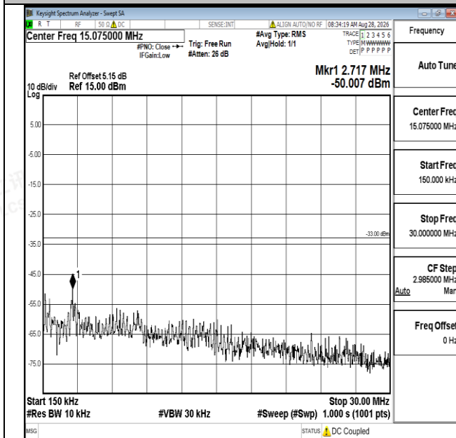
Band25-10MHz-16QAM-26640-1RB#0-0.15~30-PASS
