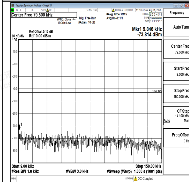
Band25-15MHz-QPSK-26115-1RB#0-0.009-0.15-PASS
