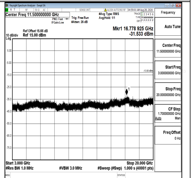
Band25-5MHz-16QAM-26665-1RB#0-3000~20000-PASS
