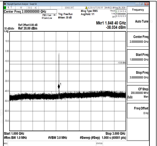
Band25-5MHz-QPSK-26065-1RB#0-1000~3000-PASS
