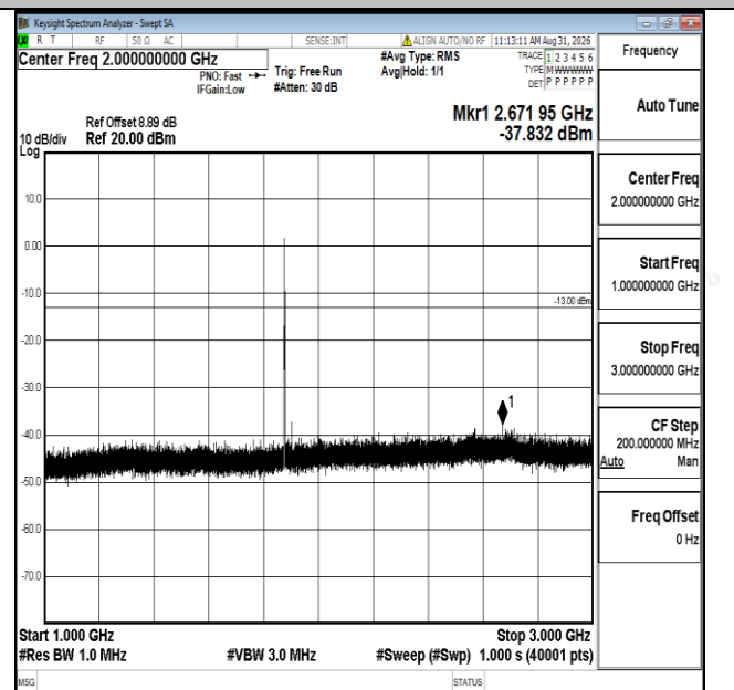
Band25-15MHz-QPSK-26365-1RB#0-1000~3000-PASS
