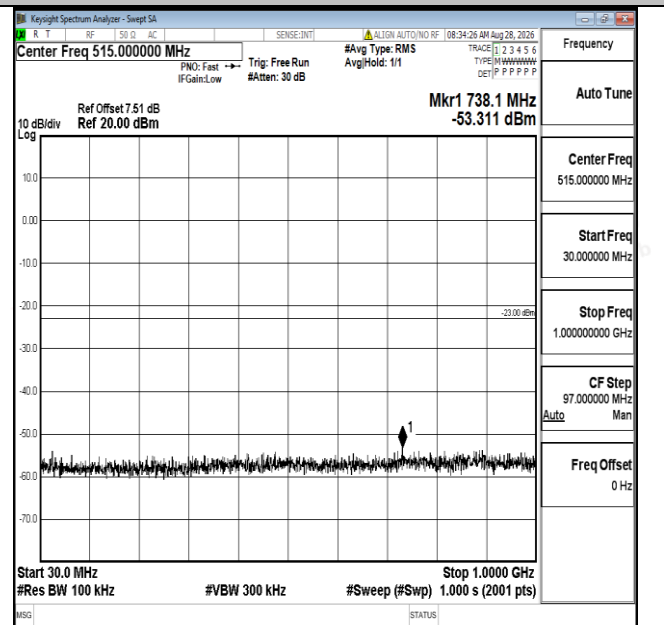
Band25-10MHz-16QAM-26640-1RB#0-30~1000-PASS
