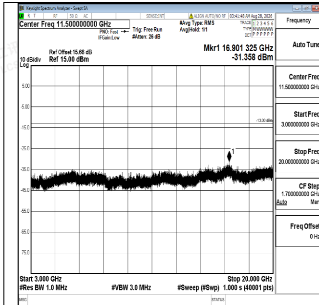
Band25-3MHz-QPSK-26675-1RB#0-3000~20000-PASS
