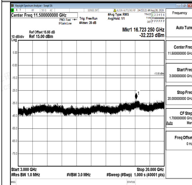
Band25-5MHz-QPSK-26665-1RB#0-3000~20000-PASS
