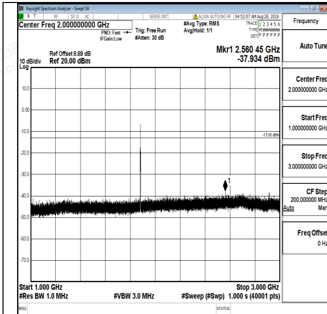
Band25-5MHz-16QAM-26365-1RB#0-1000~3000-PASS
