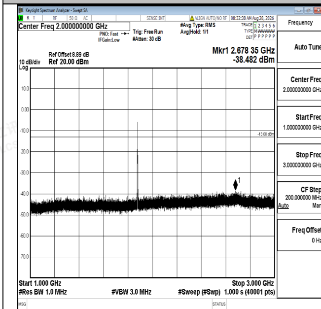
Band25-10MHz-16QAM-26365-1RB#0-1000~3000-PASS
