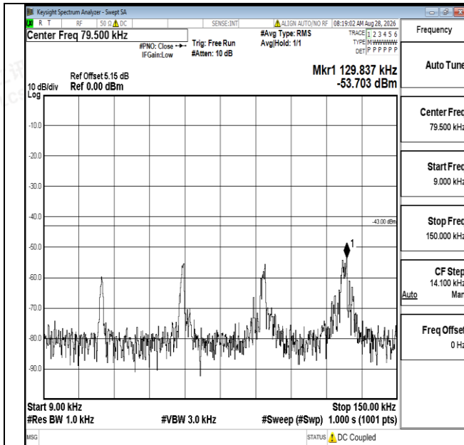
Band25-10MHz-QPSK-26090-1RB#0-0.009~0.15-PASS
