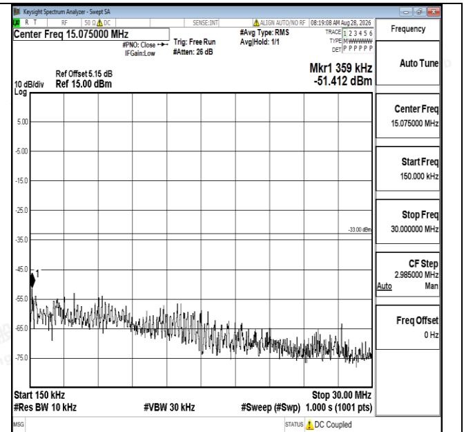
Band25-10MHz-QPSK-26090-1RB#0-0.15~30-PASS
