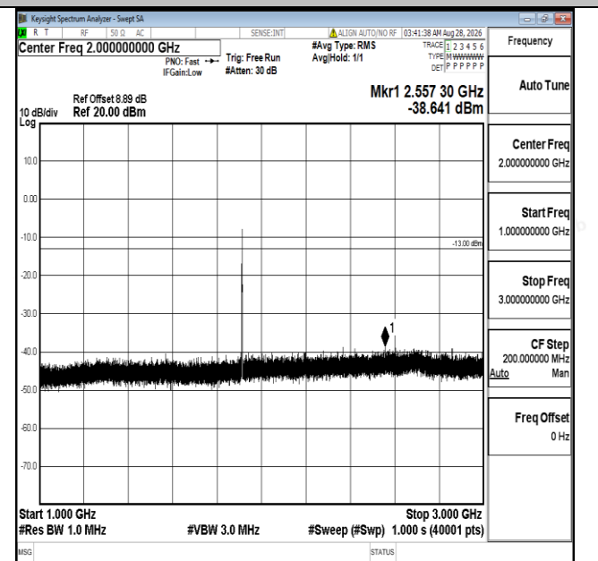
Band25-3MHz-QPSK-26675-1RB#0-1000~3000-PASS
