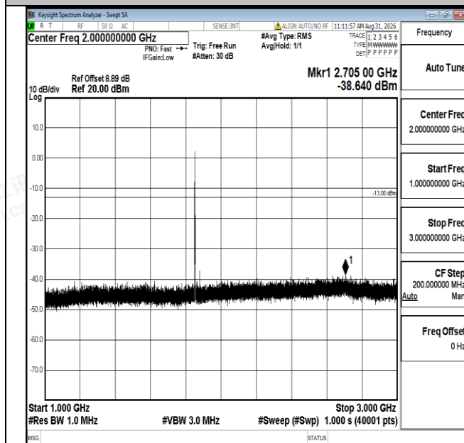
Band25-15MHz-16QAM-26115-1RB#0-1000~3000-PASS
