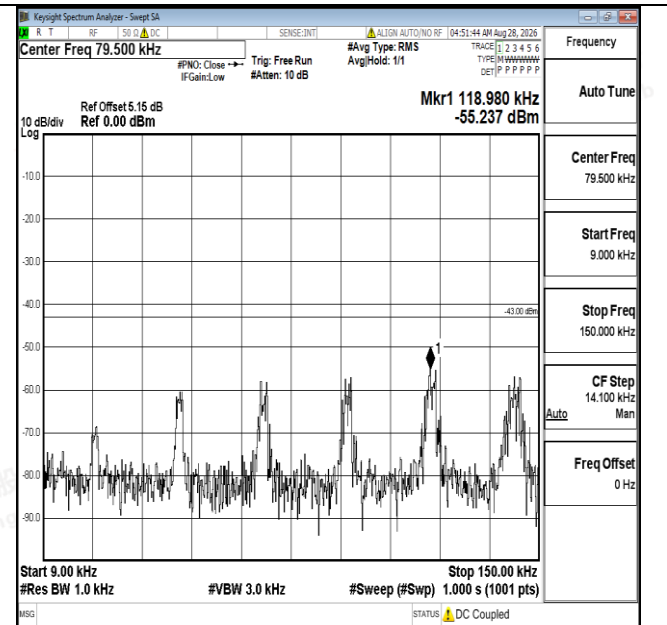
Band25-5MHz-16QAM-26365-1RB#0-0.009~0.15-PASS
