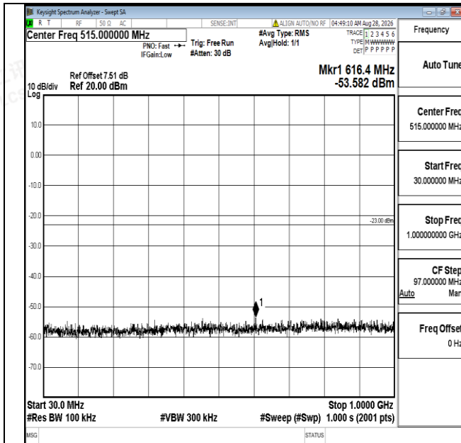
Band25-5MHz-QPSK-26065-1RB#0-30~1000-PASS
